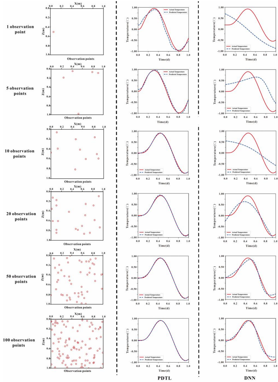
Figure 6. Comparisons of the predicted temperature (blue curves) and reference temperature (red curves) using PDLT and DNN models for homogeneous streambed.
