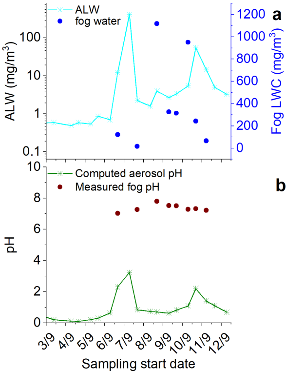
355 Figure 2. Timeseries of (a) aerosol liquid water content (ALW) calculated with E-AIM and measured fog liquid water content (LWC) retrieved from the measured water collected with the CASC sampler and, (b) pH in aerosol calculated with E-AIM and measured pH in fog. Fog samples H1001 and H1002 have been averaged over the TSP sample S-34 collection time. TSP samples reported here are those corresponding to sample IDs S20 to S38.
