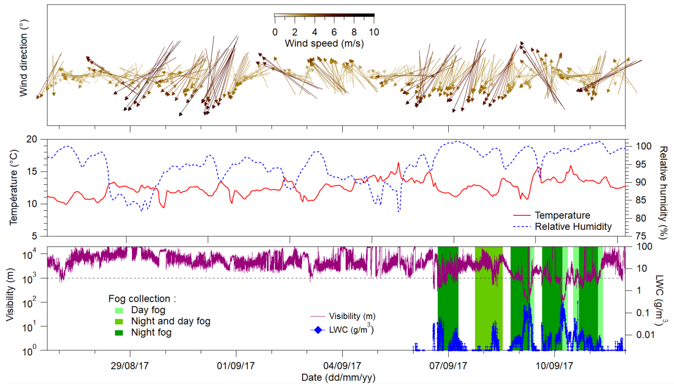
Figure 1. Timeseries of wind direction and speed (top panel); hourly average relative humidity RH%, and temperature T (middle panel); visibility and liquid water content (LWC) of the fog (bottom panel). The green shades on the bottom panel correspond to the fog collection periods. Fog events are generally classified as visibility < 1 km.
