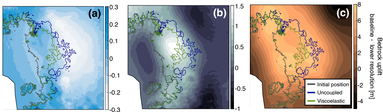
Figure A6. Loss in bedrock uplift due to setting the maximum Love number degree in the PLUS setup to (a) 512 (39 km), (b) 180 (111 km), and (c) 90 (222 km), instead of the reference value of 40,000-000 (1 km). Grounding line positions at year 2350 for the Viscoelastic viscoelastic (green) and Uncoupled-uncoupled (blue) runs are overlaid for reference. The initial grounding line position is reported in gray. Note that the colorbar scales vary between panels.
