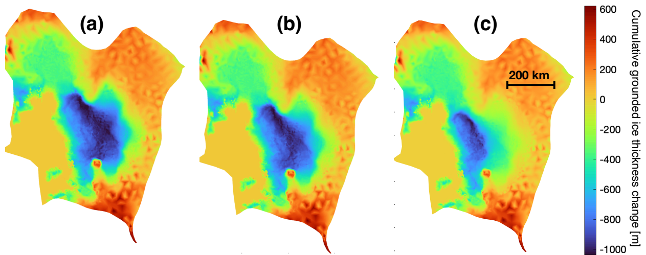
Figure A7. Cumulative grounded ice thickness change through 2350 in the (a) Uncoupled uncoupled , (b) Elastic elastic , and (c) Viscoelastic viscoelastic runs of the PLUS setup.
