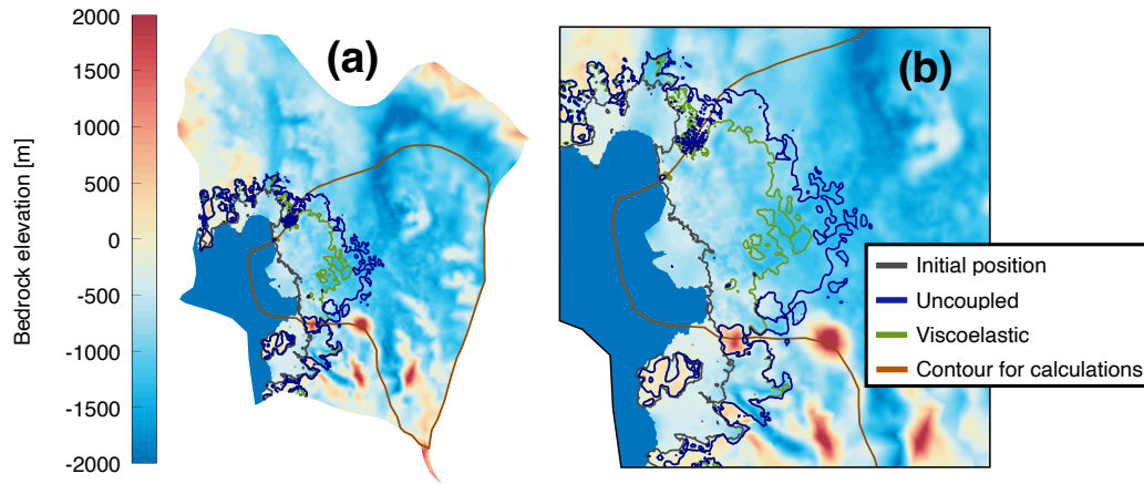
Figure A4. Contour of the region over which GMSL contribution and ungrounded ice area are calculated throughout the paper (brown). Viscoelastic (green) and Uncoupled uncoupled (blue) grounding line projections in 2350 for the PLUS setup are overlaid for reference. Initial grounding line position is reported in gray. (a) Represents the region of the Amundsen-Sea sector ASE under study and (b) corresponds to the region depicted in Figs. 1 and 2.
