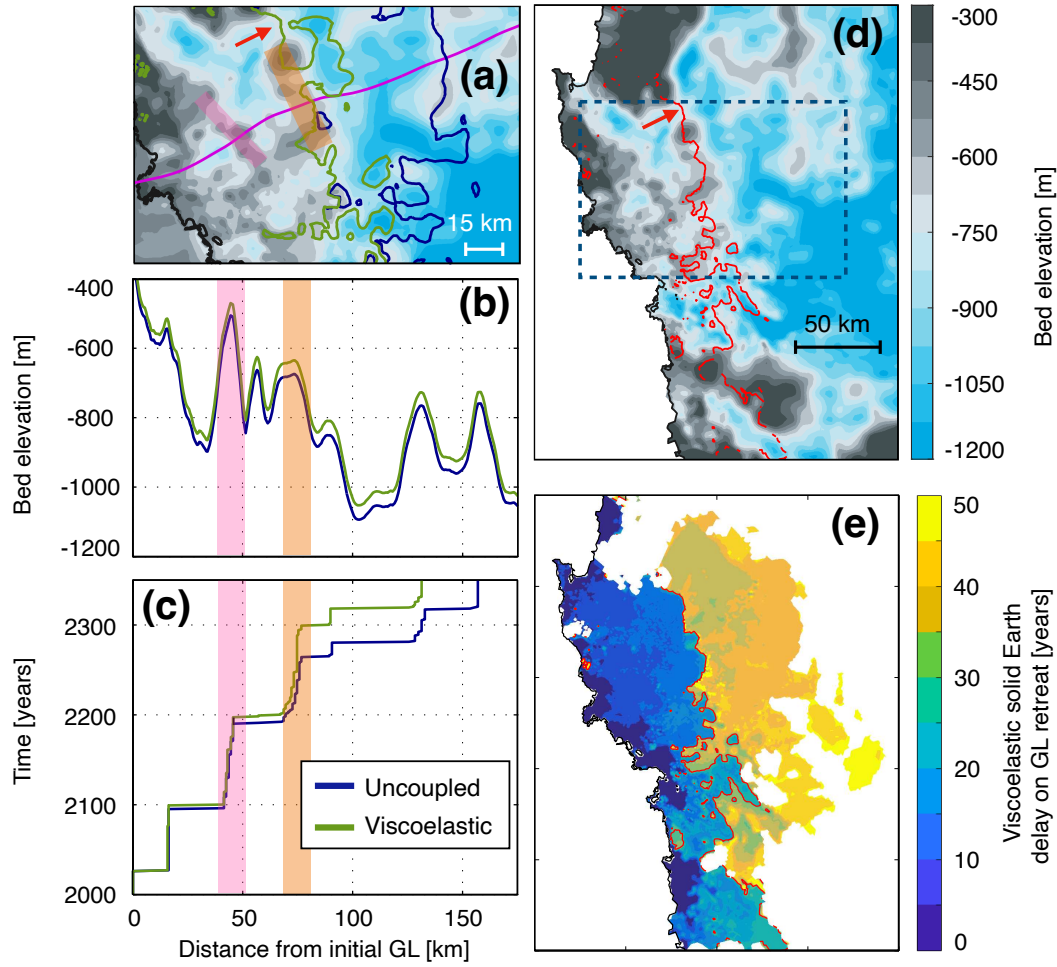
Figure 4. (a) Grounding Line (GL) positions at year 2292 for the Viscoelastic-viscoelastic (green) and Uncoupled-uncoupled (blue) runs of the PLUS setup overlaid on the initial bedrock. Initial GL is represented in black. (b) Topography along the magenta flowline. The green line includes viscoelastic uplift at year 2292. (c) GL migration (x-axis) through time (y-axis). The x-axis is shared with (b). Circles-The pink and orange shadings indicate the locations of 2 key bedrock ridges which pin the GL for extended time periods. (d) Initial bedrock in , the Viscoelastic-run's GL retreat area . The blue dotted box corresponds to the area depicted in (a). (e) Delay in GL delay-induced-by-retreat due to GRD effects . The red line identifies the 25 year delay isocontour which coincides with the 2nd-second ridge of the basin and marks a sharp increase in the delay.
