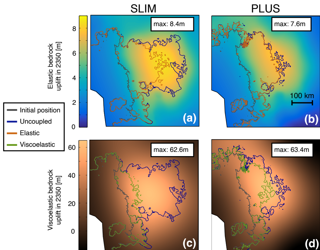
Figure 2. Bedrock uplifts at year 2350 for the SLIM (a and c) and PLUS (b and d) setups. The grounding line positions for the Viscoelastic viscoelastic (green), Elastic-elastic (brown) and Uncoupled-uncoupled (blue) runs are overlaid on top of the Elastic-elastic (a and b) and Viscoelastic-viscoelastic (c and d) bedrock uplifts. The initial grounding line position is represented in gray.
