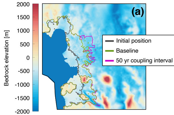
Figure A5. Grounding line projections in the SLIM setup at year 2350. The projection for the baseline Viscoelastic viscoelastic run (green) is shown alongside the projection for the 50 year coupling interval run (magenta). The initial grounding line position is reported in gray.
