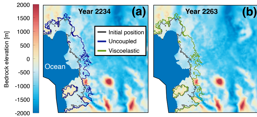
Figure A3. Grounding line projections in the Amundsen-Sea sector ASE in the SLIM-PLUS setup. (a) Projection for the year 2234 in the Uncoupled uncoupled run (blue). (b) Projection at year 2263 in the Viscoelastic viscoelastic run (green). Initial grounding line position is reported in gray.
