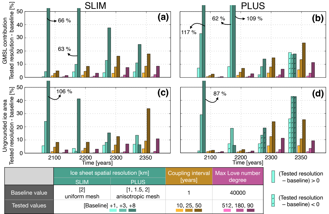
Figure 5. Sensitivity to (i) ice sheet spatial resolution, (ii) maximum Love number degree and (iii) coupling interval, for the SLIM (a and c) and PLUS (b and d) setups. Differences For each tested resolution, differences to the baseline in GMSL contribution are represented in the top row, and differences in ungrounded ice area are shown in the bottom row. Results are provided for four years (2100, 2200, 2300, 2350). For each parameter, three values are explored, with lighter colors indicating finer resolutions. For the ice sheet spatial resolution, the SLIM baseline uses a uniform 2 km mesh, while the PLUS baseline uses an anisotropic mesh refined to 1, 1.5 and 2 km in the region of grounding line retreat.
