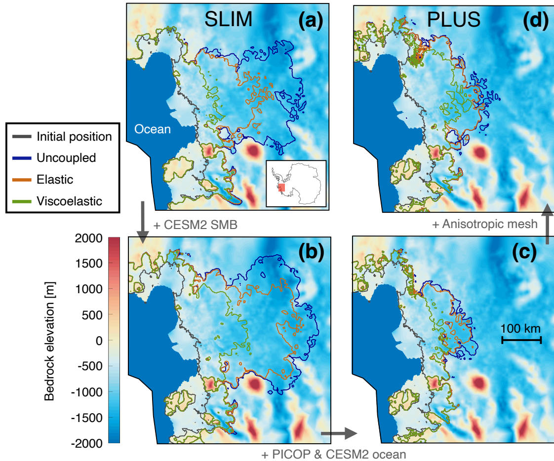
Figure 1. Grounding line projection in the Amundsen Sea sector (ASE) at year 2350 for the SLIM (a) and PLUS (d) setups. Projections for intermediate setups are shown to illustrate the effects of incorporating CESM2 SMB forcings (b), PICOP with CESM2 ocean forcings (c), and an anisotropic mesh. The grounding line positions for the Viscoelastic-viscoelastic (green), Elastic-elastic (brown) and Uncoupled uncoupled (blue) runs are overlaid on top of the bedrock topography. The initial grounding line position is represented in gray and the ice-free ocean is depicted in solid blue. The location of the basin in Antarctica is shown in the bottom right inset of (a).
