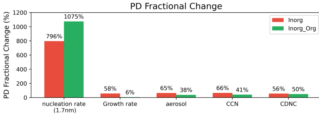
280 Figure 7. Figure 6. The global mean of the PD fractional change ((PD-PI)/PI) of key variables. Model experiments are described in Table 2 and model data come from monthly mean value over 10 years.
