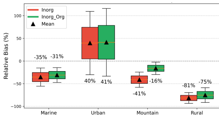
195 Figure 1. Box plots showing the relative bias (%) between simulated monthly mean and observed median CCN number concentrations across categorized background sites (Marine, Urban, Mountain, Rural). Red and green boxes represent the Inorg and Inorg_Org experiments, respectively. Black triangles indicate the mean relative bias for each category. Numerical values above the boxes denote the corresponding mean normalized mean bias (NMB) for each experiment. Information on the measurement sites is provided in Table 2.
