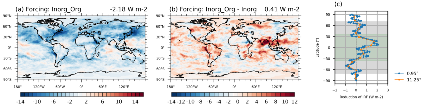
275 Figure 6 Figure 5. The effective radiative forcing due to aerosol–cloud interactions ( ERF_{aci} ) aerosol after including organic NPF (a) and the difference in the ERF_{aci} of anthropogenic aerosol between with and without organic NPF (b). The zonal mean of the information in (b) is shown in (c) (Blue scatters show the zonal mean with an interval of 0.95^\circ and the orange scatters show the zonal mean with an interval of 11.25^\circ ). The global average value is shown on the top right of each panel. Model experiments are described in Table 2 and model data come from monthly mean value over 10 years.
