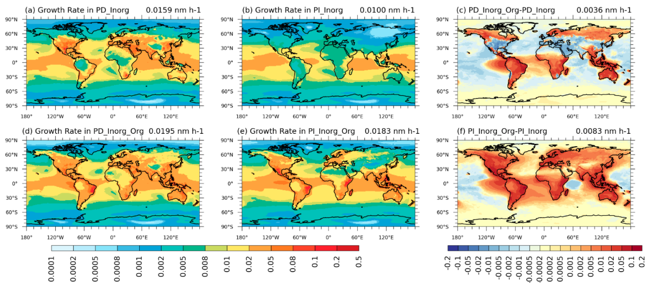
335 Figure 8. Spatial distribution of the simulated vertically-mean growth rate in (a and d) PD and (b and e) PI experiments. The difference between Inorg\_Org and Inorg in PD and PI experiments is shown in (c) and (f) (unit: \text{nm h}^{-1} ). Global mean values are shown on the top right of each figure.
