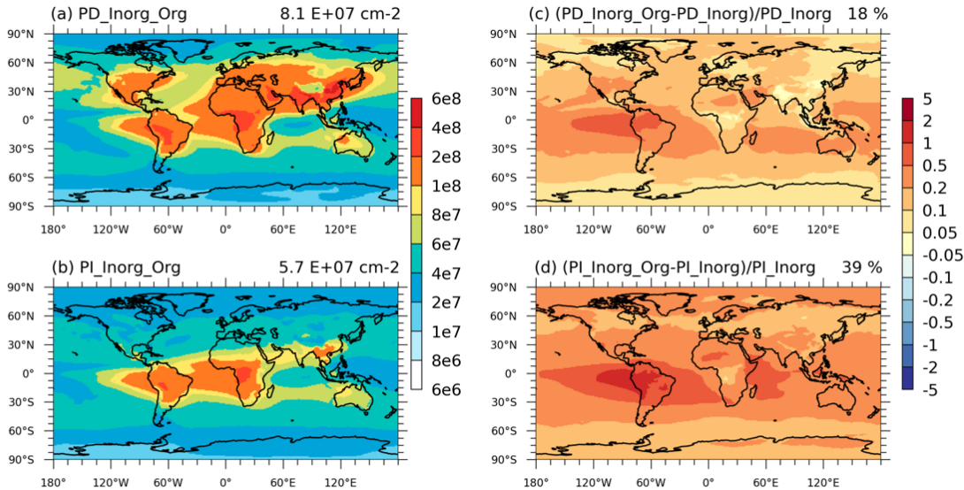
Figure 2. Spatial distribution of the simulated vertically-integrated CCN at 0.2% supersaturation (ss) in (a) PD_Inorg_Org and (b) PI_Inorg_Org (unit: \text{cm}^{-2} ). The relative change after adding organic NPF in PD and PI environments are shown in (c) and (d). Global mean values are shown on the top right of each figure.
