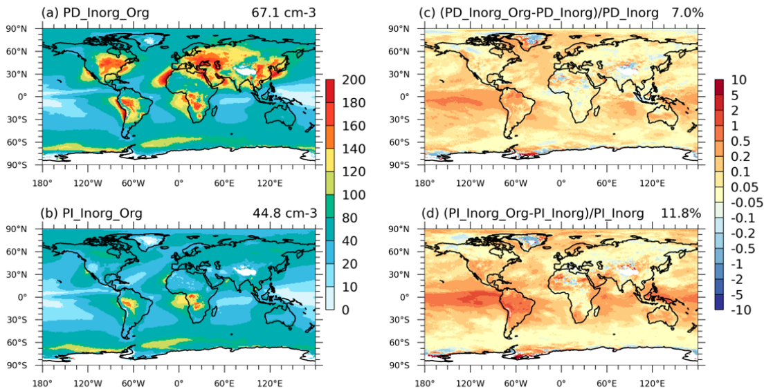
Figure 3. Spatial distribution of the simulated cloud droplet number concentration (CDNC) at the top of low clouds in (a) PD_Inorg_Org and (b) PI_Inorg_Org (unit: \text{cm}^{-3} ). The relative change after adding organic NPF in PD and PI environments are shown in (c) and (d). Global mean values are shown on the top right of each figure.
