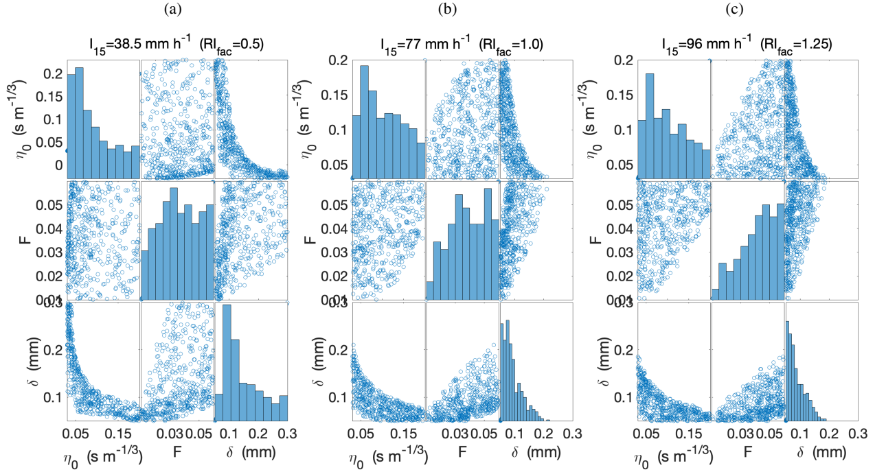
Figure 4. (a) I_{15} = 38.5 \text{ mm h}^{-1} ( RI_{fac} = 0.5 ); (b): I_{15} = 77 \text{ mm h}^{-1} ( RI_{fac} = 1 ); (c): I_{15} = 96 \text{ mm h}^{-1} ( RI_{fac} = 1.25 ). Each panel contains histograms and pairwise scatter plots of \eta_0 , F , and \delta that result in GP volume predictions \pm 10\% of the targeted volumes. The target volume for a given I_{15} is defined as that predicted by the Gartner et al. Emergency Assessment Volume model (Gartner et al., 2014). Note that the vertical and horizontal labels apply to each scatter plot in the matrix, but only the horizontal labels apply to the histograms.
