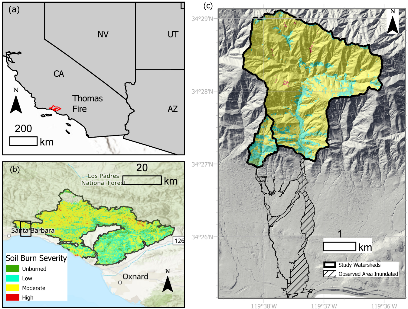
Figure 1. (a) The Thomas Fire ignited on 4 December 2017 and burned over 1140 km 2 in southern California, USA. (b) The western portion of the burned area included a series of steep watersheds (black rectangle) above the community of Montecito, located near Santa Barbara. (c) Our study focuses on two watersheds, Oak Creek (0.45 km 2 ) and San Ysidro Creek (7.6 km 2 ), located upstream of Montecito. The KTYD gauge is located approximately 5 km west of the watershed centroid.
