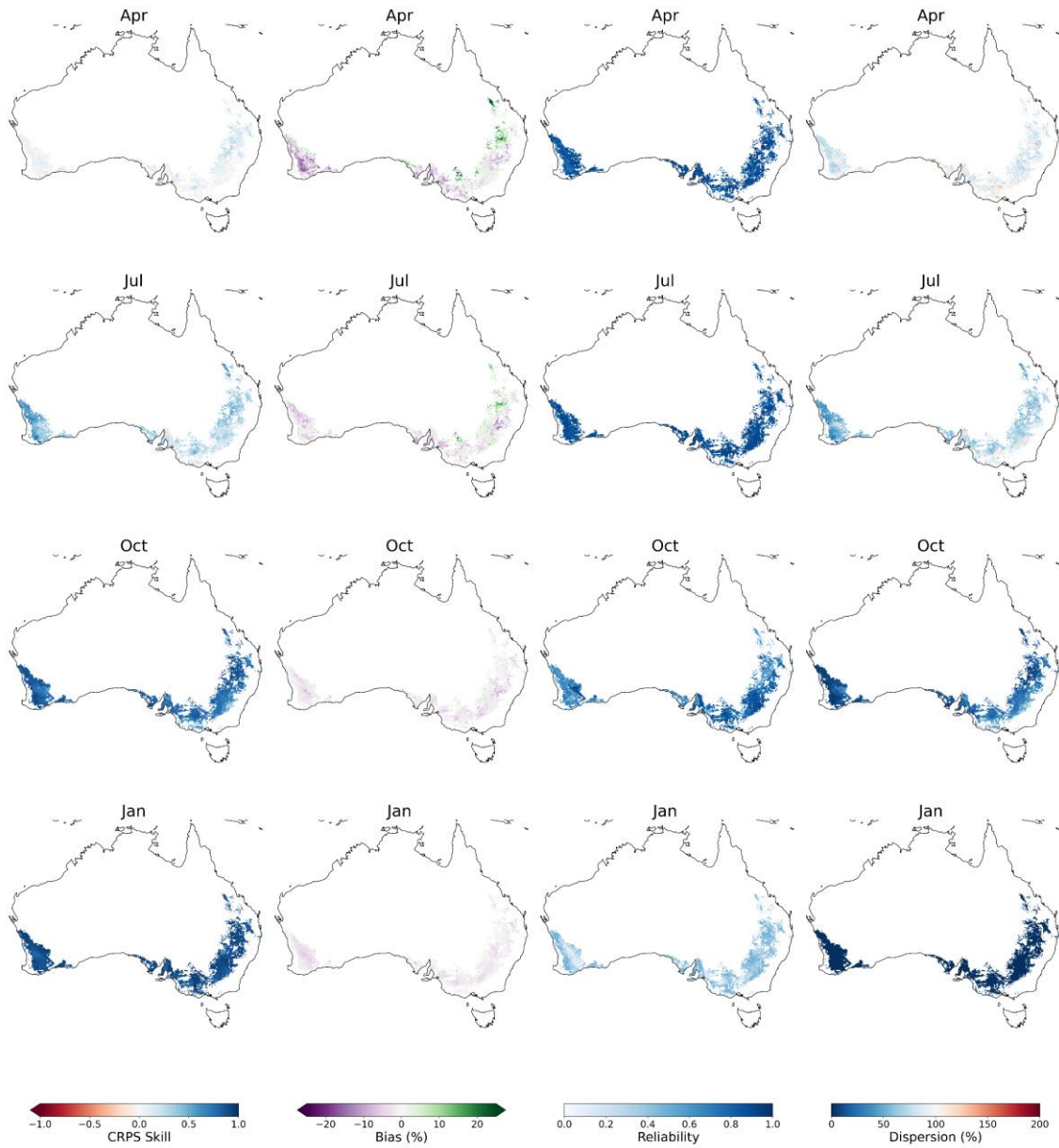
290 Figure 5: Forecast verification maps for the APSIM potential wheat yield indicator calculated over the period 1990-2018. Columns are per verification metric: CRPS Skill Score, bias, reliability and dispersion. Rows are per forecast issue date: April in the previous financial year, then July, October and January of the current financial year.
