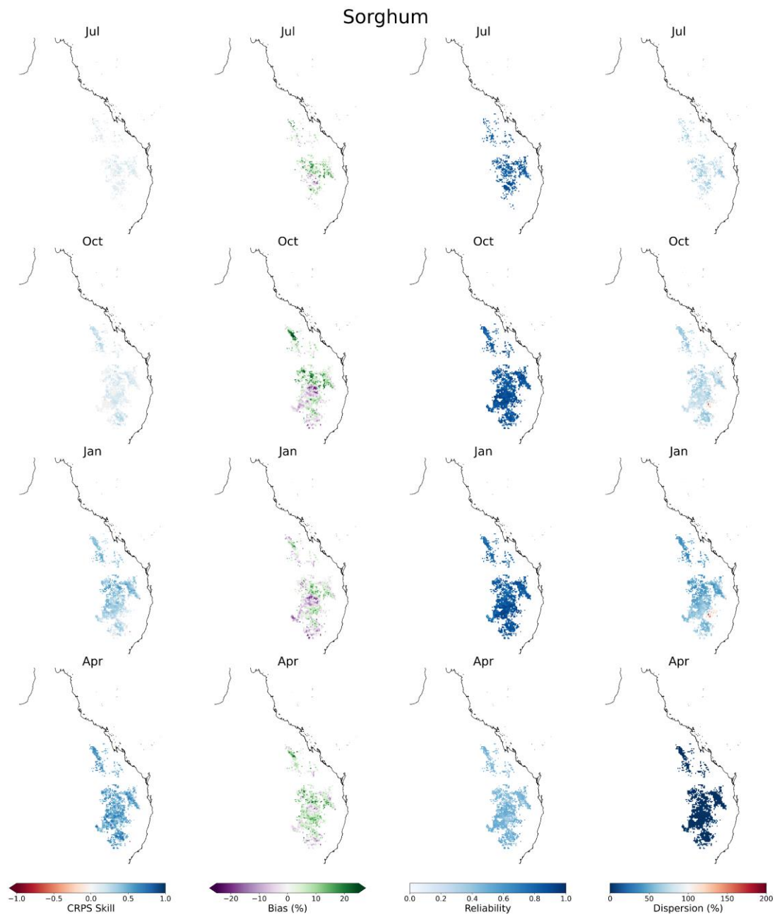
295 Figure 6: Forecast verification maps for the APSIM potential sorghum yield indicator calculated over the period 1990-2018. Columns are per verification metric: CRPS Skill Score, bias, reliability and dispersion. Rows are per forecast issue date: July, October, January and April of the current financial year.
