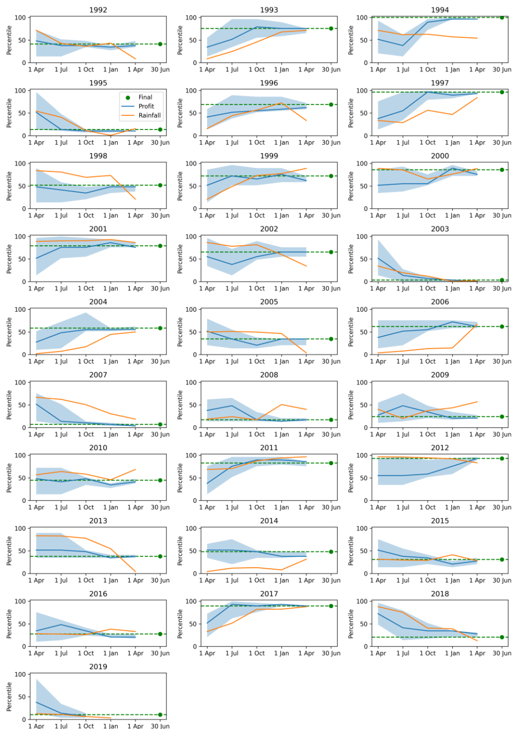
385 Figure 8: Time series plots of the nationally averaged farm profit indicator within agricultural zones (blue line) with the blue shading depicting the interdecile range of the ensemble. The x-axis depicts the forecast issue date and the y-axis is the percentile. The final farm profit for the financial year is plotted (green line) as well as the nationally averaged 12-month lagged rainfall percentile (orange line).
