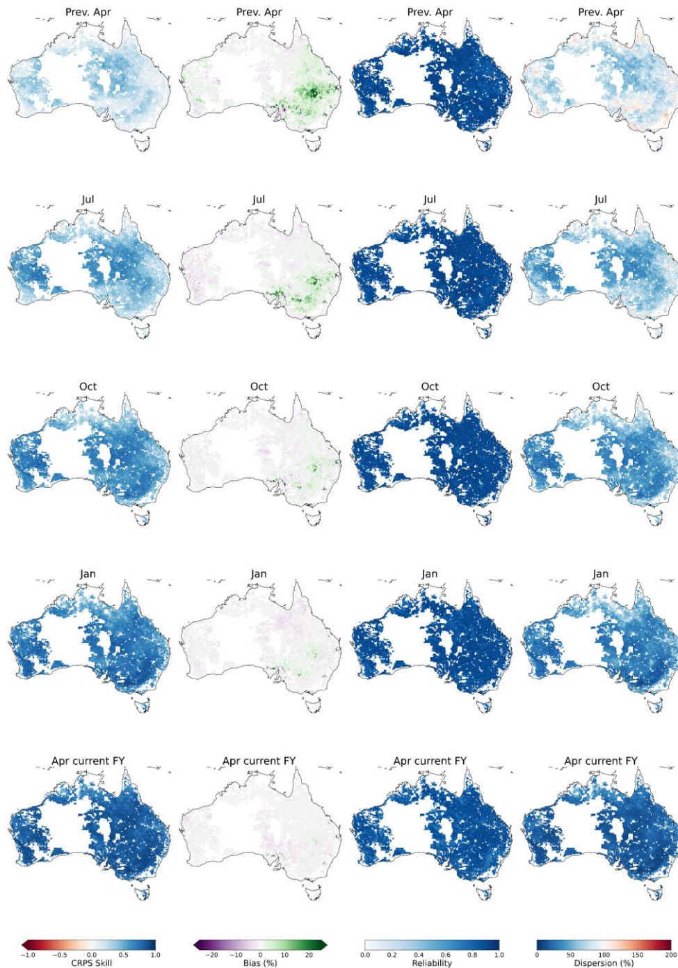
Figure 4: Forecast verification maps for the farm profit indicator calculated over the period 1990-2018. Columns are per verification metric: CRPS Skill Score, bias, reliability and dispersion. Rows are per forecast issue date: April in the previous financial year, then July, October, January and April of the current financial year.
