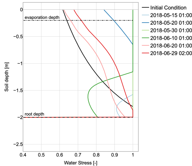
Figure 16. Evolution of water stress factor along the soil profile at various arbitrarily chosen times in the baseline simulation. This information can support more accurate and efficient irrigation scheduling based on soil water availability.
