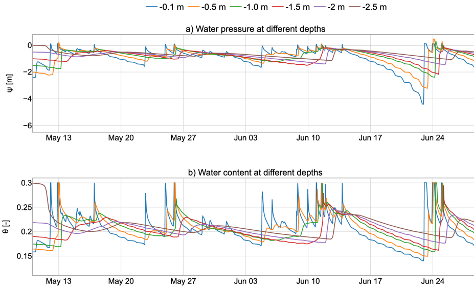
Figure 13. (a) Soil water potential, and (b) water content evolution with time at different depth in the baseline simulation. The data in these two figures are clearly related through the soil water retention curve. Notably, following certain rainfall events, soil saturation ( \psi > 0 ) is achieved a condition that cannot be adequately handled by solvers less sophisticated than those implemented in GEOSPACE.
