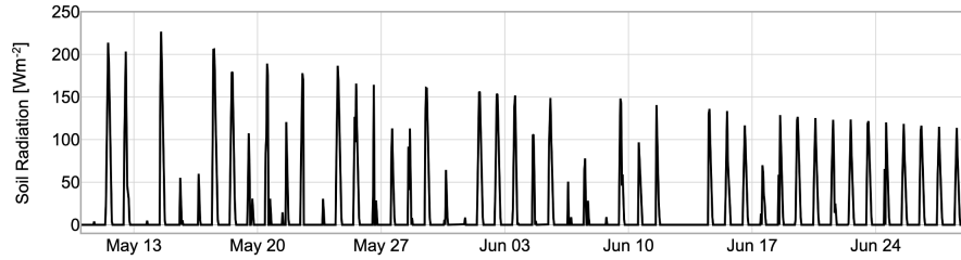
Figure 17. Radiation reaching the ground, given the prescribed LAI as input, in the baseline simulation. Decrease of radiation depends on meteorological conditions and the increase of LAI with time.
