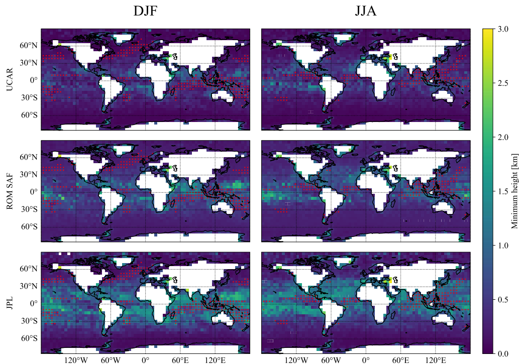
Figure A1. Maps of median minimum height on 5° bins for maritime occultations shared by all three processing centers for DJF (left) and JJA (right) 2008. Yellow coloring indicates more conservative (higher) minimum height. The minimum heights for all three centers are highest in the Tropics, especially for JPL, confirming the effects seen in Fig. 2. Bins with a seasonal mean precipitation of at least 5 mm d -1 on average are labeled with red stippling. No statistical mask is used in this figure so that fine, small-scale zonal and meridional patterns in minimum height are shown, but abnormally high or low minimum height values in individual cells — especially those along coastlines — may be due to larger noise.
