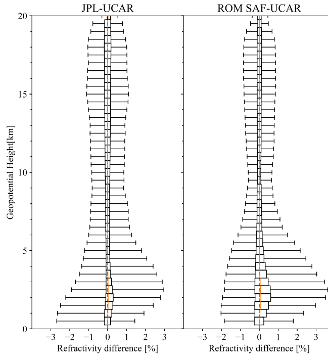
Figure 4. Box-and-whiskers plot showing the fractional refractivity differences between JPL and UCAR (left) and ROM SAF and UCAR (right) maritime occultations for winter (DJF) 2008. In order to compare across occultations, both traditional and penetration sampling bias are removed; this plot shows only structural biases between centers. Distributions are subset into 500 m geopotential height bins. Boxes show outline the central two quartiles of the distribution at each geopotential height while whiskers show the 1–99% ranges; orange lines show median at of each distribution. Gray dashed line indicates no refractivity difference.
