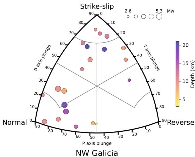
Fig. A15: NW Galicia tectonic zone. Top map: focal mechanisms with maximum horizontal axis (P or B for normal ruptures) and minimum horizontal axis (T or B for reverse ruptures) orientation. Bottom left classification diagram for earthquake rupture types. Middle right: Average tensors (complete in gray) and Kagan angles between the average tensors for each rupture type. Bottom right: Rose diagram of maximum and minimum horizontal axes orientation.
