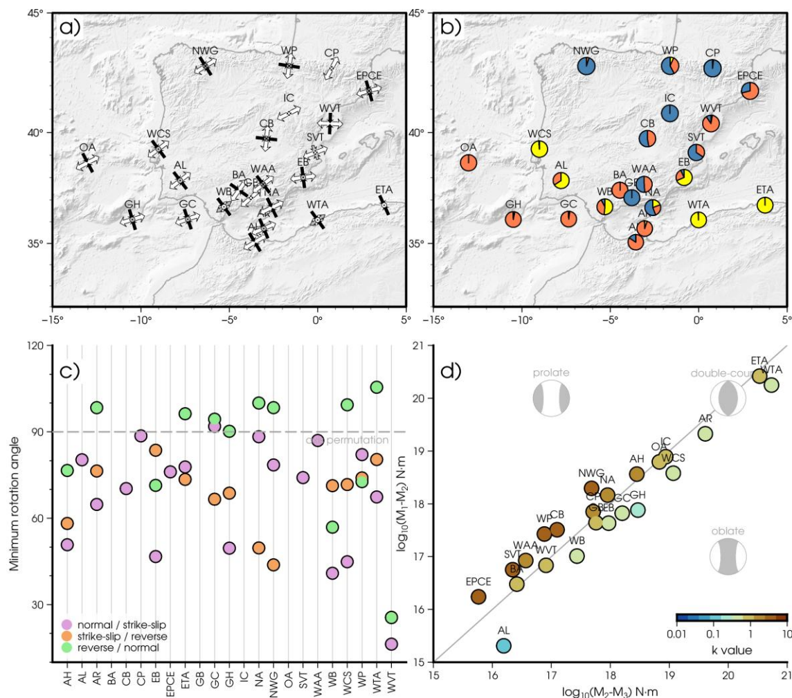
Figure 11: a) Strain principal directions derived from the combined moment tensors. Black shows the orientation of the shortening (P) axis; in white is shown the stretching axis (T) and grey the intermediate axis. The orientations are simplified showing only the trend of the principal axes and omitting the plunge. Note that the intermediate axis (in grey) can be a shortening or a stretching axis; when it is the vertical axis it is represented by a circle with a cross or with a dot respectively. b) Pie diagram showing the proportion of seismic moment released by strike-slip (red), reverse (yellow) and normal (blue) events on each zone. c) Representation of the minimum rotation angle (Kagan angle) between combined focal mechanisms for the different rupture types in each zone. A 90° angle represents a pure axes permutation. d) Flinn diagram adapted to the combined seismic strain tensor. Each circle represents the position on the diagram of each zone considered in the study. The color is proportional to the k value as is shown in the color scale. The gray tensors represent the seismic strain tensors for prolate, double-couple (plane strain) and oblate shape ellipsoids. The diagonal line represents the plane strain shapes, pure double couple in seismic tensor terminology. Note that the scales used for color and graph axes are logarithmic.
