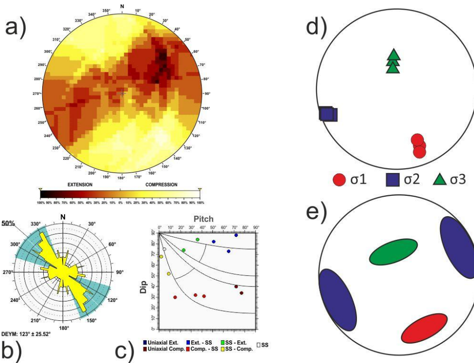
Fig. B12 Gorringle - Horseshoe tectonic zone. Results of the stress and strain analyses for different zones: a) Right Dihedra solution. b) Rose diagram of the Dey (horizontal shortening direction) obtained from the Slip model. c) Pitch/Dip plot for the neo-formed nodal planes obtained from the Slip Model. d) Stress Inversion Results. e) Variability of the three principal stress axes of the stress inversion.
