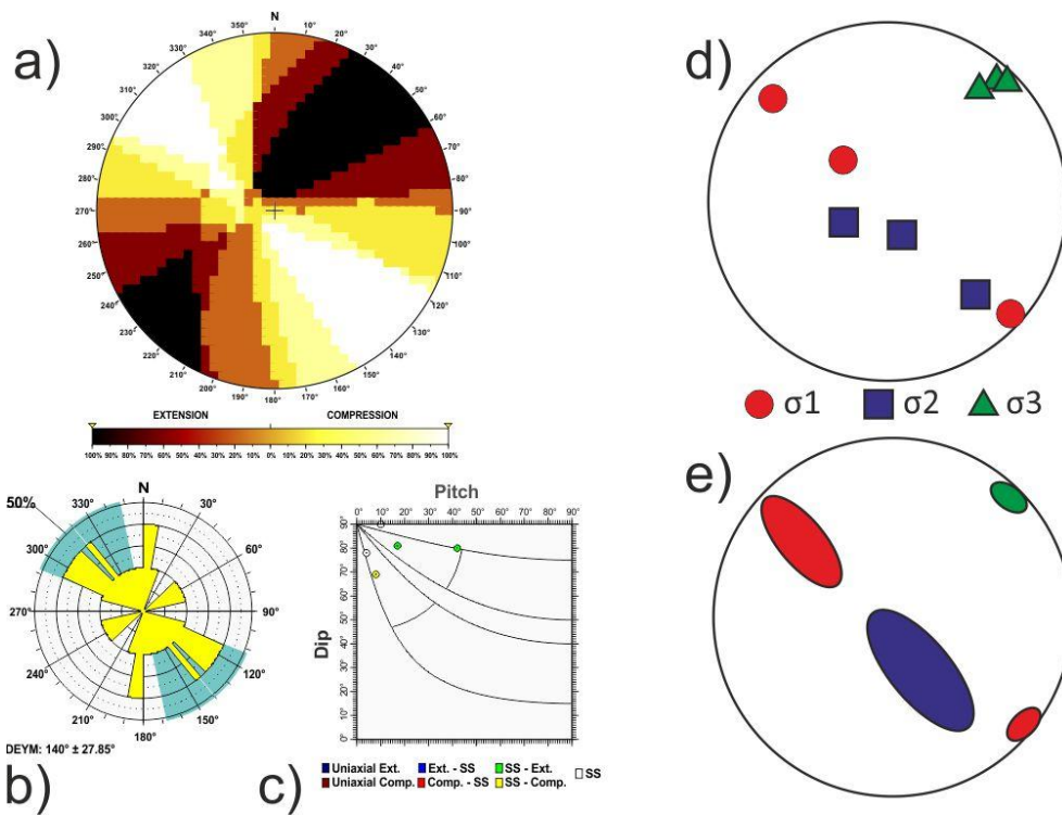
1515 Fig. B16 Offshore Atlantic tectonic zone. Results of the stress and strain analyses for different zones: a) Right Dihedra solution. b) Rose diagram of the Dey (horizontal shortening direction) obtained from the Slip model. C) Pitch/Dip plot for the neo-formed nodal planes obtained from the Slip Model. d) Stress Inversion Results. e) Variability of the three principal stress axes of the stress inversion.
