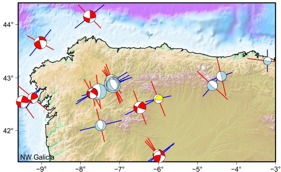
Mean tensors and Kagan angles
