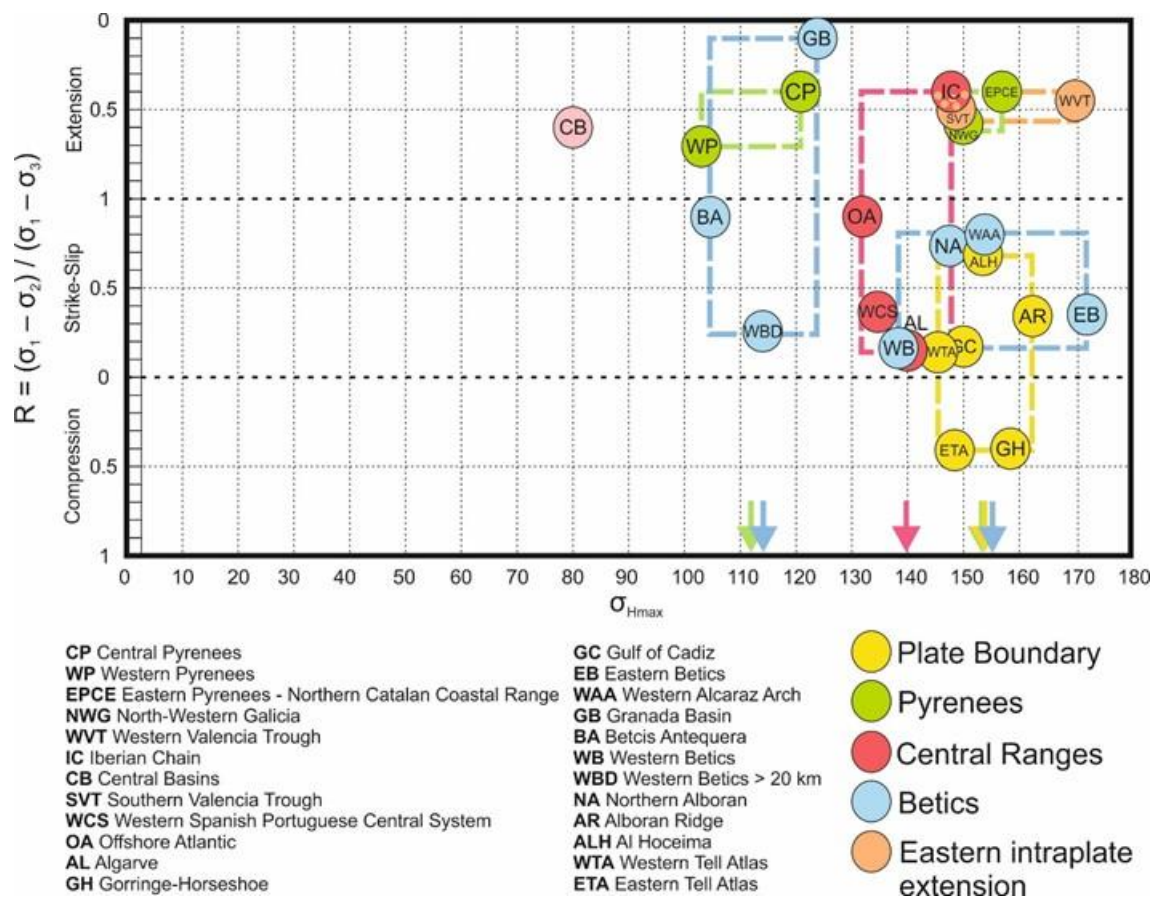
Figure 14: R (Stress tensor ratio) Vs S_{Hmax} trend ( \sigma_1 for thrusts and strike-slip faults stress regimes, \sigma_2 normal faulting stress regimes). The N-S direction is marked by 0^\circ and 180^\circ , while the E-W direction coincides with the value of 90^\circ . The areas considered have been grouped into those at the plate boundary (yellow, AR, GH, ETA, GC, WTA, and ALH), those in the Pyrenees (green, EPCE, NWG, CP, and WP), those in the Central Ranges (in red, OA, WCS, AL and IC), those in the Betics (in blue, separated BA, GB, WBD from the strike-slip solutions BA, GB, WBD), those related to the intraplate extension in E Iberia (Mediterranean) (in orange, WVT, SVT and IC. The latter is also included in the Central Ranges solution). CB (in pink) does not seem to be related to any of the previous groupings. The dashed rectangles mark each group's maximum and minimum values of R and S_{Hmax} , with their corresponding colour. The lower arrows indicate the average values of S_{Hmax} for each group.
