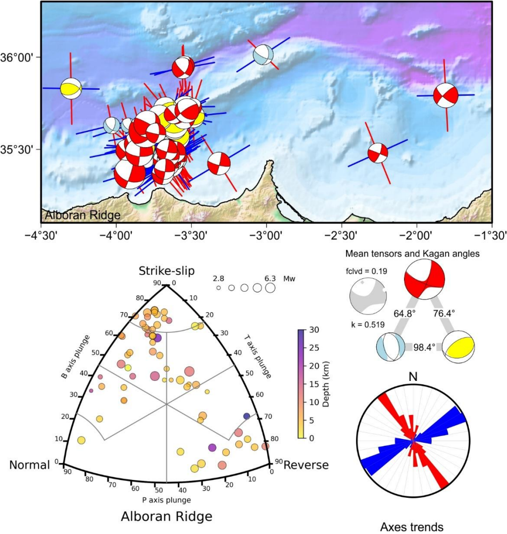
1175 Fig. A3: Alboran Ridge tectonic zone. Top map: focal mechanisms with maximum horizontal axis (P or B for normal ruptures) and minimum horizontal axis (T or B for reverse ruptures) orientation. Bottom left classification diagram for earthquake rupture types. Middle right: Average tensors (complete in gray) and Kagan angles between the average tensors for each rupture type. Bottom right: Rose diagram of maximum and minimum horizontal axes orientation.
