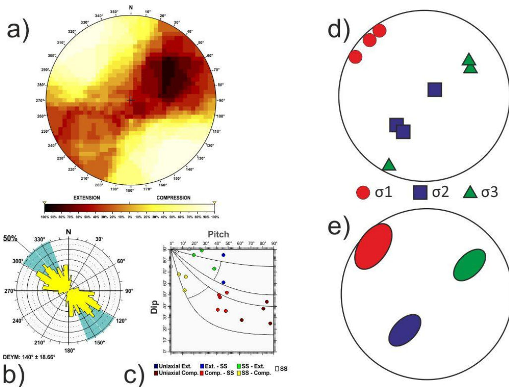
1580 Fig. B21 Western Spanish Portuguese Central System tectonic zone. Results of the stress and strain analyses for different zones: a) Right Dihedra solution. b) Rose diagram of the Dey (horizontal shortening direction) obtained from the Slip model. c) Pitch/Dip plot for the neo-formed nodal planes obtained from the Slip Model. d) Stress Inversion Results. e) Variability of the three principal stress axes of the stress inversion.
