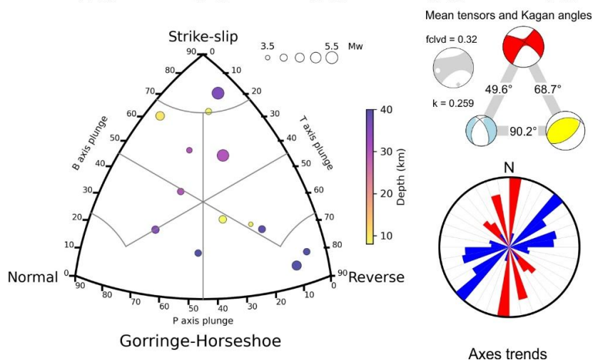
Fig. A12: Gorringshoeven tectonic zone. Top map: focal mechanisms with maximum horizontal axis (P or B for normal ruptures) and minimum horizontal axis (T or B for reverse ruptures) orientation. Bottom left classification diagram for earthquake rupture types. Middle right: Average tensors (complete in gray) and Kagan angles between the average tensors for each rupture type. Bottom right: Rose diagram of maximum and minimum horizontal axes orientation.
