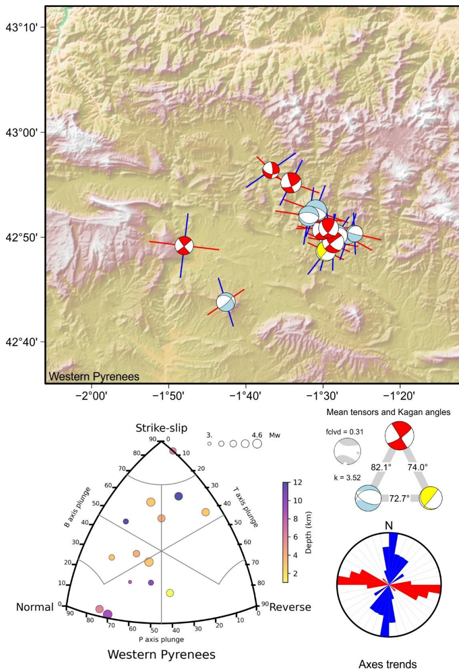
1285 Fig. A22: Western Pyrenees tectonic zone. Top map: focal mechanisms with maximum horizontal axis (P or B for normal ruptures) and minimum horizontal axis (T or B for reverse ruptures) orientation. Bottom left classification diagram for earthquake rupture types. Middle right: Average tensors (complete in gray) and Kagan angles between the average tensors for each rupture type. Bottom right: Rose diagram of maximum and minimum horizontal axes orientation.
