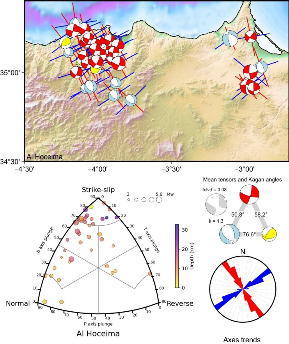
1155 Fig. A1: Al Hoceima tectonic zone. Top map: focal mechanisms with maximum horizontal axis (P or B for normal ruptures) and minimum horizontal axis (T or B for reverse ruptures) orientation. Bottom left classification diagram for earthquake rupture types. Middle right: Average tensors (complete in gray) and Kagan angles between the average tensors for each rupture type. Bottom right: Rose diagram of maximum and minimum horizontal axes orientation.
