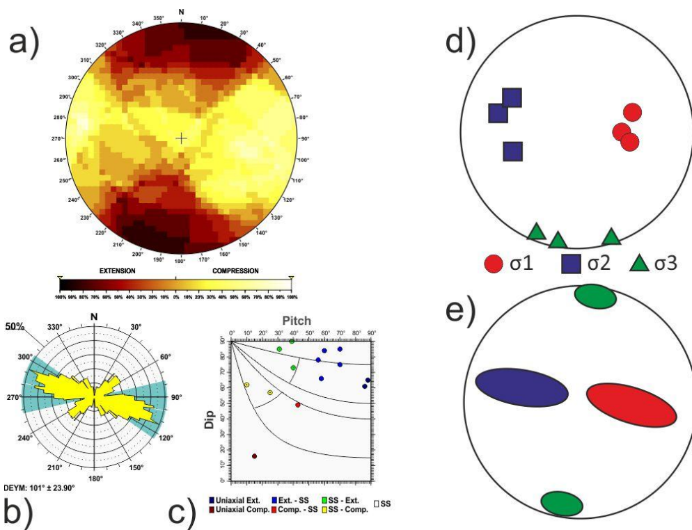
1590 Fig. B22 Western Pyrenees tectonic zone. Results of the stress and strain analyses for different zones: a) Right Dihedra solution. b) Rose diagram of the Dey (horizontal shortening direction) obtained from the Slip model. c) Pitch/Dip plot for the neo-formed nodal planes obtained from the Slip Model. d) Stress Inversion Results. e) Variability of the three principal stress axes of the stress inversion.
