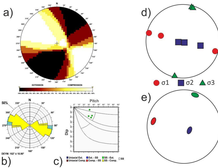
1350 Fig. B4 Betics Antequera tectonic zone. Results of the stress and strain analyses for different zones: a) Right Dihedra solution. b) 1355 Rose diagram of the Dey (horizontal shortening direction) obtained from the Slip model. C) Pitch/Dip plot for the neo-formed nodal 1360 planes obtained from the Slip Model. d) Stress Inversion Results. e) Variability of the three principal stress axes of the stress inversion.
