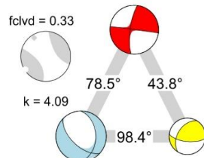
Mean tensors and Kagan angles
