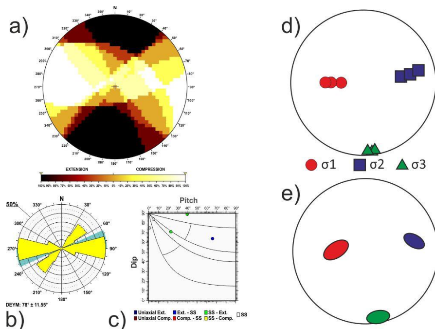
Fig. B5 Central Basins tectonic zone. Results of the stress and strain analyses for different zones: a) Right Dihedra solution. b) Rose diagram of the Dey (horizontal shortening direction) obtained from the Slip model. c) Pitch/Dip plot for the neo-formed nodal planes obtained from the Slip Model. d) Stress Inversion Results. e) Variability of the three principal stress axes of the stress inversion.
