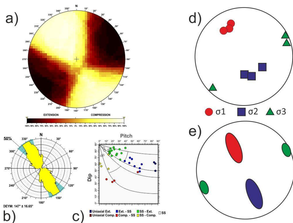
Fig. B1 Al Hoceima tectonic zone. Results of the stress and strain analyses for different zones: a) Right Dihedra solution. b) Rose diagram of the Dey (horizontal shortening direction) obtained from the Slip model. c) Pitch/Dip plot for the neo-formed nodal planes obtained from the Slip Model. d) Stress Inversion Results. e) Variability of the three principal stress axes of the stress inversion. e) Variability of the three principal stress axes of the stress inversion.
