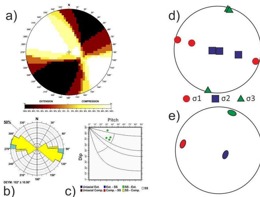
Fig. B4 Betics Antequera tectonic zone. Results of the stress and strain analyses for different zones: a) Right Dihedra solution. b) Rose diagram of the Dey (horizontal shortening direction) obtained from the Slip model. c) Pitch/Dip plot for the neo-formed nodal planes obtained from the Slip Model. d) Stress Inversion Results. e) Variability of the three principal stress axes of the stress inversion.
