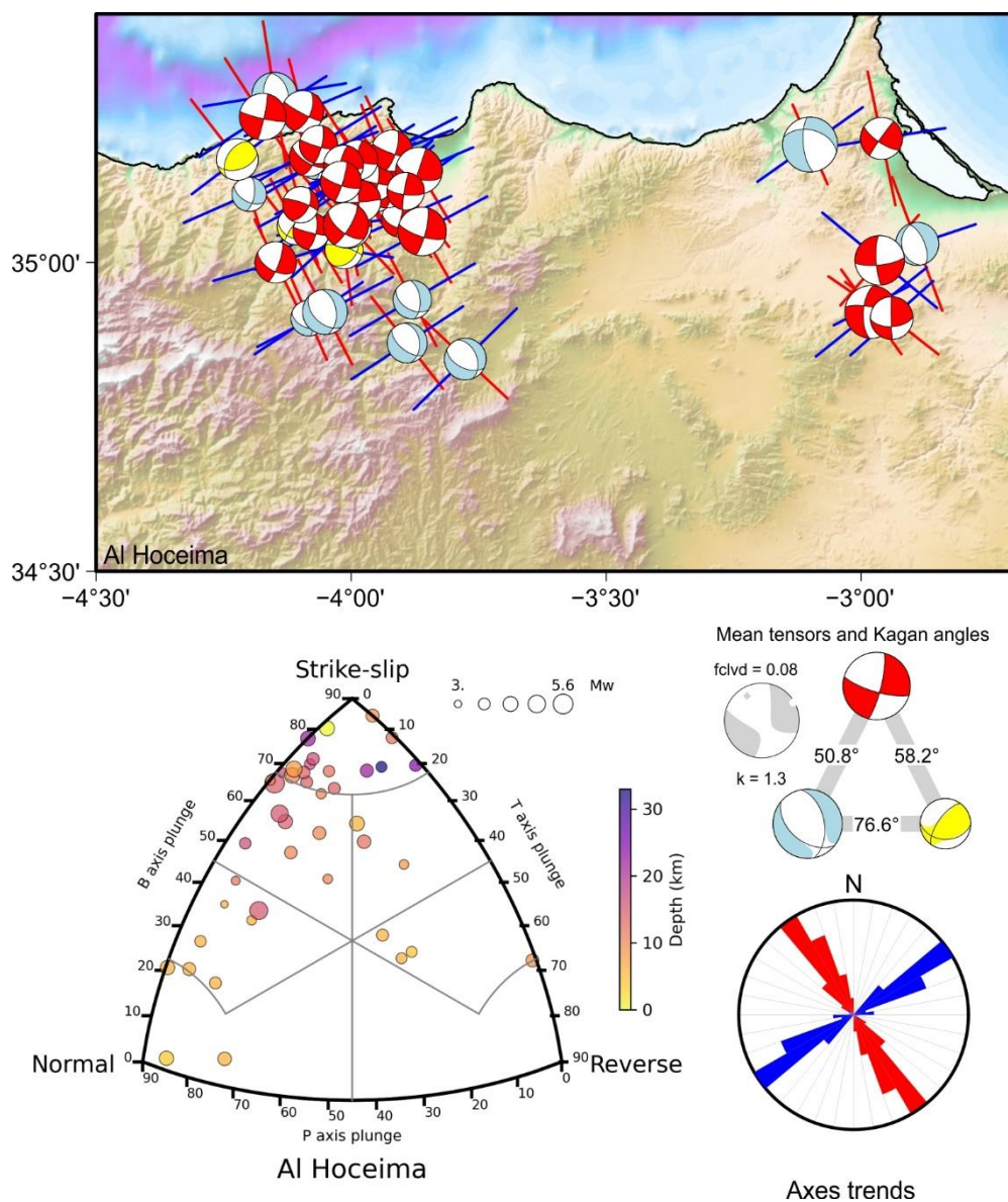
Fig. A1: Al Hoceima tectonic zone. Top map: focal mechanisms with maximum horizontal axis (P or B for normal ruptures) and minimum horizontal axis (T or B for reverse ruptures) orientation. Bottom left classification diagram for earthquake rupture types. Middle right: Average tensors (complete in gray) and Kagan angles between the average tensors for each rupture type. Bottom right: Rose diagram of maximum and minimum horizontal axes orientation.
