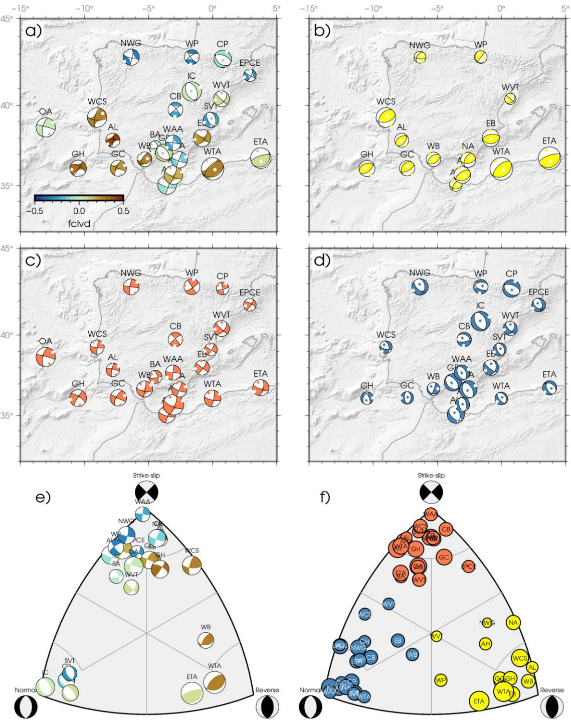
Figure 10: a) Combined strain focal mechanisms for each of the tectonic zones. The colour of the beach ball represents the compensated linear vector dipole factor fclvd. b) Combined focal mechanism for reverse faulting earthquakes in each zone. c) Combined focal mechanism for strike-slip earthquakes in each zone. d) Combined focal mechanism for normal earthquakes in
