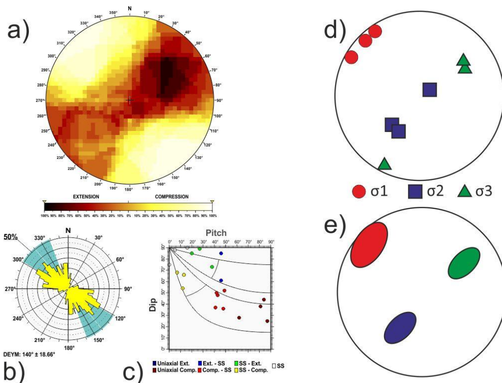
Fig. B20 Western Spanish Portuguese Central System tectonic zone. Results of the stress and strain analyses for different zones: a) Right Dihedra solution. b) Rose diagram of the Dey (horizontal shortening direction) obtained from the Slip model. c) Pitch/Dip plot for the neo-formed nodal planes obtained from the Slip Model. d) Stress Inversion Results. e) Variability of the three principal stress axes of the stress inversion.
