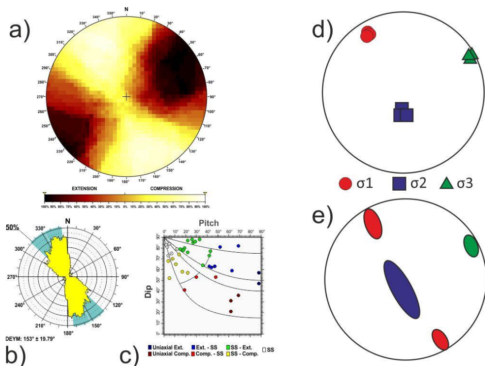
Fig. B14 Northern Alboran tectonic zone. Results of the stress and strain analyses for different zones: a) Right Dihedra solution. b) Rose diagram of the Dey (horizontal shortening direction) obtained from the Slip model. c) Pitch/Dip plot for the neo-formed nodal planes obtained from the Slip Model. d) Stress Inversion Results. e) Variability of the three principal stress axes of the stress inversion.
