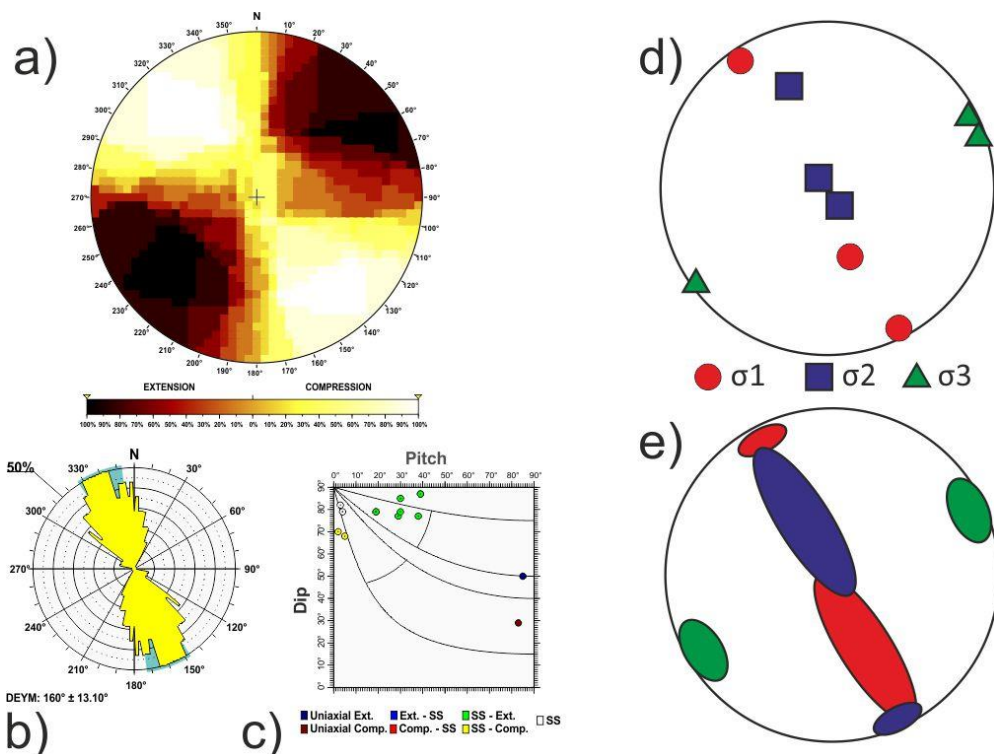
Fig. B18 Western Alcaraz Arch tectonic zone. Results of the stress and strain analyses for different zones: a) Right Dihedra solution. b) Rose diagram of the Dey (horizontal shortening direction) obtained from the Slip model. c) Pitch/Dip plot for the neo-formed nodal planes obtained from the Slip Model. d) Stress Inversion Results. e) Variability of the three principal stress axes of the stress inversion.
