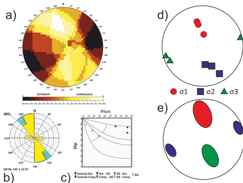
Fig. B8 Eastern Pyrenees tectonic zone. Results of the stress and strain analyses for different zones: a) Right Dihedra solution. b) Rose diagram of the Dey (horizontal shortening direction) obtained from the Slip model. c) Pitch/Dip plot for the neo-formed nodal planes obtained from the Slip Model. d) Stress Inversion Results. e) Variability of the three principal stress axes of the stress inversion.
