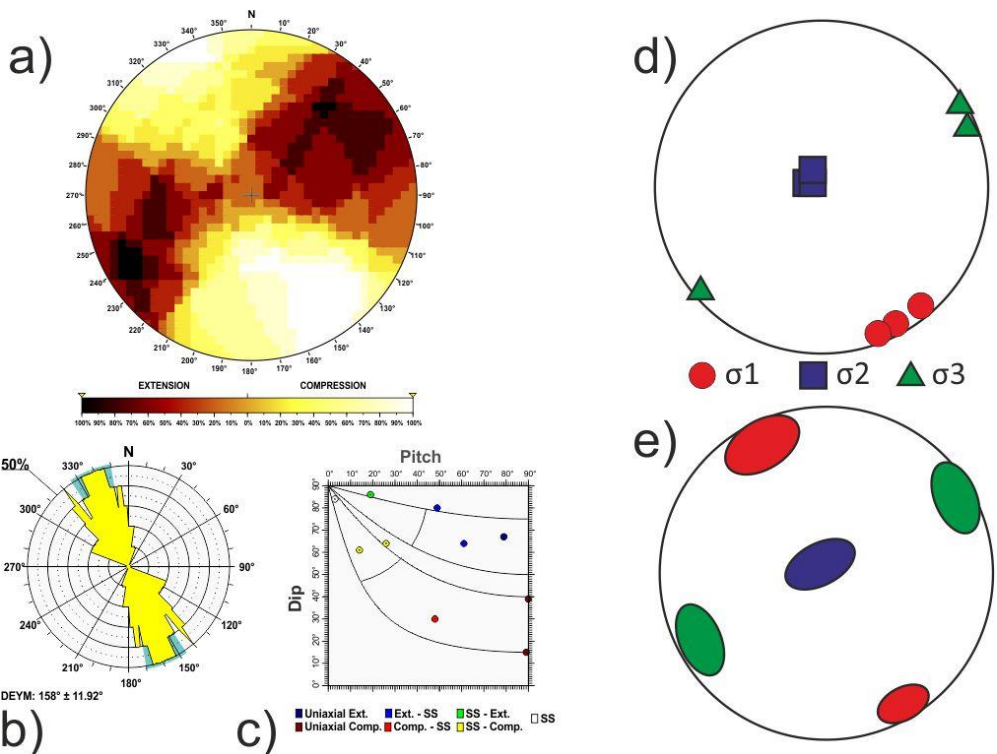
Fig. B11 Gulf of Cadiz tectonic zone. Results of the stress and strain analyses for different zones: a) Right Dihedra solution. b) Rose diagram of the Dey (horizontal shortening direction) obtained from the Slip model. c) Pitch/Dip plot for the neo-formed nodal planes obtained from the Slip Model. d) Stress Inversion Results. e) Variability of the three principal stress axes of the stress inversion.
