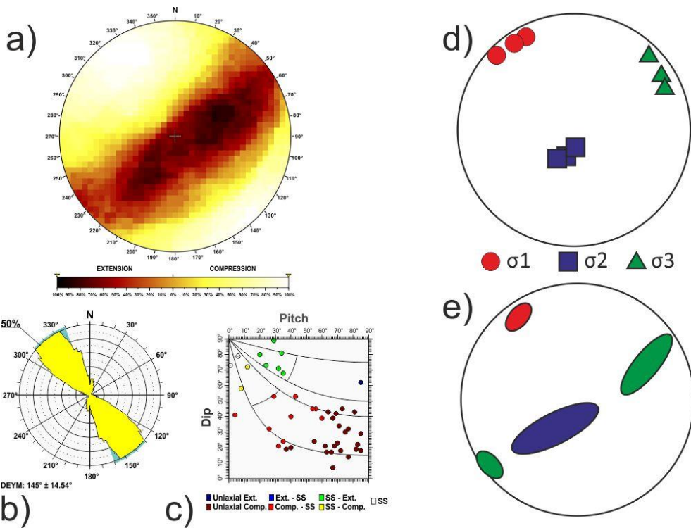
Fig. B22 West Tell Atlas tectonic zone. Results of the stress and strain analyses for different zones: a) Right Dihedra solution. b) Rose diagram of the Dey (horizontal shortening direction) obtained from the Slip model. c) Pitch/Dip plot for the neo-formed nodal planes obtained from the Slip Model. d) Stress Inversion Results. e) Variability of the three principal stress axes of the stress inversion.
