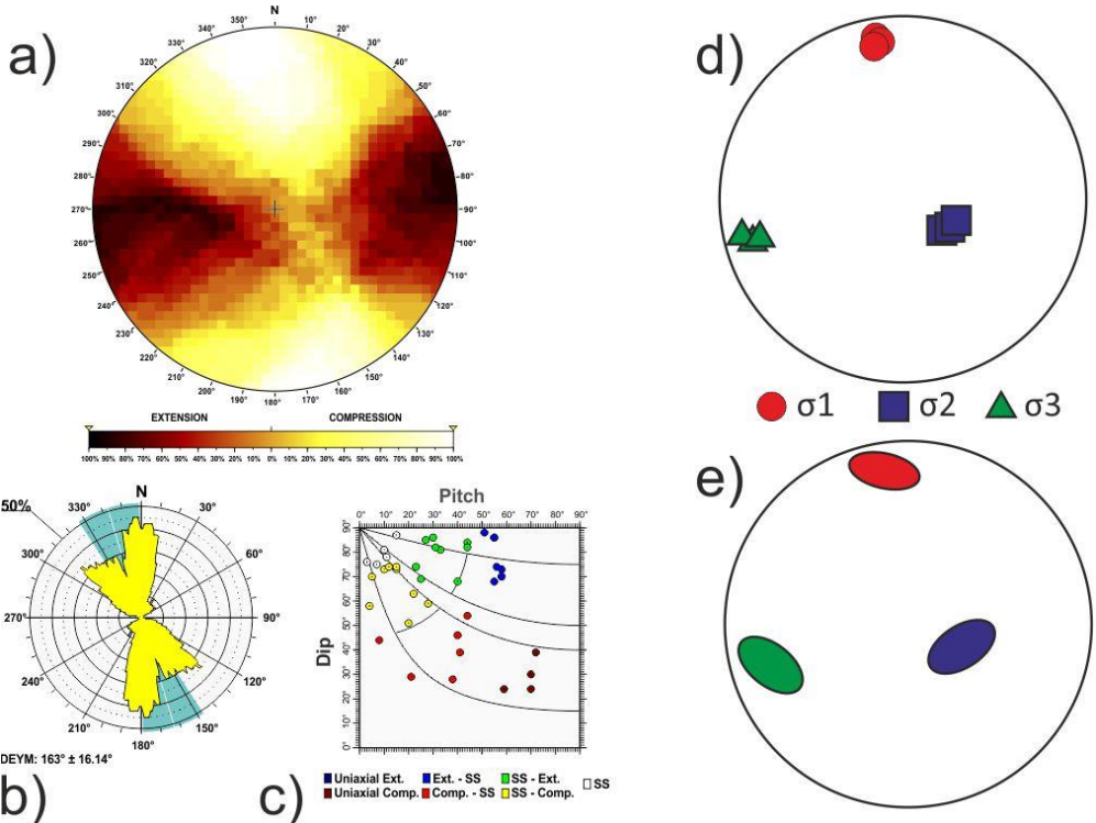
Fig. B7 Eastern Betics tectonic zone. Results of the stress and strain analyses for different zones: a) Right Dihedra solution. b) Rose diagram of the Dey (horizontal shortening direction) obtained from the Slip model. c) Pitch/Dip plot for the neo-formed nodal planes obtained from the Slip Model. d) Stress Inversion Results. e) Variability of the three principal stress axes of the stress inversion.
