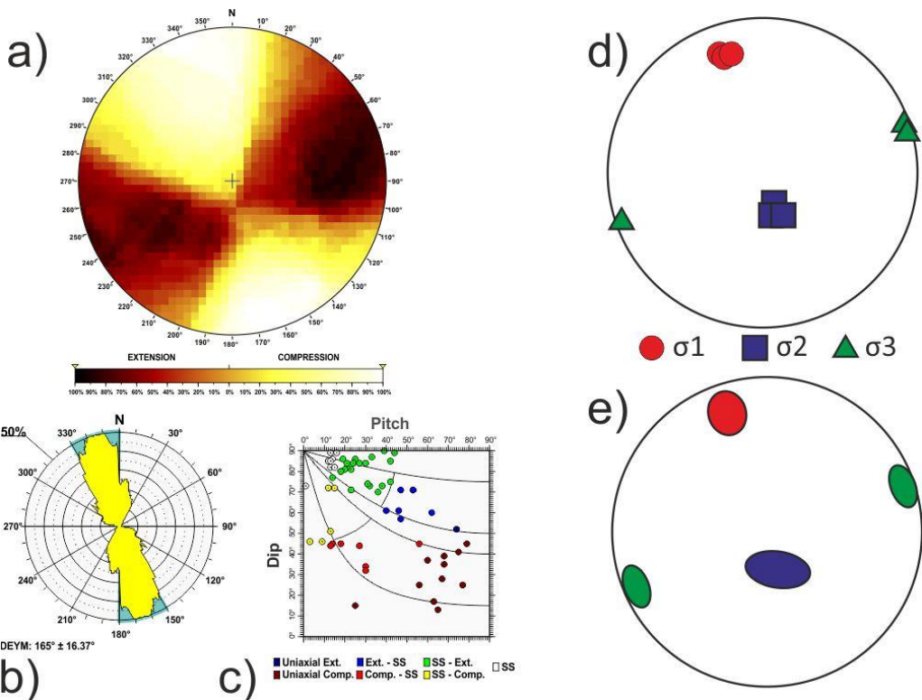
Fig. B3 Alboran Ridge tectonic zone. Results of the stress and strain analyses for different zones: a) Right Dihedra solution. b) Rose diagram of the Dey (horizontal shortening direction) obtained from the Slip model. c) Pitch/Dip plot for the neo-formed nodal planes obtained from the Slip Model. d) Stress Inversion Results. e) Variability of the three principal stress axes of the stress inversion.
