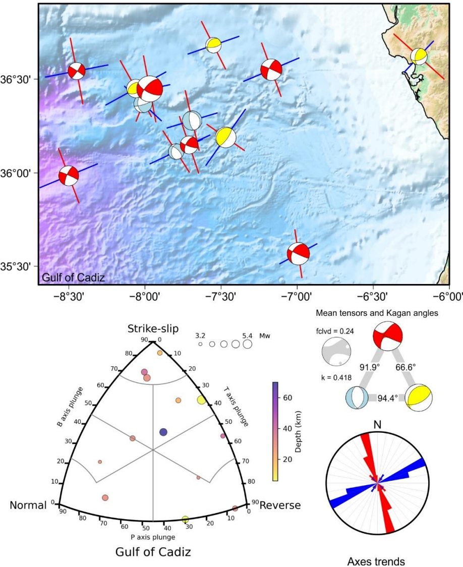
1085 Fig. A11: Gulf of Cadiz tectonic zone. Top map: focal mechanisms with maximum horizontal axis (P or B for normal ruptures) 1090 and minimum horizontal axis (T or B for reverse ruptures) orientation. Bottom left classification diagram for earthquake rupture types. Middle right: Average tensors (complete in gray) and Kagan angles between the average tensors for each rupture type. Bottom right: Rose diagram of maximum and minimum horizontal axes orientation.
