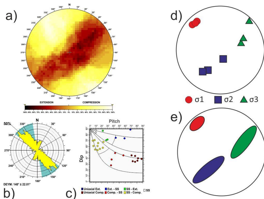
Fig. B19 Western Betics tectonic zone. Results of the stress and strain analyses for different zones: a) Right Dihedra solution. b) Rose diagram of the Dey (horizontal shortening direction) obtained from the Slip model. c) Pitch/Dip plot for the neo-formed nodal planes obtained from the Slip Model. d) Stress Inversion Results. e) Variability of the three principal stress axes of the stress inversion.
