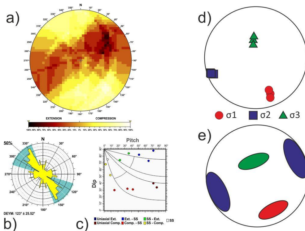
Fig. B12 Gorringe - Horseshoe tectonic zone. Results of the stress and strain analyses for different zones: a) Right Dihedra solution. b) Rose diagram of the Dey (horizontal shortening direction) obtained from the Slip model. c) Pitch/Dip plot for the neo-formed nodal planes obtained from the Slip Model. d) Stress Inversion Results. e) Variability of the three principal stress axes of the stress inversion.
