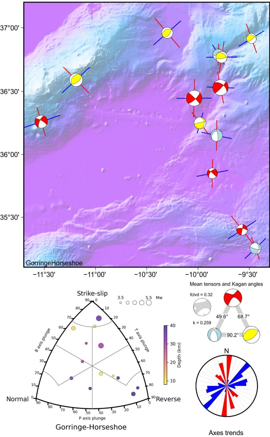
Fig. A12: Gorrington-Horseshoe tectonic zone. Top map: focal mechanisms with maximum horizontal axis (P or B for normal ruptures) and minimum horizontal axis (T or B for reverse ruptures) orientation. Bottom left classification diagram for earthquake rupture types. Middle right: Average tensors (complete in gray) and Kagan angles between the average tensors for each rupture type. Bottom right: Rose diagram of maximum and minimum horizontal axes orientation.
