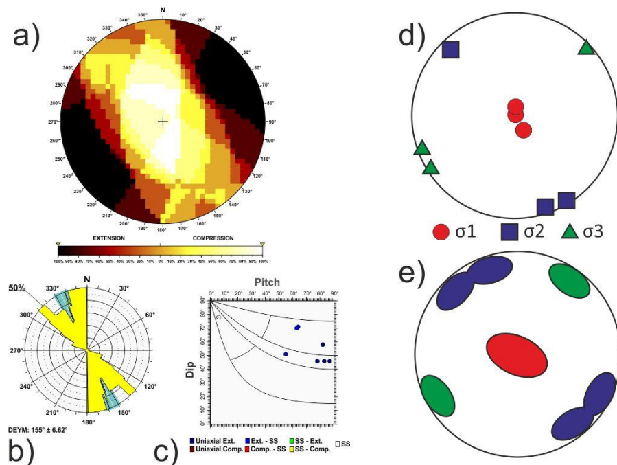
Fig. B13 Iberian Chain tectonic zone. Results of the stress and strain analyses for different zones: a) Right Dihedra solution. b) Rose diagram of the Dey (horizontal shortening direction) obtained from the Slip model. c) Pitch/Dip plot for the neo-formed nodal planes obtained from the Slip Model. d) Stress Inversion Results. e) Variability of the three principal stress axes of the stress inversion.
