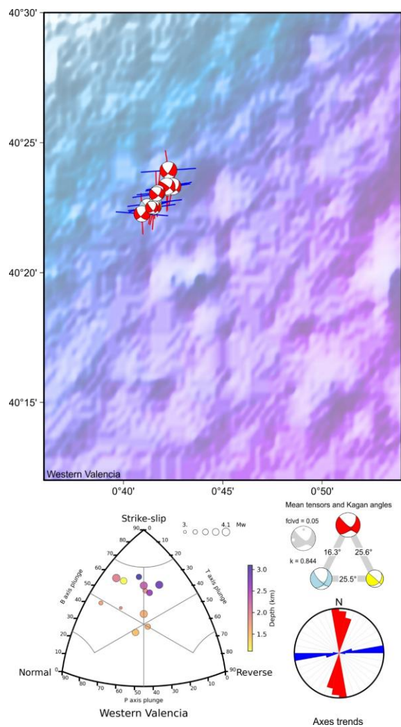
Fig. A24: Western Valencia tectonic zone. Top map: focal mechanisms with maximum horizontal axis (P or B for normal ruptures) and minimum horizontal axis (T or B for reverse ruptures) orientation. Bottom left classification diagram for earthquake rupture types. Middle right: Average tensors (complete in gray) and Kagan angles between the average tensors for each rupture type. Bottom right: Rose diagram of maximum and minimum horizontal axes orientation.
