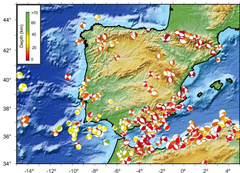
Figure 2: Distribution of the 542 focal mechanisms used in this study. The color of focal mechanisms indicates hypocentral depth.
