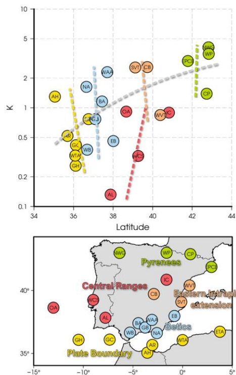
Figure 12: Relationship between the k-value of the strain tensor and the latitude of the zone. The colours are related to the tectonic setting as shown in the map. The coloured dashed lines show the trend of each population, while the grey dashed line shows the general trend of K-value increment with latitude.
