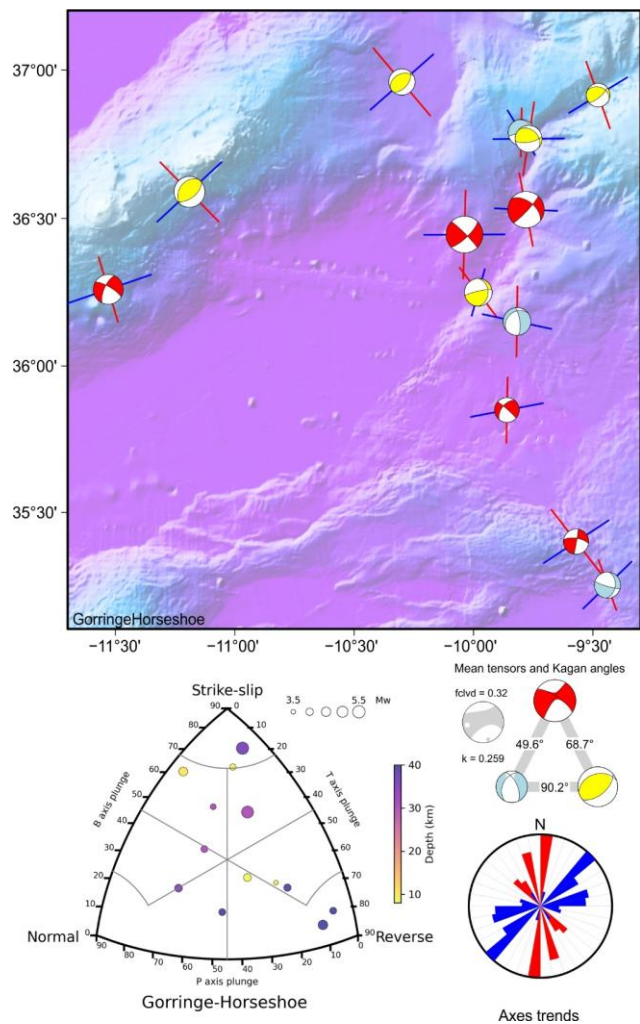
Fig. A12: Goringe-Horseshoe tectonic zone. Top map: focal mechanisms with maximum horizontal axis (P or B for normal ruptures) and minimum horizontal axis (T or B for reverse ruptures) orientation. Bottom left classification diagram for earthquake rupture types. Middle right: Average tensors (complete in gray) and Kagan angles between the average tensors for each rupture type. Bottom right: Rose diagram of maximum and minimum horizontal axes orientation.
