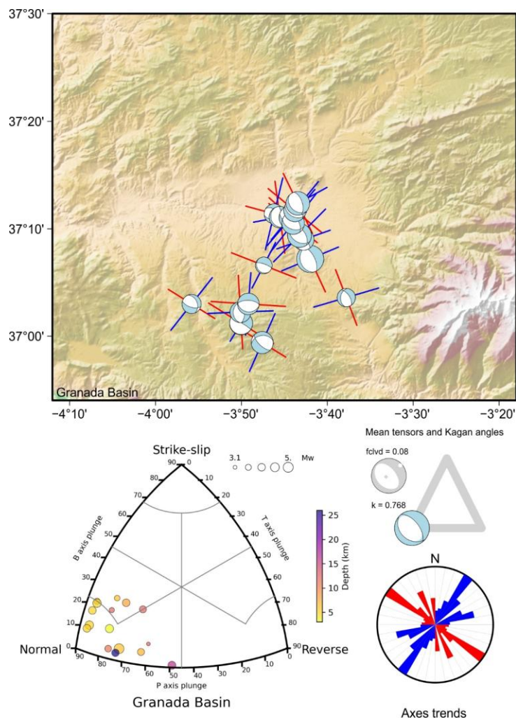
1375 Fig. A10: Granada Basin tectonic zone. Top map: focal mechanisms with maximum horizontal axis (P or B for normal ruptures) and minimum horizontal axis (T or B for reverse ruptures) orientation. Bottom left classification diagram for earthquake rupture types. Middle right: Average tensors (complete in gray) and Kagan angles between the average tensors for each rupture type. Bottom right: Rose diagram of maximum and minimum horizontal axes orientation.
