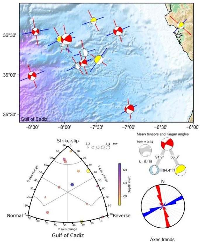
1380 Fig. A11: Gulf of Cádiz tectonic zone. Top map: focal mechanisms with maximum horizontal axis (P or B for normal ruptures) and minimum horizontal axis (T or B for reverse ruptures) orientation. Bottom left classification diagram for earthquake rupture types. Middle right: Average tensors (complete in gray) and Kagan angles between the average tensors for each rupture type. Bottom right: Rose diagram of maximum and minimum horizontal axes orientation.
