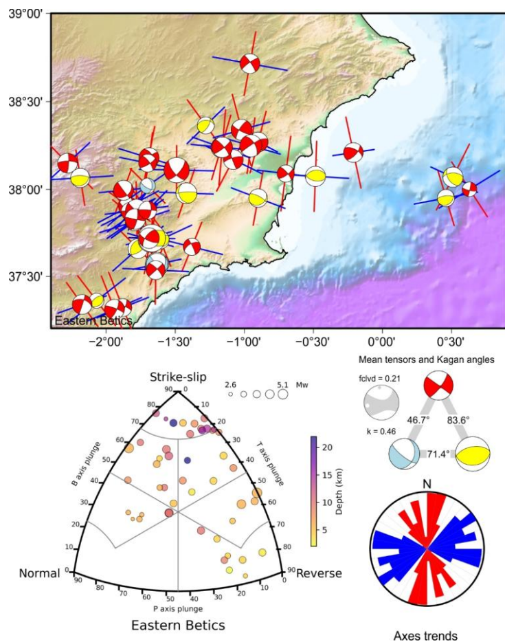
1355 Fig. A7: Eastern Betics tectonic zone. Top map: focal mechanisms with maximum horizontal axis (P or B for normal ruptures) and minimum horizontal axis (T or B for reverse ruptures) orientation. Bottom left classification diagram for earthquake rupture types. Middle right: Average tensors (complete in gray) and Kagan angles between the average tensors for each rupture type. Bottom right: Rose diagram of maximum and minimum horizontal axes orientation.
