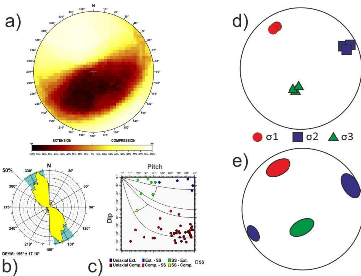
1570 Fig. B9 East Tell Atlas tectonic zone. Results of the stress and strain analyses for different zones: a) Right Dihedra solution. b) Rose diagram of the Dey (horizontal shortening direction) obtained from the Slip model. c) Pitch/Dip plot for the neo-formed nodal planes obtained from the Slip Model. d) Stress Inversion Results. e) Variability of the three principal stress axes of the stress inversion.
