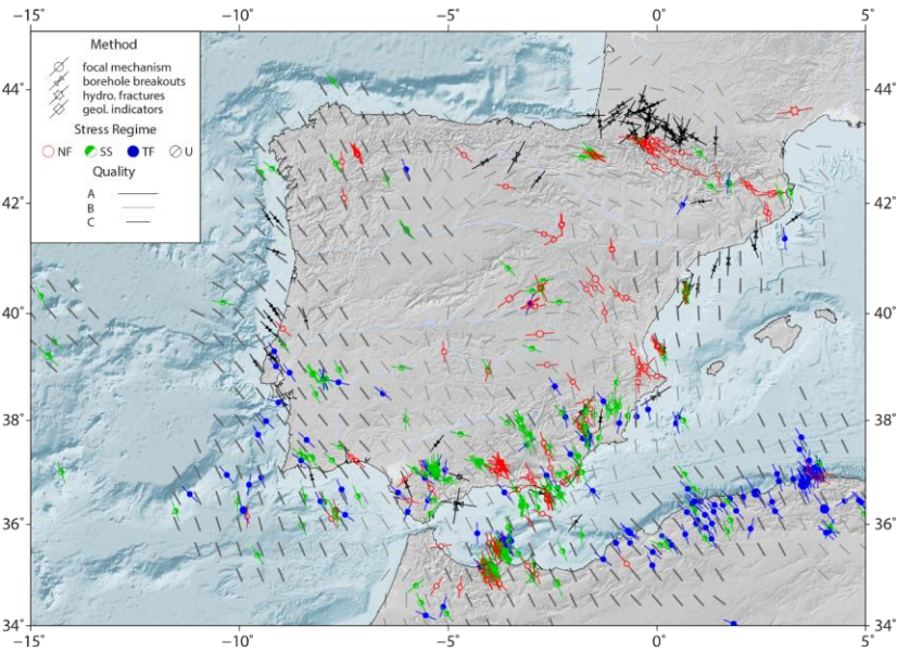
Figure 9: Stress map of Greater Iberia based on A-C quality data records from this study and from re-evaluated data of the WSM database release 2016 (Heidbach et al., 2016). Plotted is the orientation of maximum horizontal stress \sigma_{Hmax} for depths between 0-40 km. See the inset legend for details on data types, stress regime (NF= normal faulting, SS= strike-slip, TF= thrust faulting, U= unknown). Data symbols indicate the type of stress indicator and line length are proportional to data quality. Grey bars on a 0.5^\circ grid show the mean \sigma_{Hmax} orientation that is estimated with a search radius of 150 km using weights for data quality and distance to the grid point. Dark grey bars on the grid show mean \sigma_{Hmax} orientations with a standard deviation \leq 25^\circ , light grey bars with standard deviation > 25^\circ . Topography and bathymetry is taken from SRTM15+ (Tozer et al., 2019)
