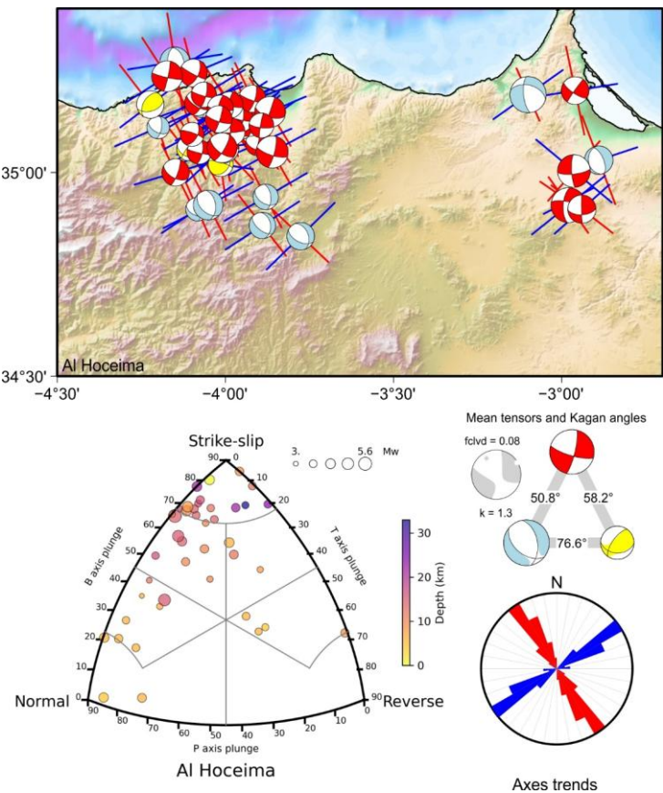
1310 Fig. A1: Al Hoceima tectonic zone. Top map: focal mechanisms with maximum horizontal axis (P or B for normal ruptures) and 1311 minimum horizontal axis (T or B for reverse ruptures) orientation. Bottom left classification diagram for earthquake rupture types. 1312 Middle right: Average tensors (complete in gray) and Kagan angles between the average tensors for each rupture type. Bottom 1313 right: Rose diagram of maximum and minimum horizontal axes orientation.
