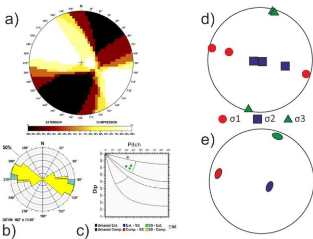
Fig. B4 Betic Antequera tectonic zone. Results of the stress and strain analyses for different zones: a) Right Dihedra solution. b) Rose diagram of the Dey (horizontal shortening direction) obtained from the Slip model. c) Pitch/Dip plot for the neo-formed nodal planes obtained from the Slip Model. d) Stress Inversion Results. e) Variability of the three principal stress axes of the stress inversion.
