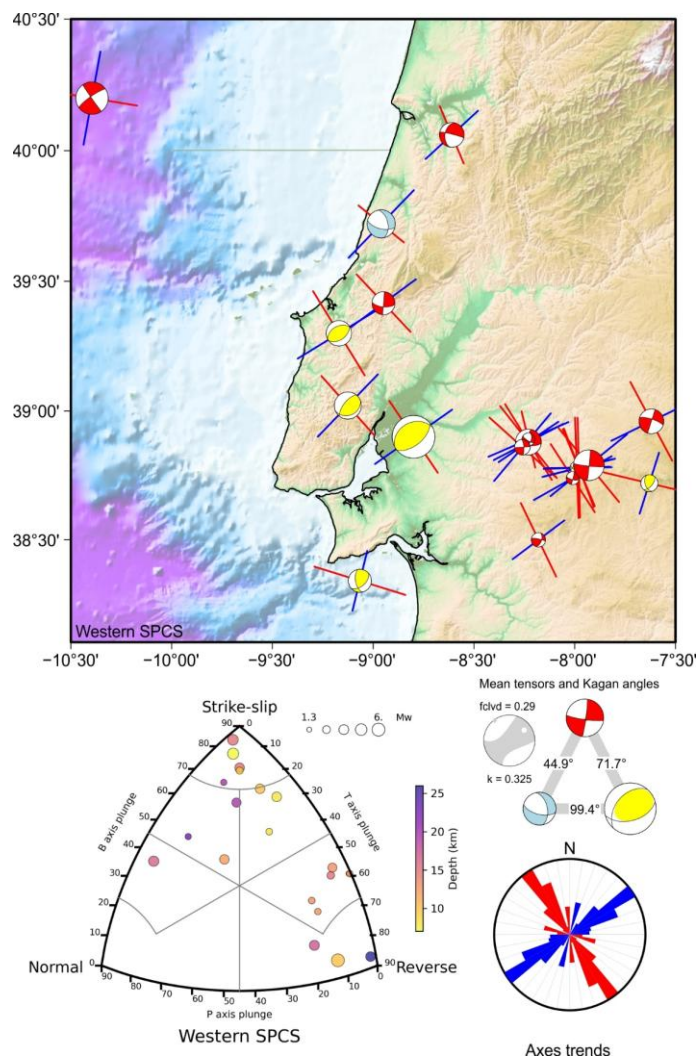
1435 Fig. A21: Western Spanish Portuguese Central System tectonic zone. Top map: focal mechanisms with maximum horizontal axis (P or B for normal ruptures) and minimum horizontal axis (T or B for reverse ruptures) orientation. Bottom left classification diagram for earthquake rupture types. Middle right: Average tensors (complete in gray) and Kagan angles between the average tensors for each rupture type. Bottom right: Rose diagram of maximum and minimum horizontal axes orientation.
