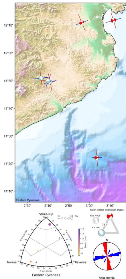
1365 Fig. A8: Eastern Pyrenees tectonic zone. Top map: focal mechanisms with maximum horizontal axis (P or B for normal ruptures) and minimum horizontal axis (T or B for reverse ruptures) orientation. Bottom left classification diagram for earthquake rupture types. Middle right: Average tensors (complete in gray) and Kagan angles between the average tensors for each rupture type. Bottom right: Rose diagram of maximum and minimum horizontal axes orientation.
