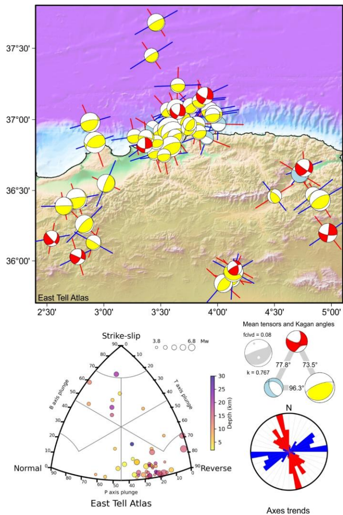
1370 Fig. A9: East Tell Atlas tectonic zone. Top map: focal mechanisms with maximum horizontal axis (P or B for normal ruptures) and minimum horizontal axis (T or B for reverse ruptures) orientation. Bottom left classification diagram for earthquake rupture types. Middle right: Average tensors (complete in gray) and Kagan angles between the average tensors for each rupture type. Bottom right: Rose diagram of maximum and minimum horizontal axes orientation.
