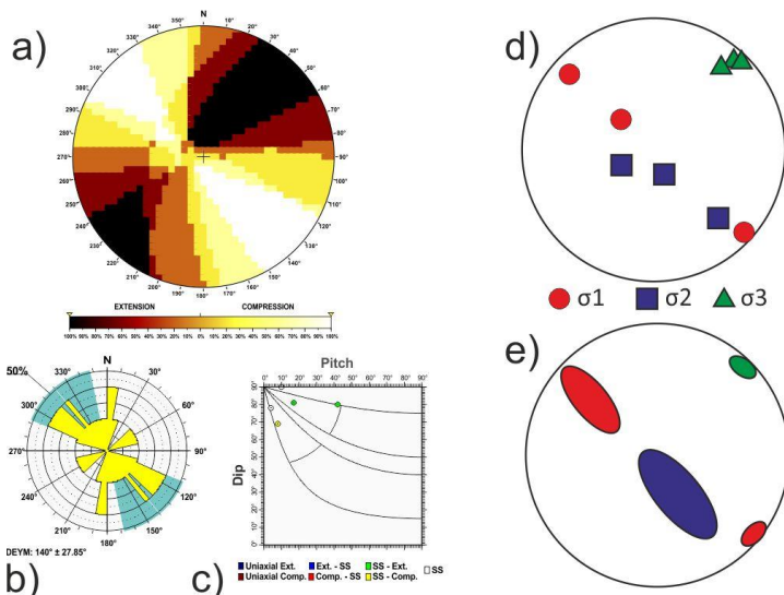
Fig. B16 Offshore Atlantic tectonic zone. Results of the stress and strain analyses for different zones: a) Right Dihedra solution. b) Rose diagram of the Dey (horizontal shortening direction) obtained from the Slip model. c) Pitch/Dip plot for the neo-formed nodal planes obtained from the Slip Model. d) Stress Inversion Results. e) Variability of the three principal stress axes of the stress inversion.
