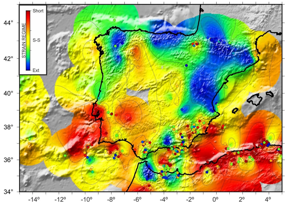
265 Figure 3: Style of active deformation (strain regime) for Iberia determined from focal mechanisms. The map shows the shape factor ( k' ) determined using the Slip Model (Reches, 1983 and de Vicente, 1988). Each dot represents a focal mechanism. Search radius of 150 km. Short.: shortening. S-S: shear strain. Ext.: extension.
