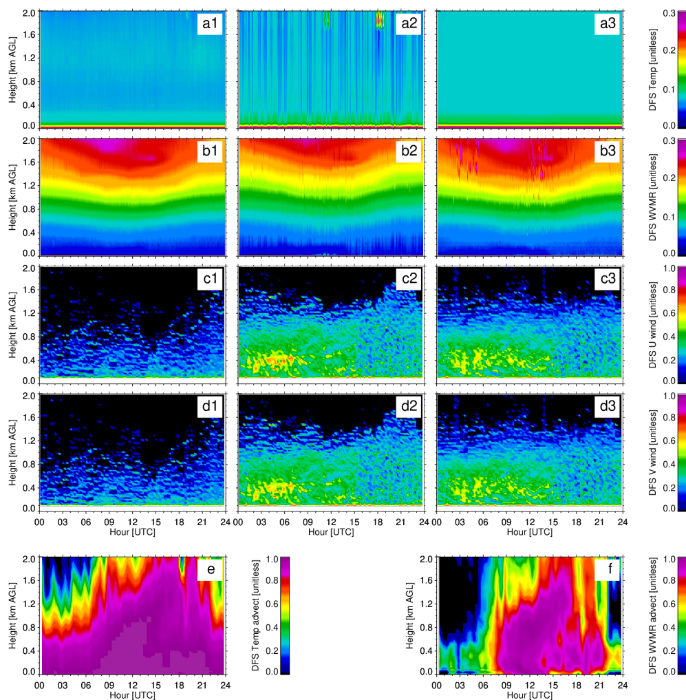
Figure 5: Same as Fig 2, but showing the DFS of the various products.
