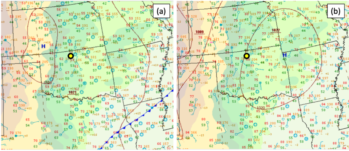
Fig 4: Surface synoptic maps at 0600 (a) and 1800 (b) on 13 June 2019. The yellow dot indicates the approximate location of the ARM C1 site. From the NOAA Weather Prediction Center map archive at https://www.wpc.ncep.noaa.gov/archives/web_pages/sfc/sfc_archive.php
