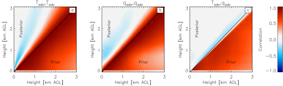
Fig 8: The level-to-level correlations between the advection of temperature/temperature (a), water vapor/water vapor (b), and temperature/water vapor (c) for 13 June 2019. The prior correlations are shown below the diagonal, and the posterior correlations are above the diagonal.
