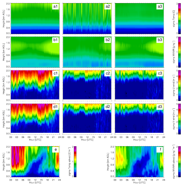
Figure 3: Same as Fig 2, but showing the 1-σ uncertainties of the various products, which were computed as the square root of the diagonal of the posterior covariance matrices.
