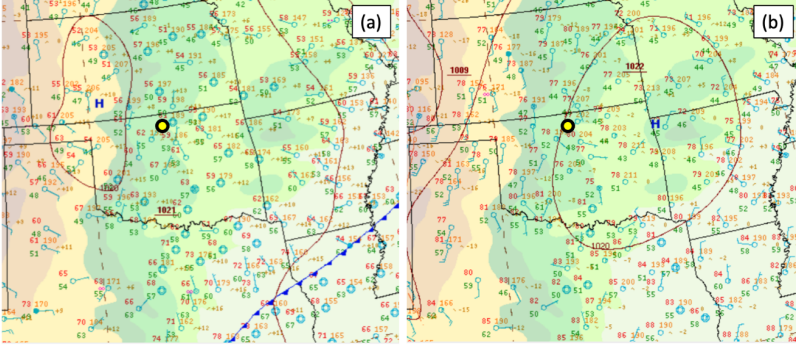
Fig 4: Surface synoptic maps at 0600 (a) and 1800 (b) on 13 June 2019. The yellow dot indicates the approximate location of the ARM C1 site. From the NOAA Weather Prediction Center map archive at https://www.wpc.ncep.noaa.gov/archives/web_pages/sfc/sfc_archive.php
