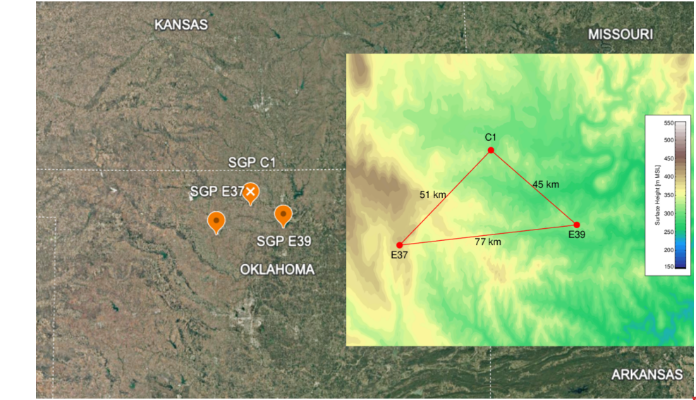
Figure 1: A satellite image of north central Oklahoma, showing the locations of the three sites used in this analysis ( extracted from Google Earth ). The inset shows the three sites, including the distances between them, where the background color indicates the elevation across the domain.
