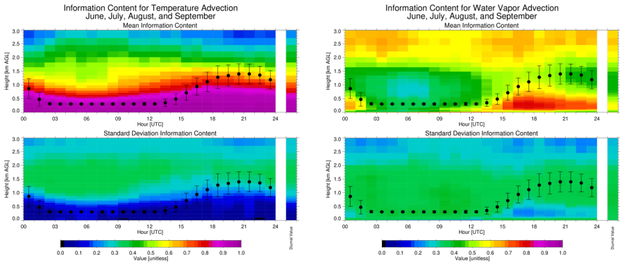
Figure 10: Same as Fig 8, but for the “warm season” (Table 1).
