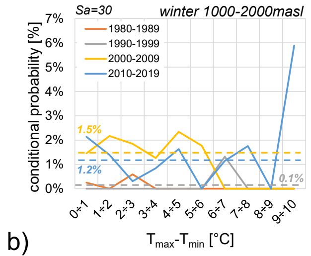
Figure 17. Conditional probabilities of rockfalls conditioned by ranges of temperature amplitude from 1970 to 2019: (a) during spring season below 1000 m a.s.l.; (b) during winter season between 1000 m-2000 m a.s.l.. Rockfall probabilities are represented by the coloured dotted lines according to the decade as shown in the legend.
