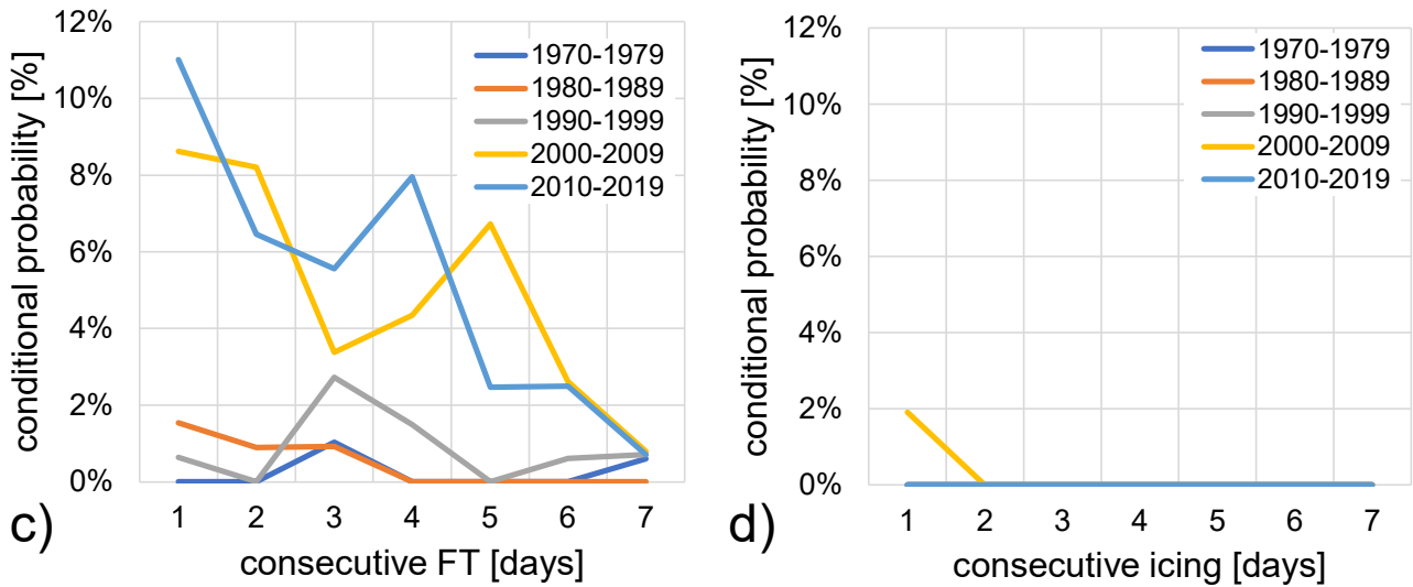
Figure 20. Conditional probabilities of rockfalls during spring between 1000 m a.s.l. and 2000 m a.s.l. from 1970 to 2019 with a 7 days aggregation scale. (a and c) triggered by freeze-thaw cycles with minimum and mean times-series. (b and d) triggered by icing with minimum and maximum time-series. Rockfall probabilities are represented by the coloured dotted lines according to the decade as shown in the legend.
