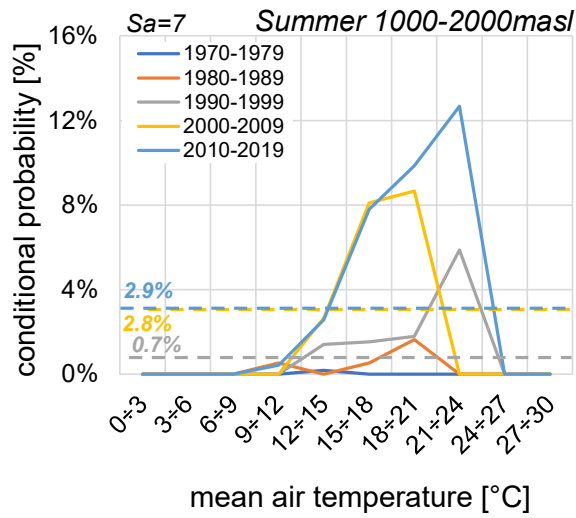
Figure 16. Conditional probabilities of rockfalls triggered by mean temperature values from 1970 to 2019: (a) during summer season between 1000-2000 m a.s.l. with an aggregation scale S_a = 7 days. (b) during autumn season above 2000 m a.s.l. with an aggregation scale S_a = 30 days. Rockfall probabilities are represented by the coloured dotted lines according to the decade as shown in the legend.
