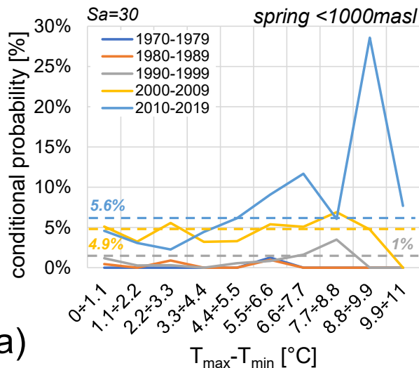
Figure 17. Conditional probabilities of rockfalls conditioned by ranges of temperature amplitude from 1970 to 2019: (a) during spring season below 1000 m a.s.l.; (b) during winter season between 1000 m-2000 m a.s.l.. Rockfall probabilities are represented by the coloured dotted lines according to the decade as shown in the legend.
