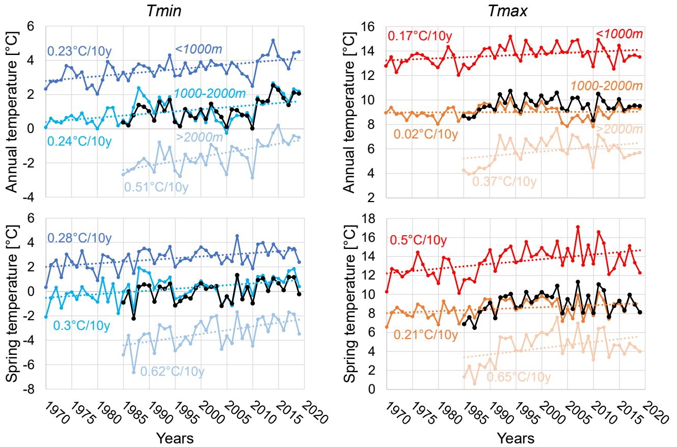
345 Figure 6. Annual and spring T_{min} and T_{max} trends considering 12 weather stations from 1970 to 2019 for case study. The lack line shows the mean time-series.
