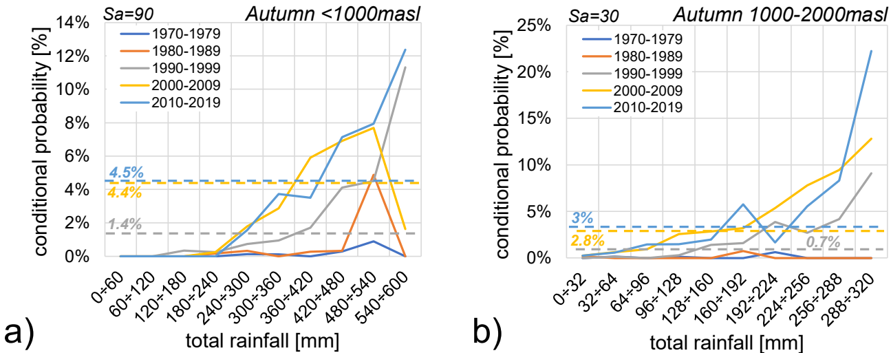
485 Figure 15. Conditional probabilities of rockfalls triggered by rainfall from 1970 to 2019 during autumn season: (a) below 1000 m a.s.l. considering an aggregation scale S_a = 90 days; (b) between 1000-2000 m a.s.l. with an aggregation scale S_a = 30 days. Rockfall probabilities are represented by the coloured dotted lines according to the decade as shown in the legend.
