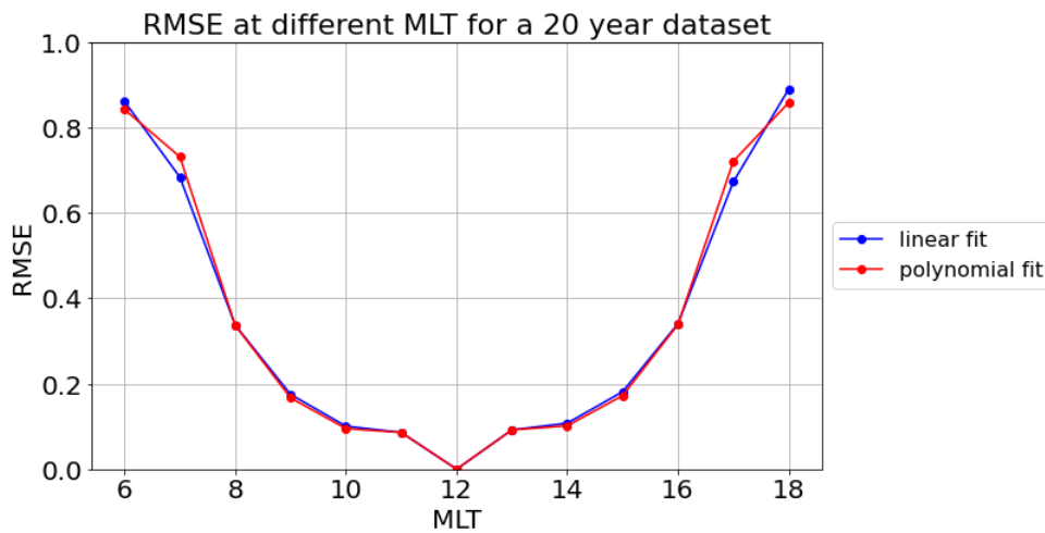
Figure 5: RMSE comparison between a polynomial fit and a linear fit in the model construction.
