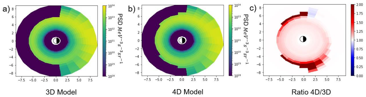
Figure 2: comparison between the phase space density of a Salammbô simulations at \mu = 5 MeV/G during the geomagnetic storm of march 2015 with the 3D magnetopause model (panel (a)), the 4D magnetopause mode (panel (b)) and the ratio of the two (panel (c))
