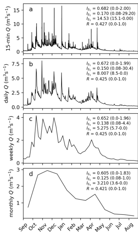
205 Figure 3. Effects of binning interval on inferred seasonality strength. An example hydrograph, given at 15-min (a), 210 daily (b), weekly (c), and monthly (d) resolution and the values of the associated seasonality metrics (Eqs. 3-5, and Eq. 8) with their possible range indicated in parentheses (constant regime – most seasonal regime). This indicates that traditional seasonality metrics tend to be more sensitive to the binning process than directional statistics are. This sensitivity is present in the absolute value of seasonality strength, the values relative to their potential minimum and maximum, and the reference values determining the possible seasonality range. Note that binning is not required for directional statistics.
