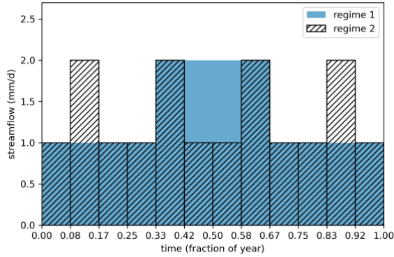
Figure 4. Comparison of streamflow regimes illustrating differences in assessing the strength of seasonality. While both regimes appear to have the same degree of seasonality when analysed using traditional metrics (Eqs. 3-5), directional statistics quantify that flow regime 1 is seasonal ( R=0.21 ), whereas flow regime 2 is non-seasonal ( R=0.0 ) due to identical flow rates throughout the different seasons.
