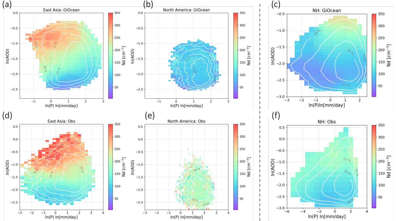
Figure 7. Cloud droplet number ( N_d ) composited on AOD and precipitation rate in GiOcean (abc) and from observations (def) and in the regions off the coast of East Asia (ad), North America (be) and Northern hemisphere ocean (cf). The density of points is indicated by white contours. The percentage labeled on each contour represents the fraction of monthly data points contained within that contour. The outermost white contour encloses the 2-D density region containing 95% of the monthly data points, effectively excluding extreme outliers.
