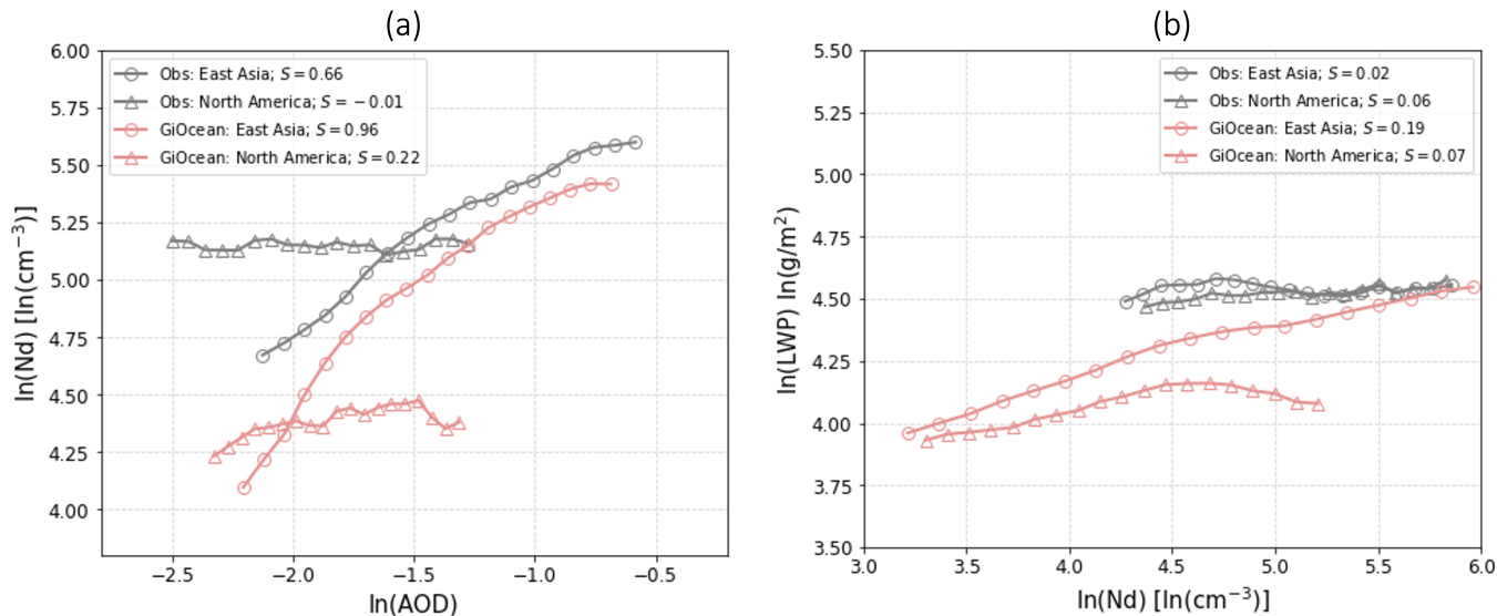
Figure 6. (a) Inferred sensitivity ( S ) of cloud droplet number concentration ( \text{Nd} ) to aerosol optical depth ( \text{AOD} ), and (b) inferred sensitivity of liquid water path ( \text{LWP} ) to \text{Nd} , based on both GiOcean (pink) and satellite observations (gray) in the outflow regions of East Asia (circles) and North America (triangles), using the sensitivity metrics defined in Eq 1 and Eq 2.
