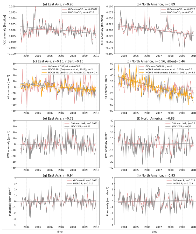
Figure 5. The monthly anomaly time series in the outflow regions of East Asia (a,c,e,g) and North America (b,d,f,h) from GiOcean (pink) and satellite observations (gray or orange). AOD (a, b), Nd (c, d), LWP (e, f), and precipitation rate (g, h). The GiOcean outputs and the sources of satellite observations are consistent with the description in Figure 2. Monthly anomalies are calculated by removing the long-term monthly climatology from the original time series. The correlation ( r ) between the monthly anomaly time series of GiOcean and satellite observations is shown in the panel title. r(\text{Ben}) is the correlation between Bennartz Nd (Bennartz and Rausch, 2017) and GiOcean COSP Nd. Linear trend lines are shown for each dataset in the line labels, with the slope ( s ) indicating the trend per month. Units of slope: a, b in 1/\text{month} ; c, d in \text{cm}^{-3}/\text{month} ; e, f in \text{g}, \text{m}^{-2}/\text{month} ; and g, h in \text{mm}, \text{day}^{-1}/\text{month} .
