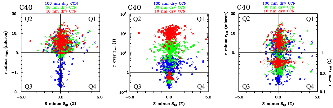
380 Fig. 8. Results for C40 simulations from GKY24. The same data as in Fig. 6, but on the modified phase diagram and with smaller number of points (0.5% for each dry CCN radius). Red/green/blue colors represent droplets formed on CCN of 10/30/100 nm dry radius. The same data is shown in all panels. The left panel applies the difference between droplet radius and critical radius on the vertical axis. The middle panel uses the ratio between the droplet radius and the critical radius. The right panel applies the difference between droplet radius and critical radius when the difference is positive (quarters Q1 and Q2), and the ratio between the droplet radius and the critical radius in Q3 and Q4 quarters.
