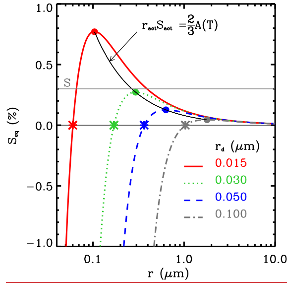
Fig. 1. Examples of KoehlerKöhler curves for selected dry radii of NaCl ( \kappa = 1.28 ) and temperature of 273.16 K. Critical supersaturations and critical radii are marked as large dots. Radii corresponding to S_{eq} = 0 are marked as large stars. See text for discussion.
