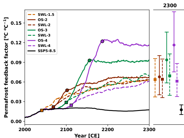
Figure 8. Timeseries of permafrost feedback factor under stabilization (dashed lines) and overshoot (solid lines) scenarios for 1.5 °C (orange), 2.0 °C (sienna), 3.0 °C (green), and 4.0 °C (purple) global warming levels, as well as the SSP5-8.5 scenario (black). Square markers indicate the time points when the temperature overshoot reaches its peak or stabilized warming begins, while circle markers indicate when the overshoot returns to 1.5 °C. Results represent the ensemble median of 250 simulations. Dots on the adjacent right panels represent values in the year 2300, with uncertainty ranges estimated as the 5th to 95th percentiles. The permafrost feedback factor is calculated as the ratio of additional global warming caused by the permafrost carbon feedback (i.e., the difference between the PFC and NPFC simulations) to the global mean temperature change in the NPFC simulations.
