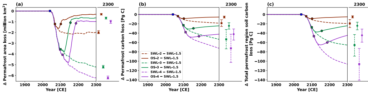
285 Figure 4. Similar to Figure 3, but showing timeseries of changes relative to the SWL-1.5 scenario in (a) permafrost area loss, (b) permafrost carbon loss, and (c) total permafrost region soil carbon loss under stabilization and overshoot scenarios for 2.0 °C (sienna brown), 3.0 °C (green), and 4.0 °C (purple) global warming levels. Square markers indicate the time points when the temperature overshoot reaches its peak or stabilized warming begins, while circle markers indicate when the overshoot returns to 1.5 °C. Results represent the ensemble median of 250 simulations based on the PFC simulations. Dots on the adjacent right panels represent values in the year 2300, with uncertainty ranges estimated as the 5th to 95th percentiles.
