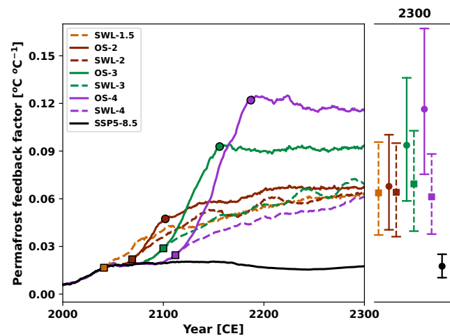
Figure 8. Timeseries of permafrost feedback factor under stabilization (dashed lines) and overshoot (solid lines) scenarios for 1.5 °C (orange), 2.0 °C ( sienna brown ), 3.0 °C (green), and 4.0 °C (purple) global warming levels, as well as the SSP5-8.5 scenario (black). Square markers indicate the time points when the temperature overshoot reaches its peak or stabilized warming begins, while circle markers indicate when the overshoot returns to 1.5 °C. Results represent the ensemble median of 250 simulations. Dots on the adjacent right panels represent values in the year 2300, with uncertainty ranges estimated as the 5th to 95th percentiles. The permafrost feedback factor is calculated as the ratio of additional global warming caused by the permafrost carbon feedback (i.e., the difference between the PFC and NPFC simulations) to the global mean temperature change in the NPFC simulations.
