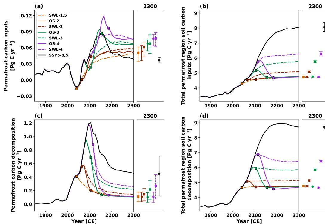
Figure 5. Timeseries of changes in (a) permafrost carbon inputs, (b) total permafrost region soil carbon inputs, (c) permafrost carbon decomposition and (d) total permafrost region soil carbon decomposition, under the stabilization (dashed lines) and overshoot (solid lines) scenarios for 1.5 °C (orange), 2.0 °C (brown), 3.0 °C (green), and 4.0 °C (purple) global warming levels, along with the SSP5-8.5 scenario (black). Square markers indicate the time points when the temperature overshoot reaches its peak or stabilized warming begins, while circle markers indicate when the overshoot returns to 1.5 °C. Results represent the ensemble median of 250 simulations based on the PFC simulations. Dots on the adjacent right panels represent values in the year 2300, with uncertainty ranges estimated as the 5th to 95th percentiles.
