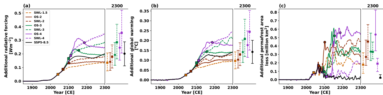
Figure 7. Additional changes in (a) radiative forcing, (b) global warming and (c-d) permafrost area loss due to permafrost carbon feedback, calculated as the difference between the PFC and NPFC simulations. Results are shown under stabilization (dashed lines) and overshoot (solid lines) scenarios for 1.5 °C (orange), 2.0 °C ( sienna brown ), 3.0 °C (green), and 4.0 °C (purple) global warming levels, along with the SSP5-8.5 scenario (black). Square markers indicate the time points when the temperature overshoot reaches its peak or stabilized warming begins, while circle markers indicate when the overshoot returns to 1.5 °C. Results represent the ensemble median of 250 simulations. Dots on the adjacent right panels represent values in the year 2300, with uncertainty ranges estimated as the 5th to 95th percentiles. In panel (a), the additional radiative forcing is calculated using the simplified expressions (Etminan et al., 2016) based on simulated CO 2 concentrations. In panel (c), the additional permafrost area loss is smoothed using a 5-year rolling average to eliminate interannual variability.
