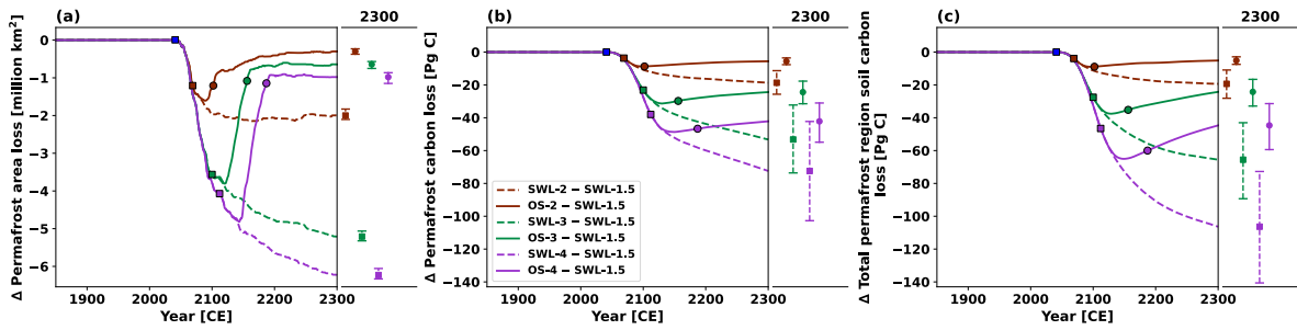
Figure 4. Similar to Figure 3, but showing timeseries of changes relative to the SWL-1.5 scenario in (a) permafrost area loss, (b) permafrost carbon loss, and (c) total permafrost region soil carbon loss under stabilization and overshoot scenarios at for 2.0 °C ( greensienna ), 3.0 °C ( redgreen ), and 4.0 °C (purple) global warming levels. Square markers indicate the time points when the temperature overshoot reaches its peak or stabilized warming begins, while circle markers indicate when the overshoot returns to 1.5 °C. Results represent the ensemble median of 250 simulations based on the PFC simulations. Dots on the adjacent right panels represent values in the year 2300, with uncertainty ranges estimated as the 5th to 95th percentiles.
