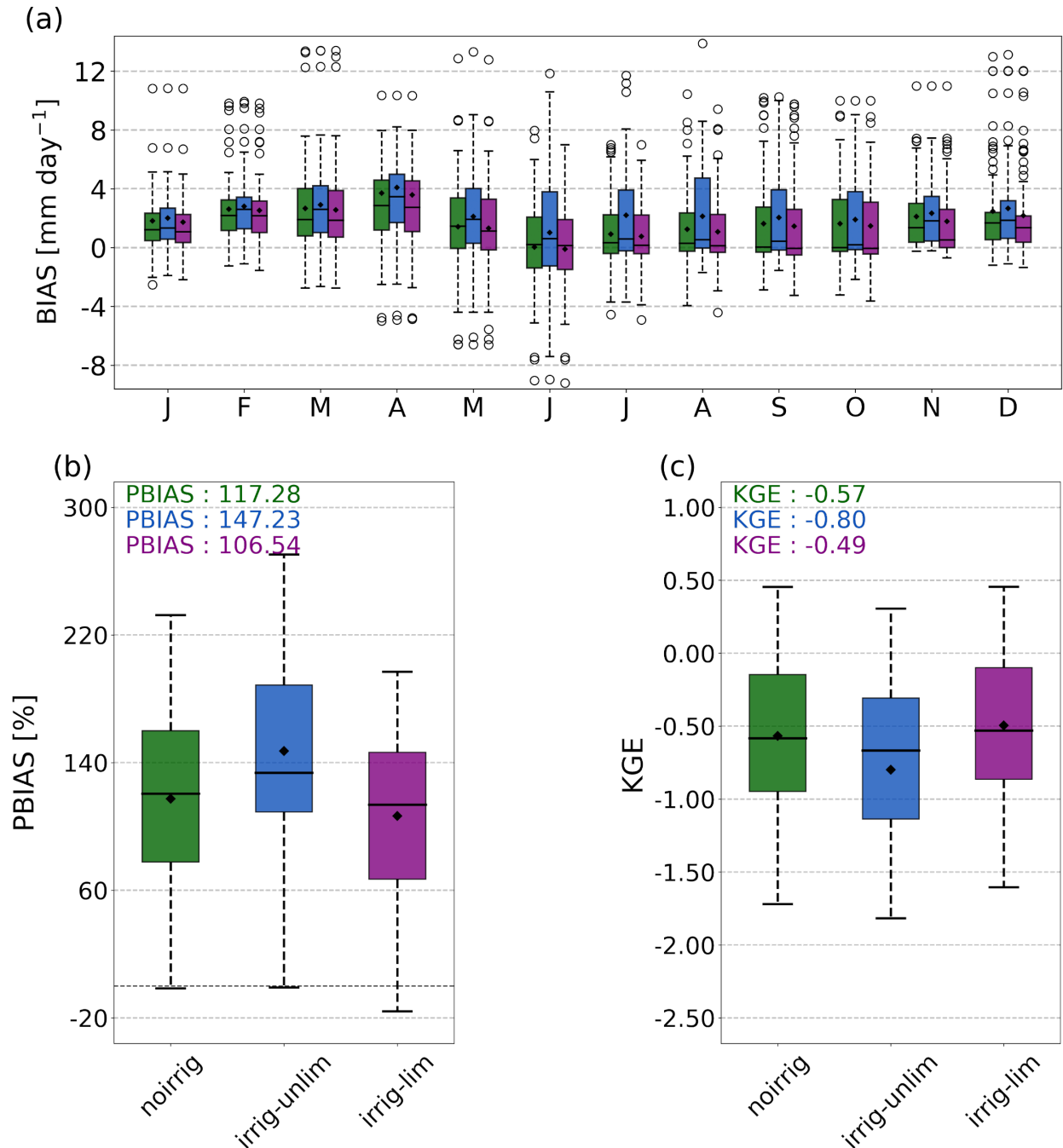
Figure 8. Evaluation of simulated streamflow in 77 irrigation-affected catchments. (a) Multi-year average monthly streamflow bias simulated using the noirrig, irrig-unlim, and irrig-lim schemes in the evaluation catchments. The boxes represent the interquartile range, black lines
