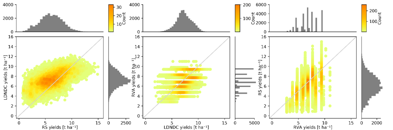
Figure A1: Pairwise relationships of parcel-level annual yield estimates for meadows and mowing pastures in the study area in 2019 based on Remote Sensing, LandscapeDNDC simulations and the reference values approach with histograms of the three modelling approaches. Note, that the colour ranges differ for the subplots.
