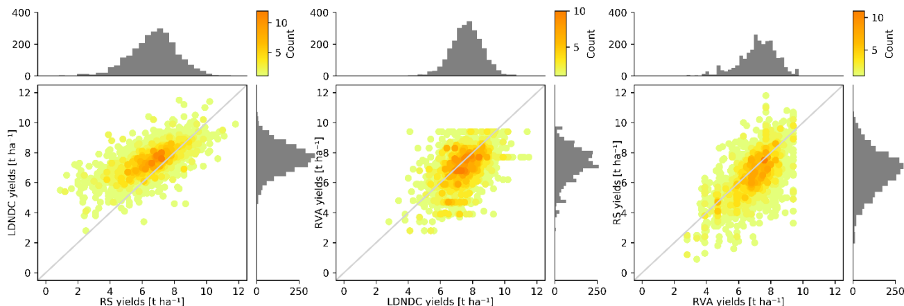
390 Figure 8: Pairwise relationships of spatially aggregated (hexagon diagonal length of 1km) annual yield estimates for meadows and mowing pastures in the study area in 2019 based on Remote Sensing, LandscapeDNDC simulations and the reference values approach with histograms of the three modelling approaches.
