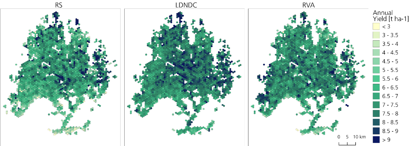
Figure 6: Spatially aggregated (hexagon diagonal length of 1km) annual yield estimates for meadows and mowing pastures in the study area in 2019 based on Remote Sensing, LandscapeDNDC simulations and the reference values approach. Hexagons for which the grassland area is smaller than 1 ha are not shown.
