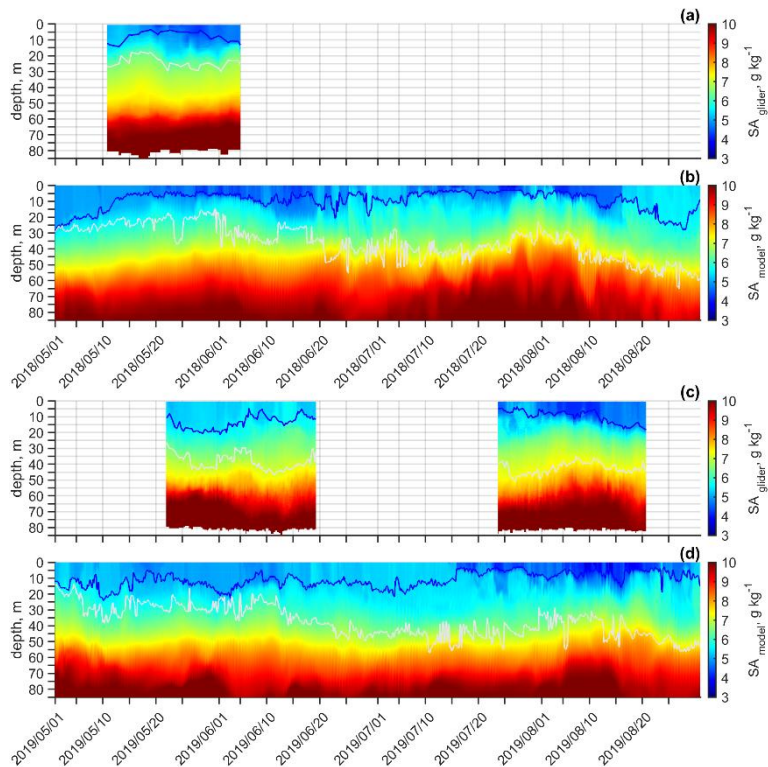
The figure above shows salinity variability based on glider data (panels a, c) and model output (panels b, d) for May–August 2018 (a, b) and 2019 (c, d). The glider data represent average profiles for each section within the selected area, forming a composite data field. The model data correspond to average profiles within a 1 \times 1 km window, providing a profile at each model timestep. The blue and white lines show the UML and CIL depth, respectively.
