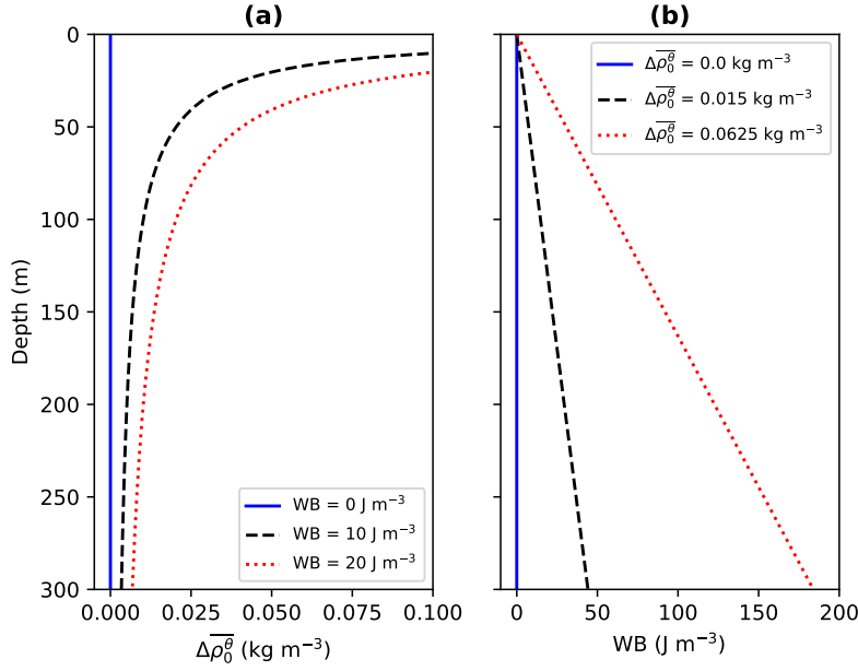
Figure 2. Relationship between the degree of density inhomogeneity ( \Delta\rho_0^c ) along the water column and the corresponding WB required to displace a water parcel from any depth to the surface (Eq. 5). Profiles are shown for various single values of (a) WB and (b) \Delta\rho_0^c .
