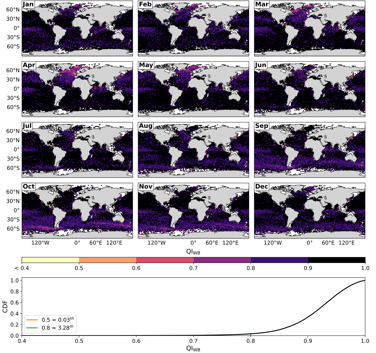
Figure 5. Upper panel: global monthly climatology of QI_{WB} for the EBM-MLD, considering \Delta\rho_0^{\theta} = 0.0150 \text{ kg m}^{-3} . Lower panel: the cumulative density function (CDF) of the conjoint distribution in space and time of QI_{WB} , with two QI_{WB} values and their corresponding percentiles shown.
