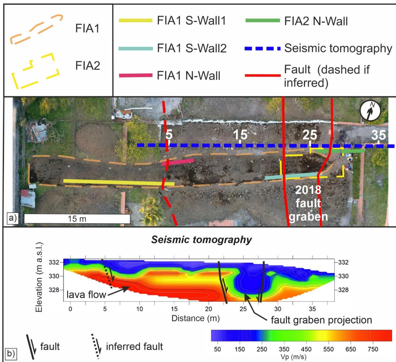
245 Figure 6: Map of Fiandaca trench site: a) orthophoto mosaic obtained by aerial drone photos showing FIA1 and FIA2 with sectors 250 of the walls investigated in detail, and faults in accordance with the 2018 coseismic ruptures; dashed blue line is the trace of seismic tomography showed in (b).
