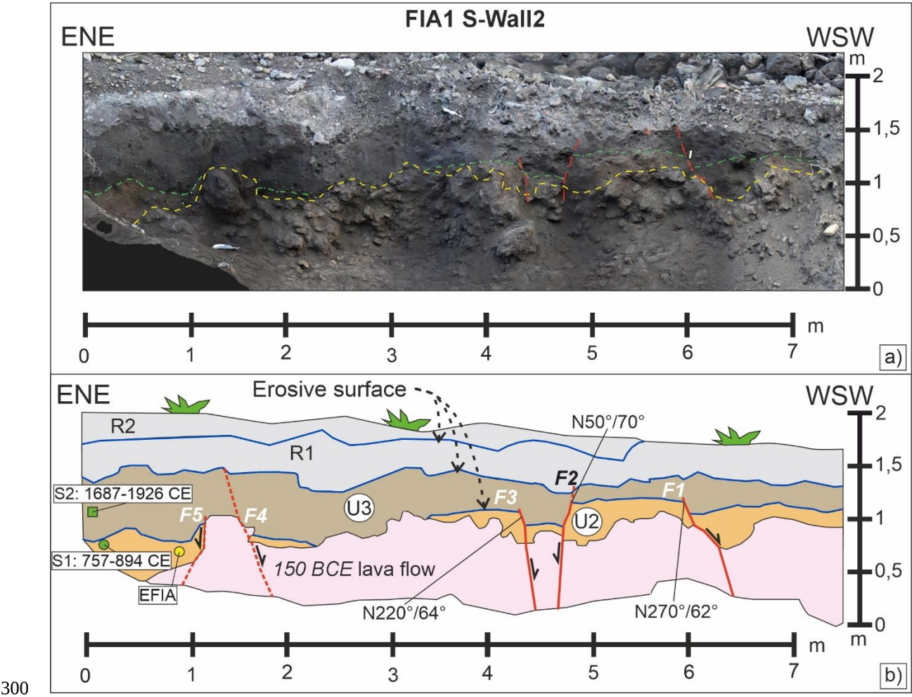
Figure 8: a) Orthophoto mosaic of the FIA1 S-Wall: the yellow dashed line is the top of the lava flow, the green dashed line is top of U2, the fault planes are shown in red. b) reconstruction of the stratigraphic succession along the FIA1 S-Wall; the fault planes in
