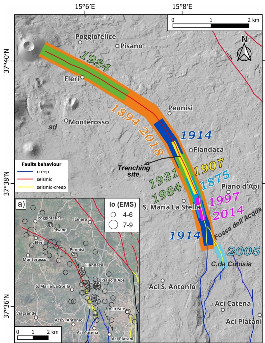
160 Figure 3: Map showing 1875 CE to present surface faulting events along the Fiandaca Fault, coloured segments represent the earthquake ruptures (modified after Azzaro et al., 2022; Tringali et al., 2023a). In the inset (a) the seismicity around the Fiandaca Fault from 1633 CE, I_0 is the epicentral intensity (after Azzaro and D'Amico, 2014).
