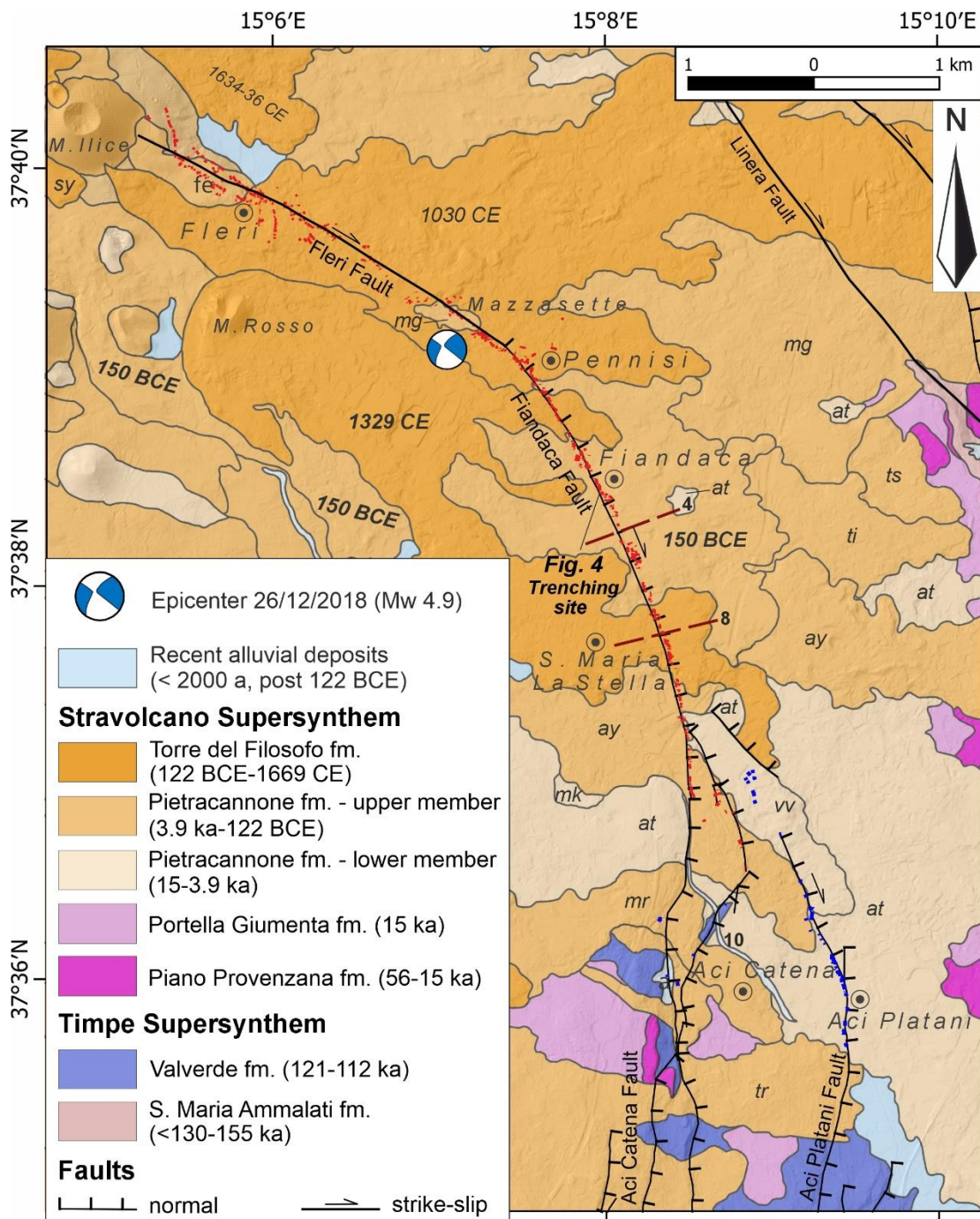
Figure 2: Geological map of Mt. Etna E flank around the Fiandaca Fault (modified after Branca et al., 2011; Azzaro et al., 2012; Barreca et al., 2013; ITHACA Working group, 2019); in red the coseismic ruptures of the 26 December 2018 earthquake, in blue the fractures related to the subsequent aseismic creep event (modified after Tringali et al., 2023a); dark red dashed lines are selected profiles across faulted lava flows (n. 5, 10); lava flows chronologically labelled: sy: Case Scandurra (850±40 CE); mg: M. Gorna; mr: M. Serra; ay: Piano d'Api; tr: Trecastagni; ti: Timone; fe: Fleri; ts: Castelluccio; mk: Monaci; vv: Villa Vincenzina; at: Aci Platani.
