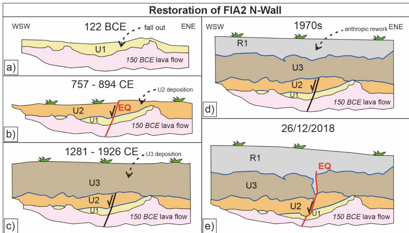
350 Figure 11: Possible restoration of the FIA2 N-Wall. a) pyroclastic fallout (122 BC Plinian eruption) is deposited on the 150±200 BC lava flow, subsequently partially eroded and reworked because of its exposure to the surface; b) an earthquake occurred during the deposition of the colluvial deposit of U2 in the period 757-894 AD; c) after an erosive event on U2, the deposition of the colluvial deposit of U3 occurred in the period 1281-1926 AD; d) reworking of the surface by the human activity and formation of the R1 during the 1970s; e) earthquake in 2018 displacing the lava flow, U1, U2, U3 and R1.
