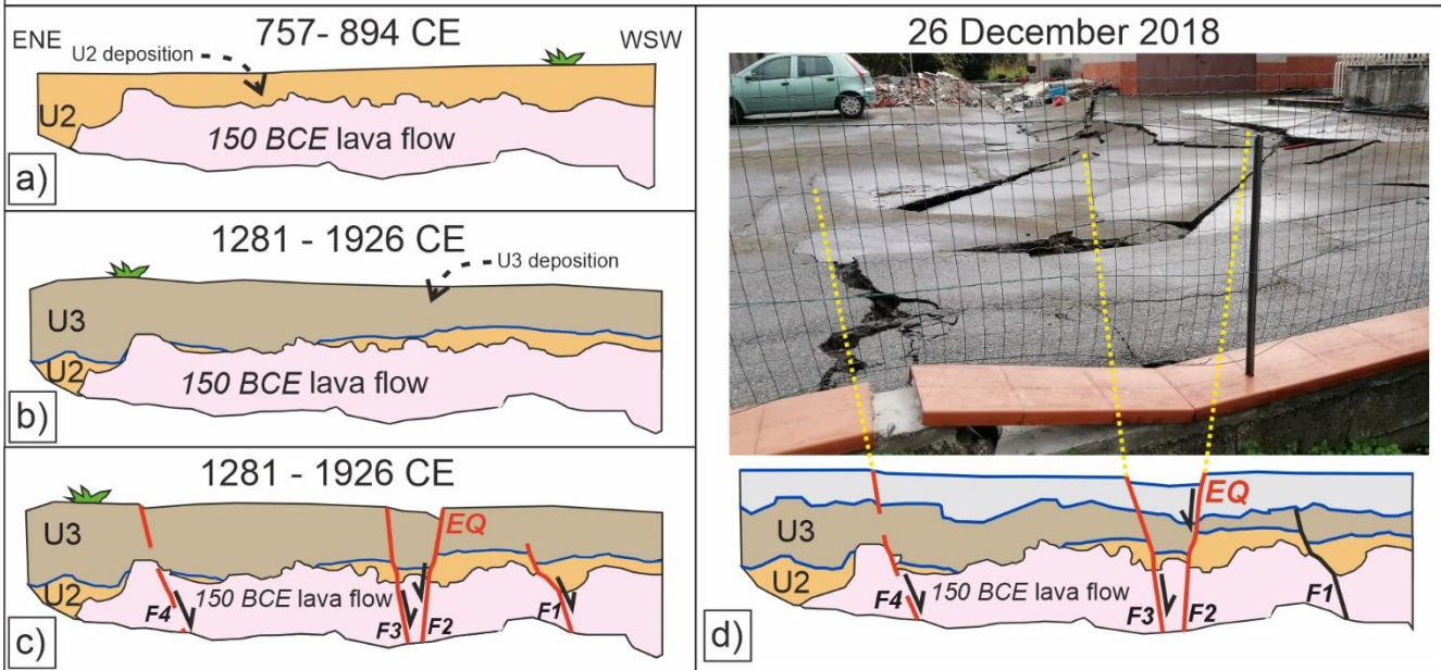
Figure 10: Possible restoration of the FIA1 S-Wall2; a) deposition of the colluvial deposit of U2 during the period 757-894 AD, subsequently partially eroded and reworked because of its exposure to the surface; b) period 1281-1926 AD with the deposition of the colluvial deposit of U3 followed by an earthquake (c) which activated F1, F2, F3 and presumably F4; d) after the reworking of the surface by the human activity and formation of the R1 during the 1970s, a second earthquake in 2018 produced a new surface faulting event along F2 and probably F3 and F4.
