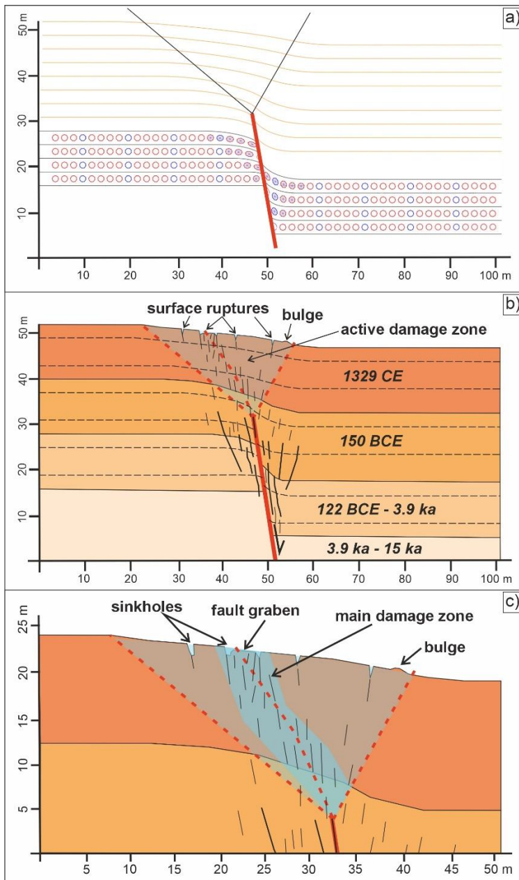
Figure 13: Results of the kinematic model (a) and proposed conceptual interpretation (b and c). The fault starts its propagation toward the surface with the formation of a monocline flexure, the process continues after the resurfacing event (yellow layers); b) interpretative model with layers associated to lava flows and their relative damage zone with the formation of dilatant fractures propagating upwards; c) zoom on the damage zone highlighting a main deformation zone with the formation of fault graben at surface with associated secondary surface ruptures, sinkholes and/or reverse features in the sides.
