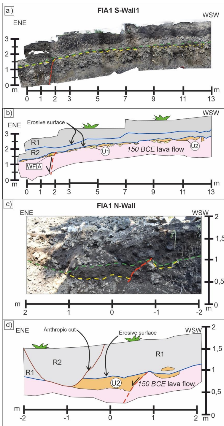
285 Figure 7: Orthophoto mosaic of the FIA1 S-Wall1 (a) and N-Wall (c): the yellow dashed line is the top of the lava flow, the green dashed line is an erosive surface interesting the tops of U2 and the lava flow, the inferred fault planes are shown in red. b) and (d) reconstruction of the stratigraphic succession along the FIA1 S-Wall1 and N-Wall (mirror); the inferred fault planes in red displace the lava flow and U2. Yellow dot is the sample collected for chemical analysis; the erosive surfaces are in blue.
