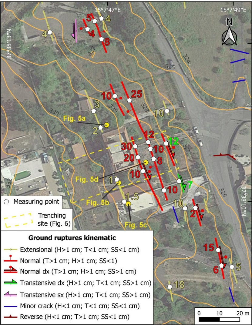
175 Figure 4: December 26, 2018, earthquake ground ruptures map around the trenching site (modified after Tringali et al., 2023a); numbers show the amount of heave (H, in yellow), throw (T, in red) and strike-slip (SS, in green); yellow dots are field photos location of Fig. 5; satellite image from Orthophoto by Regione Siciliana dataset (see data availability section).
