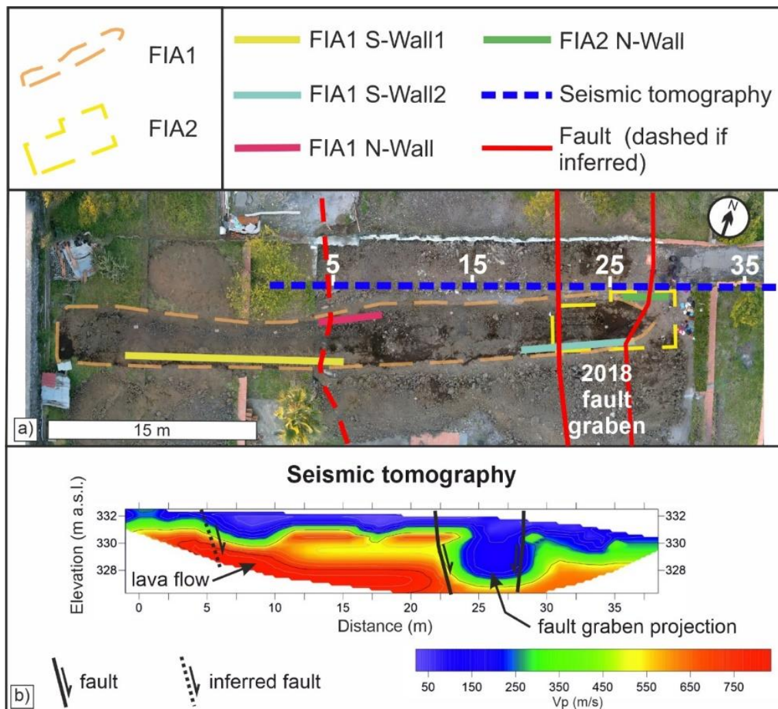
245 Figure 6: Map of Fiandaca trench site: a) orthophoto mosaic obtained by aerial drone photos showing FIA1 and FIA2 with sectors of the walls investigated in detail, and faults in accordance with the 2018 coseismic ruptures; dashed blue line is the trace of seismic tomography showed in (b).
