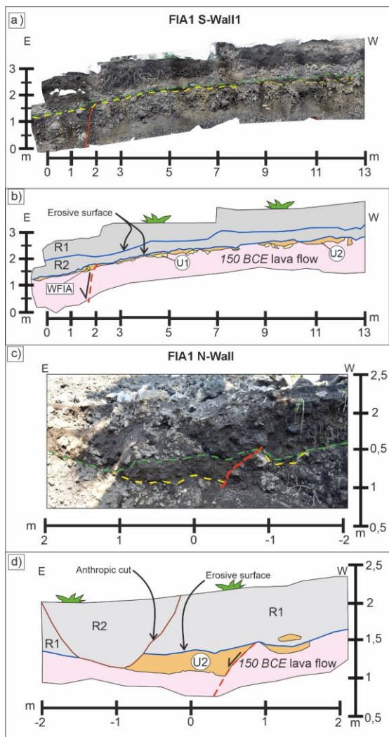
Figure 7: Orthophoto mosaic of the FIA1 S-Wall1 (a) and N-Wall (c): the yellow dashed line is the top of the lava flow, the green dashed line is an erosive surface intersecting the tops of U2 and the lava flow, the inferred fault planes are shown in red. b) and d) reconstruction of the stratigraphic succession along the FIA1 S-Wall1 and N-Wall (mirror); the inferred fault planes in red displace the lava flow and U2. Yellow dot is the sample collected for chemical analysis; the erosive surfaces are in blue.
