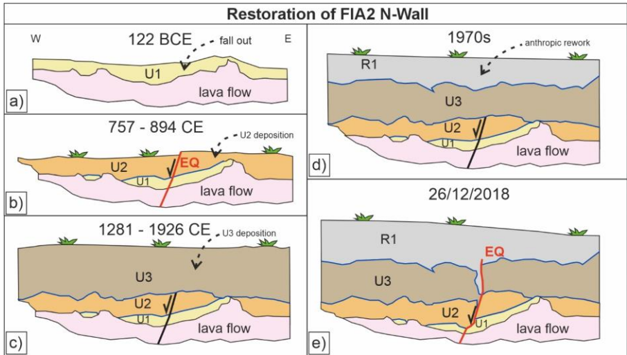
Figure 11: Possible restoration of the FIA2 N-Wall. a) pyroclastic fallout (122 BC Plinian eruption) is deposited on the 150±200 BC lava flow, subsequently partially eroded and reworked because of its exposure to the surface; b) an earthquake occurred during the deposition of the colluvial deposit of U2 in the period 757-894 AD; c) after an erosive event on U2, the deposition of the colluvial deposit of U3 occurred in the period 1281-1926 AD; d) reworking of the surface by the human activity and formation of the R1 during the 1970s; e) earthquake in 2018 displacing the lava flow, U1, U2, U3 and R1.
