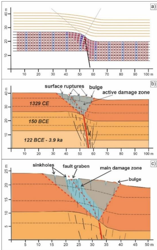
Figure 13: Results of the kinematic model (a) and proposed conceptual interpretation (b and c). The fault starts its propagation toward the surface with the formation of a monocline flexure, the process continues after the resurfacing event (yellow layers); (b) interpretative model with layers associated to lava flows and their relative damage zone with the formation of dilatant fractures propagating upwards; (c) zoom on the damage zone highlighting a main deformation zone with the formation of fault graben at surface with associated secondary surface ruptures, sinkholes and/or reverse features in the sides.
