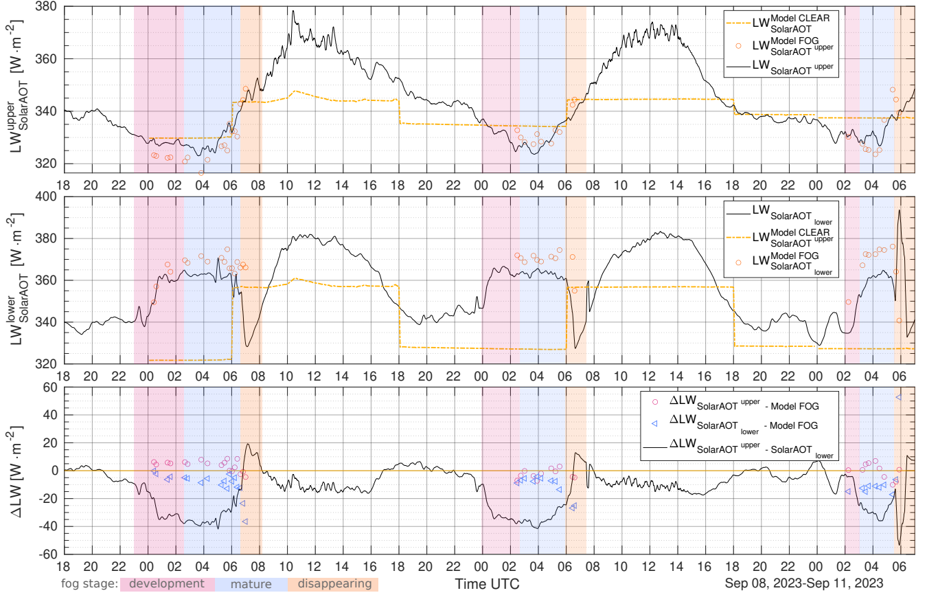
Figure 14. Incoming LW flux for SolarAOT^{upper} (upper panel) and SolarAOT^{lower} station (middle panel). The black solid line measured data, the yellow dashed line - model result for no fog conditions, the orange circles - model results for fog conditions measured by soundings. Lower panel presents with solid line difference in LW flux between SolarAOT^{upper} and SolarAOT^{lower} station, pink circles represent difference between upper station and model with fog conditions implemented and blue triangles represent difference between lower station and model with fog conditions.
