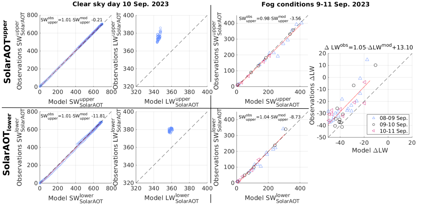
Figure 12. Scatter plots comparing observed and modeled SW (first and third column from left) and LW fluxes under clear-sky (left two columns) and fog conditions (right two columns). The last column presents the difference ( \Delta ) between upper and lower station measurements for observed and modeled LW flux in fog conditions. The red solid line indicates the linear fit to the data. Blue triangles represent measurements from the night of 8–9 Sep., black circles show fog data from the night of 9–10 Sep., and pink triangles correspond to data collected during the night of 10–11 Sep. 2023. The equation for each fit is shown in the corresponding panel.
