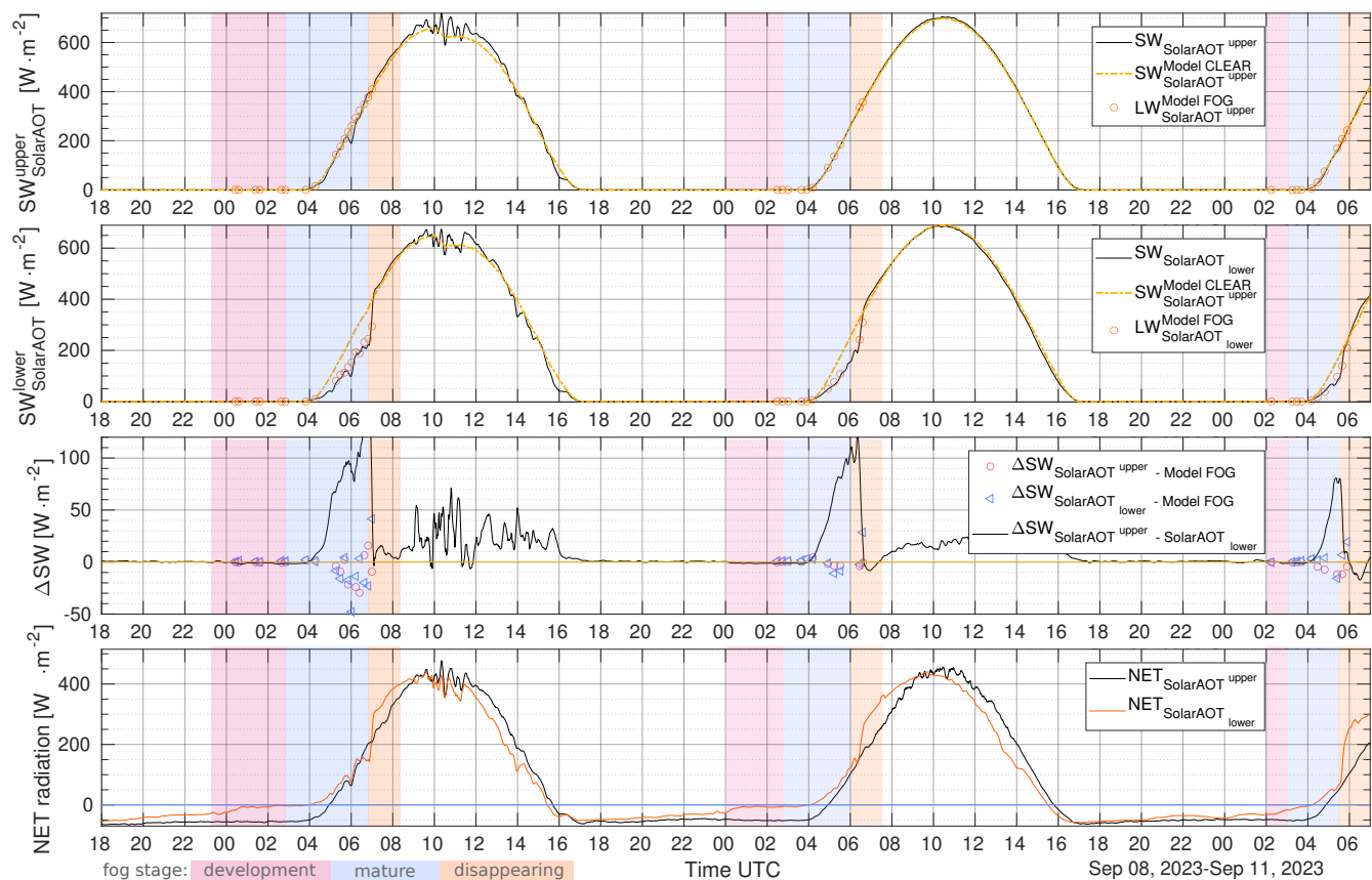
Figure 13. Incoming SW flux for SolarAOT upper and SolarAOT lower station. The black solid line measured data, the yellow dashed line - model results for no fog conditions, the orange circles - model results for fog conditions measured by soundings. The third panel from the top presents the difference in SW flux between the upper and lower site (solid line), pink circles represent the difference between SolarAOT upper station and model when fog conditions were implemented. Blue triangles represent the difference between the SolarAOT lower station and the model with implemented fog conditions. The lowest panel presents the total net radiation for SolarAOT upper (black line) and SolarAOT lower station (orange line).
