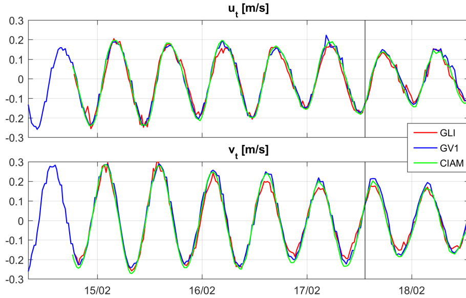
Figure 8. Depth-averaged current components computed from Equation 2, for the glider-AD2CP (GLI) and moored-ADCPs (CIAM, GV1). The vertical black line delineates the BU and VM survey periods.
