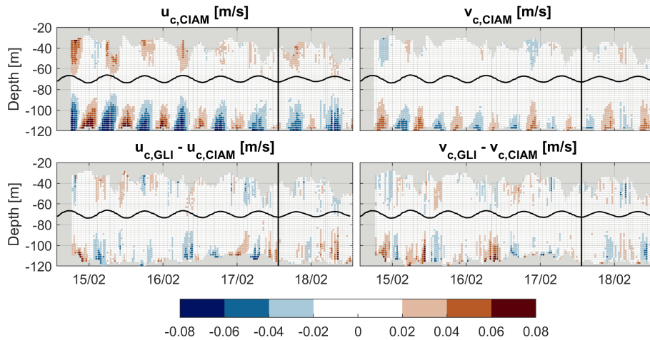
Figure 9. Up) Components of the residual currents (deviation from the depth-averaged purely barotropic constant) measured by the CIAM moored-ADCP. Down) Components of the difference between the residual currents measured by the glider-AD2CP and CIAM moored-ADCP. Residual currents are defined as u(z, t) - \bar{u}(t) , where \bar{u}(t) is the depth-averaged strictly barotropic velocity computed from Equation 2. The black undulated line represents the free surface variation with tide (put in the middle of the graphic for a better display), computed from the GV1 pressure sensor. The black straight line delineates the BU and VM survey periods.
