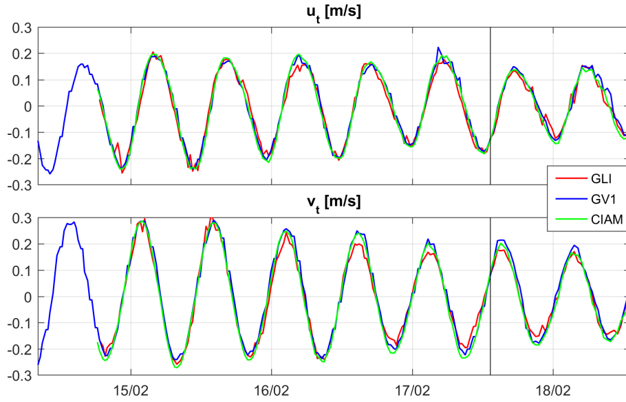
Figure 8. Depth-averaged Barotropic current components computed from Equation 2, for the glider-AD2CP (GLI) and moored-ADCPs (CIAM, GV1). The vertical black line delineates the BU and VM survey periods.
