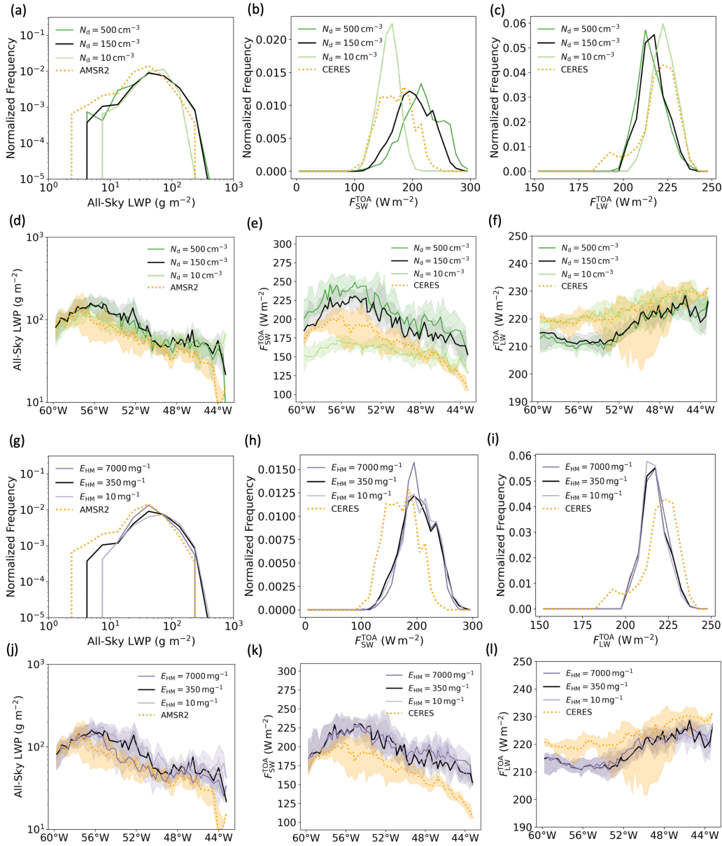
Figure J2. Model output compared with satellite retrievals for simulations with different N_d (a-f) and E_{\text{HM}} (g-l) on 24 October 2022: the normalized frequency of all-sky liquid water path (LWP) from AMSR-2 (left column), shortwave radiation at the top-of-atmosphere (middle column) and longwave radiation at the top-of-atmosphere from CERES (right column).
