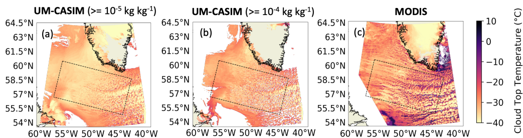
Figure D1. Cloud top temperature (CTT, a-c) from the control simulation of the March case and the MODIS onboard Aqua satellite. Two TWC (total water content) thresholds were used to determine whether a model grid is cloudy or not which are \text{TWC} \geq 10^{-5} \text{ kg kg}^{-1} (a) and \text{TWC} \geq 10^{-4} \text{ kg kg}^{-1} (b). Regions marked with grey dashed lines in (a) - (c) are the sub-domains (same as the sub-domains shown in the main content) for the comparison of CTT distributions in Figure D2.
