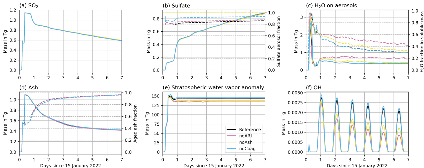
Figure 2. Same as Fig. 1, but for the experiments Reference, noARI, noCoag, and noAsh. Note that the curves in a), b), and d) are overlapping.
