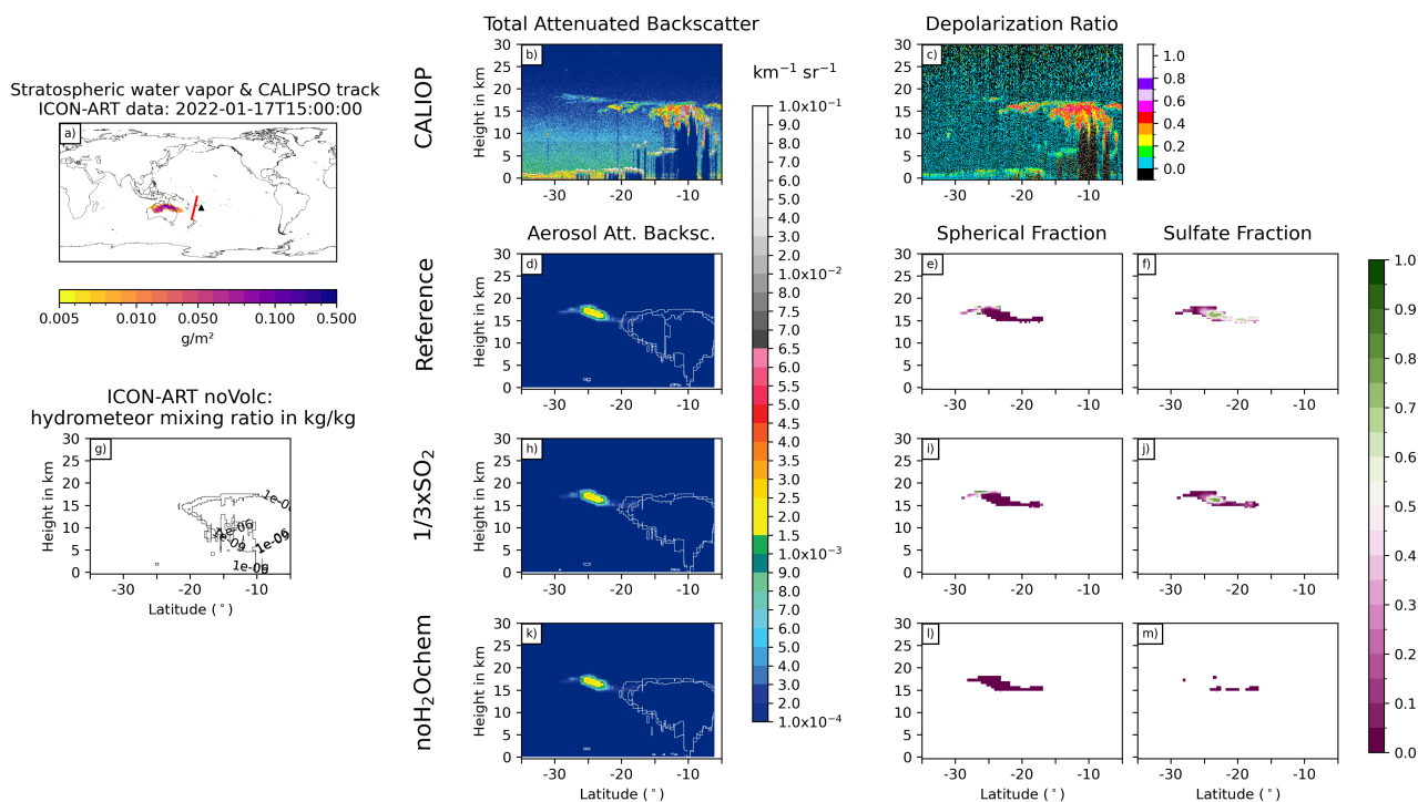
Figure 7. As Fig. 6, but for 17 January, 2022 at 15:00 UTC
