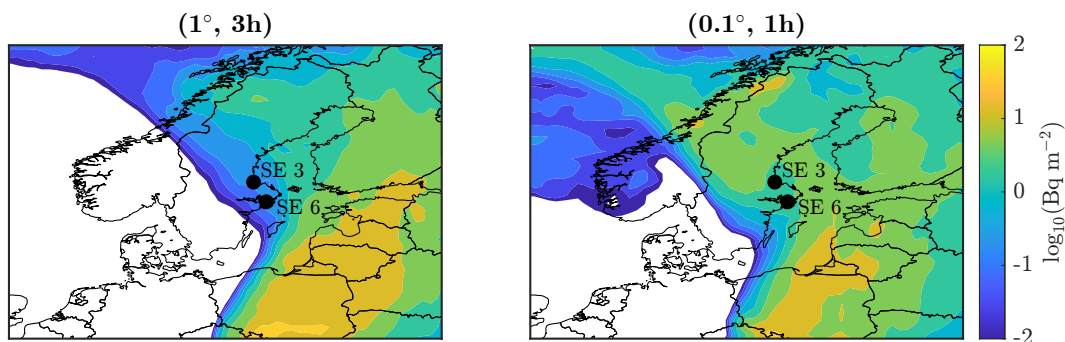
Figure 7. Total deposition using meteorological data with a spatiotemporal resolution of ( 1^\circ , 3 h) and ( 0.1^\circ , 1 h). The location of the Sweden 3 and 6 measurements are marked by the black circles.
