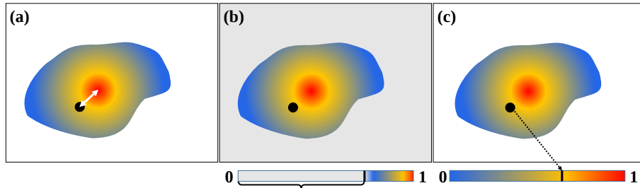
Figure 3. Schematic illustration of the three performance metrics as introduced by De Meutter et al. (2024) and adapted therefrom with a license agreement. (a) distance-Distance (b) fraction of the domain excluded (FDE) and (c) cumulative distribution score (CDS). The black bullet represents the true source location and the coloured fields represent the source location probabilities.
