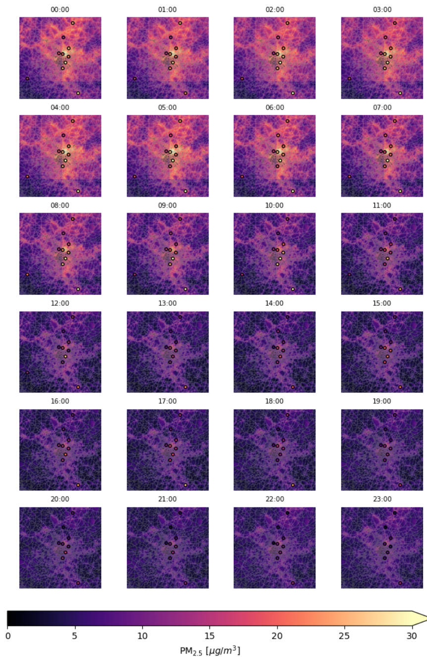
Figure 7. PM 2.5 map on 06.12.2019. The dots reprent PM 2.5 measurements from OpenAQ ground stations.
