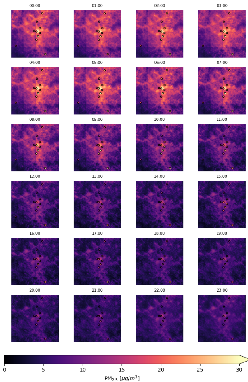
Figure 6. PM 2.5 map on 06.12.2019. The dots represent PM 2.5 measurements from OpenAQ ground stations.
