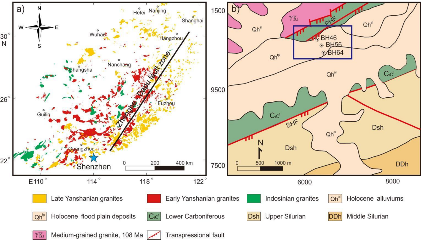
Figure 1: Regional (a) and local (b) geological map of the Pingshan district, Shenzhen (after Mao, 2014 and Shenzhen Geology, 2009). Blue rectangle (Fig. 3a) shows study area location.
