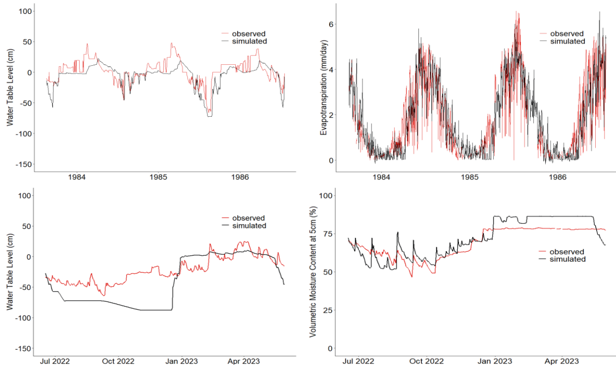
Figures showing the performance of simulated hydrological variables relative to measurements for Water Table Level (upper and lower left), Evapotranspiration (upper right) and VMC at 5cm (lower right). Calibration period is from August 1983- July 1987, while validation period is from June, 2022 to May, 2023
