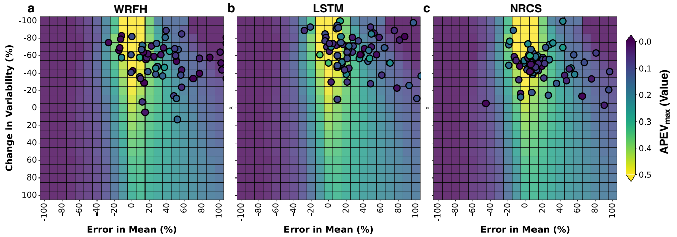
Figure 11: Comparison of value between synthetic and true forecast systems to the error in mean and change in variability. Area under PEV max curve (APEV max ) of three forecast systems (WRFH, LSTM, and NRCS) represented as scatter points (each point represents a basin), indicating the true value during drought years between WY 2006 and 2022. The background heatmaps represent the sensitivity of APEV max to error in mean and change in variability for synthetic forecasts. RMAD for true forecast systems from the optimal scenario are 100%, 81%, and 91% for WRFH, LSTM, and NRCS, respectively.
