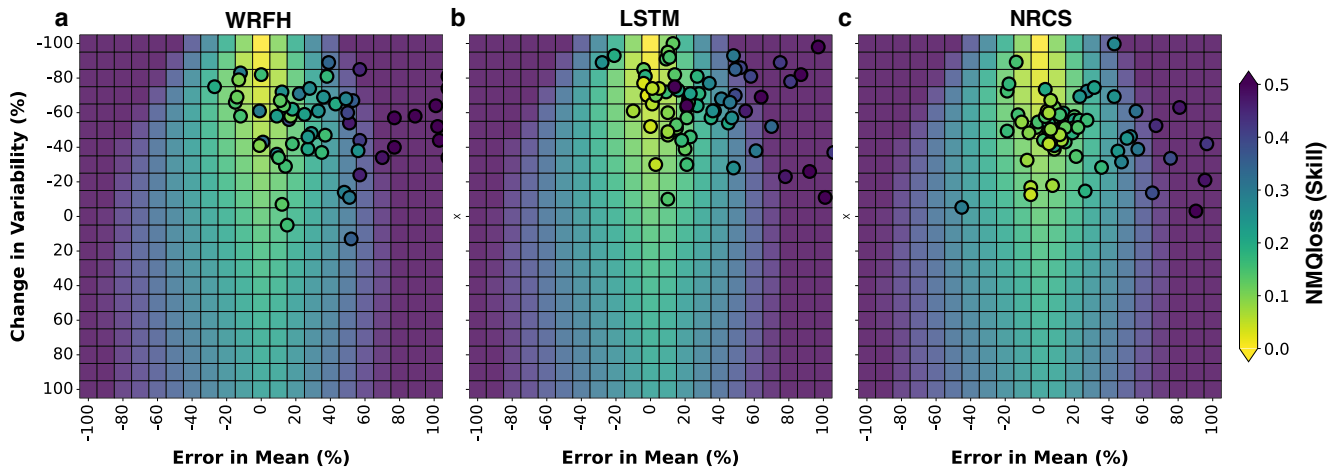
Figure 10: Comparison of skill between synthetic and true forecast systems to error in mean and change in variability. Normalized mean quantile loss (NMQloss) of three forecast systems (WRFH, LSTM, and NRCS) represented as scatter points (each point represents a basin), indicating the true skill during drought years between WY 2006 and 2022. The background heatmaps represent the sensitivity of skill to error in mean and change in variability for synthetic forecasts. RMAD for true forecast systems from the optimal scenario are 30%, 23%, and 20% for WRFH, LSTM, and NRCS, respectively.
