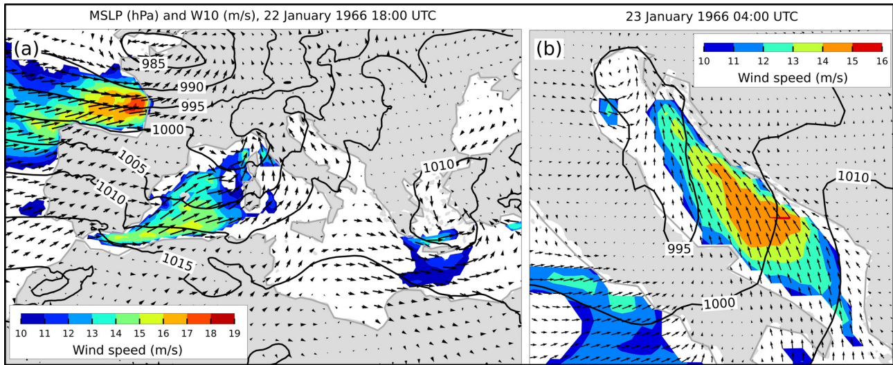
465 Figure 10: MSLP (black lines) and W10 (arrows and colours) fields from the ERA5 reanalysis. Conditions (a) over the Mediterranean that preceded the situation (b) over the Adriatic Sea (an hour before maximum SL in Bakar). Only wind speeds exceeding 10 m/s are coloured.
