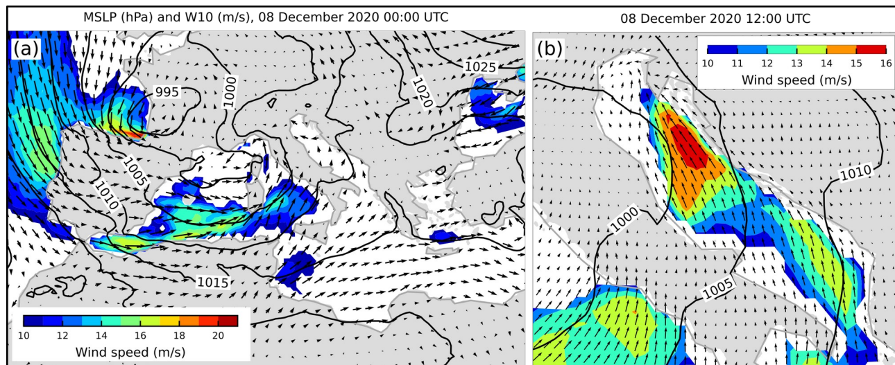
Figure 64: MSLP (black lines) and W10 (arrows and colours) fields from the ERA5 reanalysis. Conditions (a) over the Mediterranean and western Europe that preceded the situation (b) over the Adriatic Sea (an hour before maximum SL in Bakar). Only wind speeds exceeding 10 m/s are coloured.
