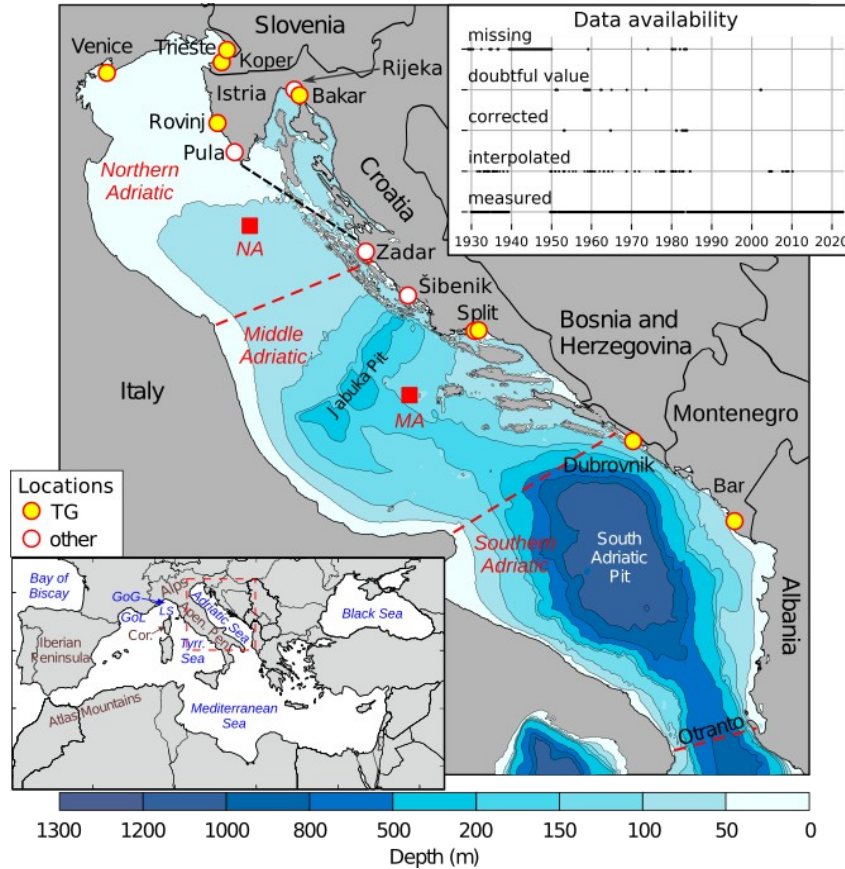
70 Figure 1: Bathymetry of the Adriatic Sea. Locations of tide-gauge stations with records of at least 60 y (Pérez Gómez et al., 2022) are marked with red-yellow circles. Other major towns along the Croatian Adriatic coast are marked with red-white circles. The subdivision of the Adriatic into sub-basins is marked with red dashed lines and the area of the Kvarner Bay is to the northeast of the black dashed line. The red rectangles mark grid points for which the atmospheric reanalysis series were analysed. The position of the Adriatic in relation to the Mediterranean is shown in the small inset in the lower left corner, and the data availability of TG Bakar time series is shown in the upper right corner. On the Mediterranean map, frequently referenced regions are labelled: Gulf of Genoa (GoG), Gulf of Lion (GoL), Ligurian Sea (LS), Tyrrhenian Sea (Tyrr. Sea), Apennine Peninsula (Apenn. Pen.) and Corsica (Cor.).
