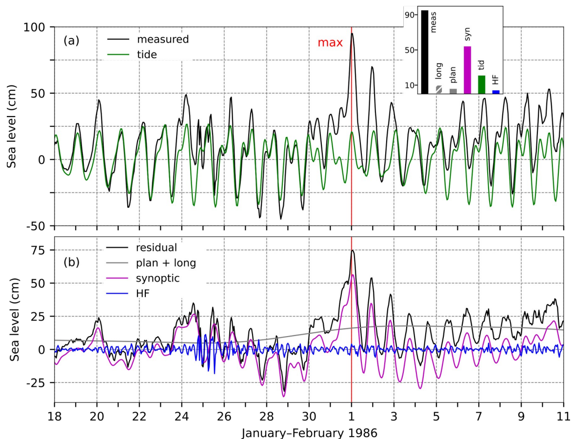
945 Figure 29: SL series for the flood of 1 February 1986. (a) Measured sea level (black) and tide (green). The inset figure shows the contributions (cm) of the five sea-level components to the maximum measured sea level ("meas"; 00:00 UTC): "HF" refers to high-frequency oscillations ( 2 \text{ h} < T < 9 \text{ h} ), "syn" to synoptic component ( 9 \text{ h} < T < 10 \text{ d} ), "tid" to tide , "plan" to planetary-scale variability ( 10 \text{ d} < T < 100 \text{ d} ), "long" to long-term sea-level variability ( 100 \text{ d} < T ). (b) Residual sea level (black), the combined series of planetary-scale variability and long-term sea-level variability (grey; plan + long), synoptic component (purple), and high-frequency oscillations (blue). 950 The red line indicates the time of occurrence of the total SL maximum.
