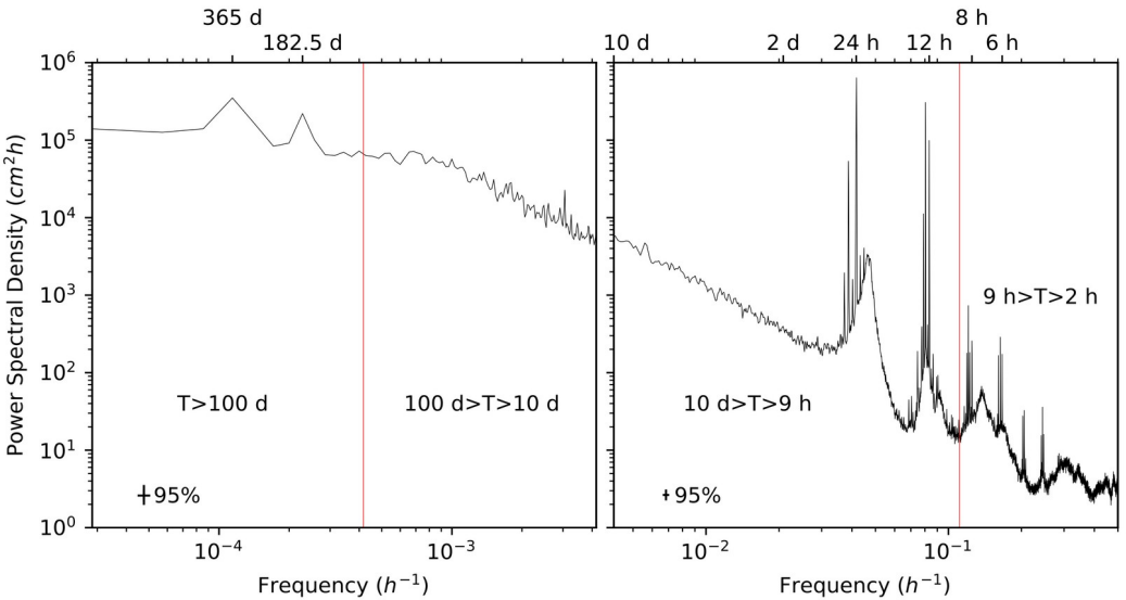
Figure 2: Power spectral densities of total SL measured at TG Bakar (1950–2022), shown for periods longer than 10 d (left) and shorter than 10 d (right). Spectra were computed using Hamming windows with 50% overlap: 4 y windows for the left panel and 1 y windows for the right. Red vertical lines indicate a period of 100 d (left) and 9 h (right). The 95% confidence intervals are indicated. Vertical lines (red and subplot edges) mark boundaries between different sea-level processes.
