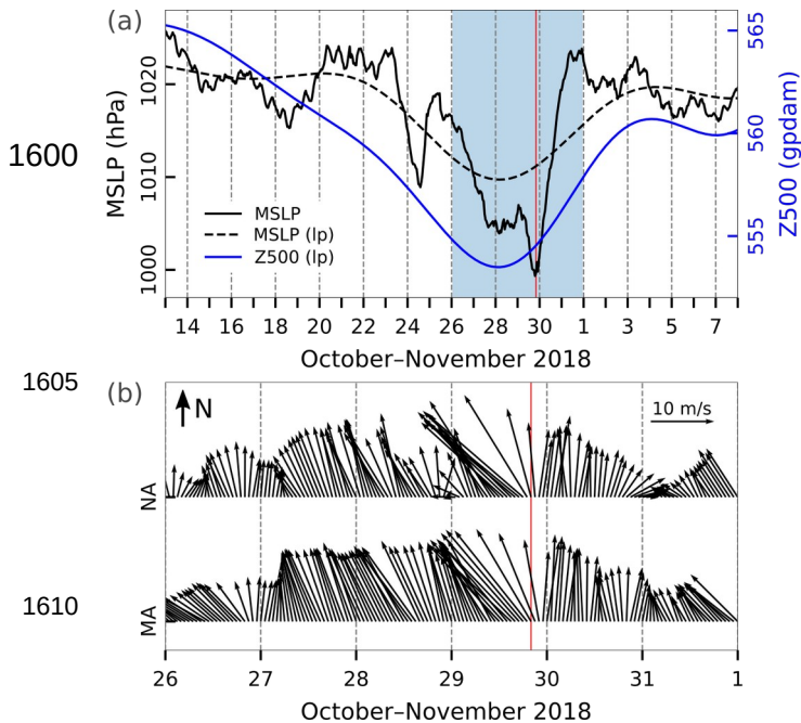
Figure 54: Series of ERA5 reanalysis data related to the flood of 29 October 2018. (a) MSLP (hourly) and MSLP (lp) (low-pass filtered with a cut-off frequency of 10 d) and Z500 (lp) (low-pass filtered with a cut-off frequency of 10 d) at a grid point near TG Bakar. (b) Hourly W10 during the period marked in blue in the upper plot for the middle (MA) and northern (NA) Adriatic (all locations marked in Fig. 1). The red line indicates onset of SL maximum.
