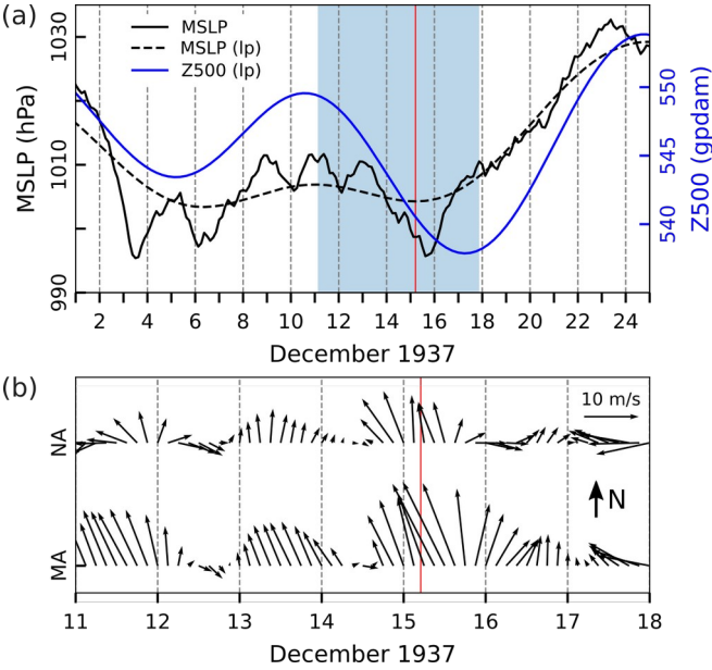
Figure 3: Series of NOAA-CIRES-DOE reanalysis data related to the flood of 15 December 1937. (a) MSLP (every 3 h) and MSLP (lp) (low-pass filtered with a cut-off frequency of 10 d) and Z500 (lp) (low-pass filtered with a cut-off frequency of 10 d) at a grid point near TG Bakar. (b) W10 (every 3 h) during the period marked in blue in the upper plot for the middle (MA) and northern (NA) Adriatic (all locations marked in Fig. 1). The red line indicates onset of SL maximum.
