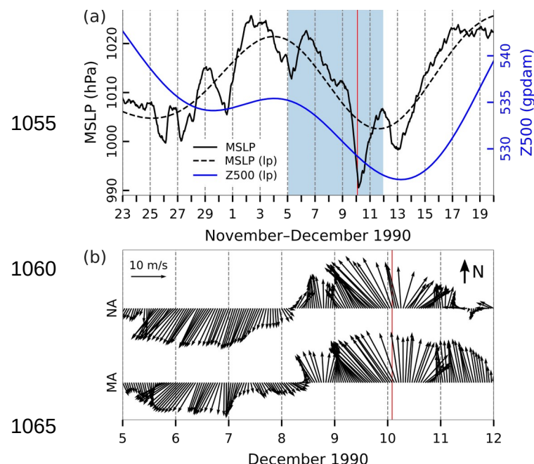
Figure 33: Series of ERA5 reanalysis data related to the flood of 10 December 1990. (a) MSLP (hourly) and MSLP (lp) (low-pass filtered with a cut-off frequency of 10 d) and Z500 (lp) (low-pass filtered with a cut-off frequency of 10 d) at a grid point near TG Bakar. (b) Hourly W10 during the period marked in blue in the upper plot for the middle (MA) and northern (NA) Adriatic (all locations marked in Fig. 1). The red line indicates onset of SL maximum.
