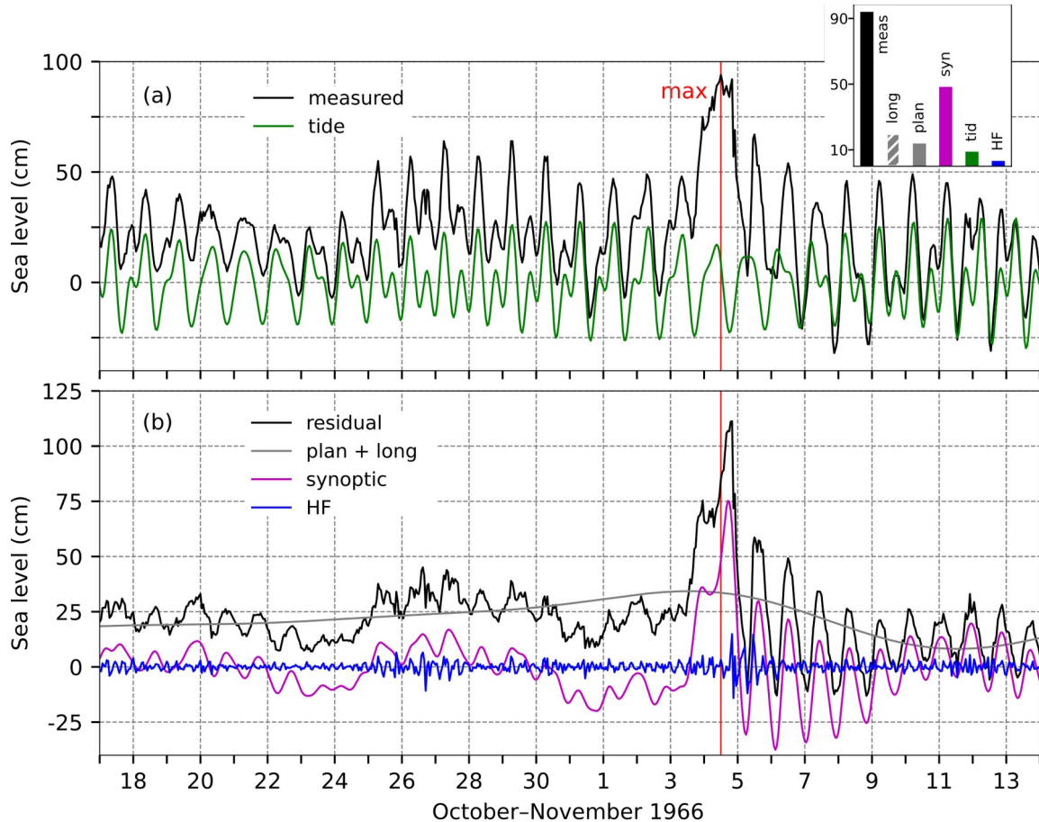
Figure 14: SL series for the flood of 4 November 1966. (a) Measured sea level (black) and tide (green). The inset figure shows the contributions (cm) of the five sea-level components to the maximum measured sea level ("meas"; 12:00 UTC): "HF" refers to high-frequency oscillations ( 2\text{ h} < T < 9\text{ h} ), "syn" to synoptic component ( 9\text{ h} < T < 10\text{ d} ), "tid" to tide , "plan" to planetary-scale variability ( 10\text{ d} < T < 100\text{ d} ), "long" to long-term sea-level variability ( 100\text{ d} < T ). (b) Residual sea level (black), the combined series of planetary-scale variability and long-term sea-level variability (grey; plan + long), synoptic component (purple), and high-frequency oscillations (blue). The red line indicates the time of occurrence of the total SL maximum.
