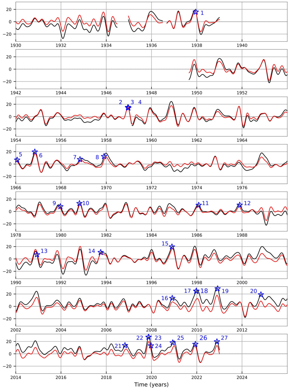
Figure A1: Long-term sea-level variability (black; cm), representing SL changes at periods longer than 100 d. Intraannual variability
