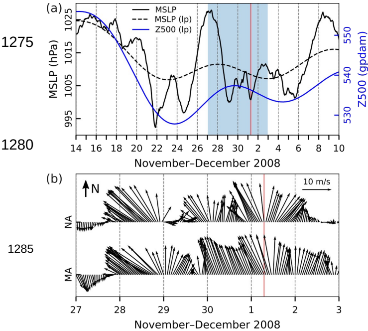
Figure 42: Series of ERA5 reanalysis data related to the flood of 1 December 2008. (a) MSLP (hourly) and MSLP (lp) (low-pass filtered with a cut-off frequency of 10 d) and Z500 (lp) (low-pass filtered with a cut-off frequency of 10 d) at a grid point near TG Bakar. (b) Hourly W10 during the period marked in blue in the upper plot for the middle (MA) and northern (NA) Adriatic (all locations marked in Fig. 1). The red line indicates onset of SL maximum.
