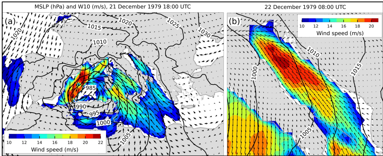
775 Figure 22: MSLP (black lines) and W10 (arrows and colours) fields from the ERA5 reanalysis. Conditions (a) over the Mediterranean that preceded the situation (b) over the Adriatic Sea (an hour before maximum SL in Bakar). Only wind speeds exceeding 10 m/s are coloured.
