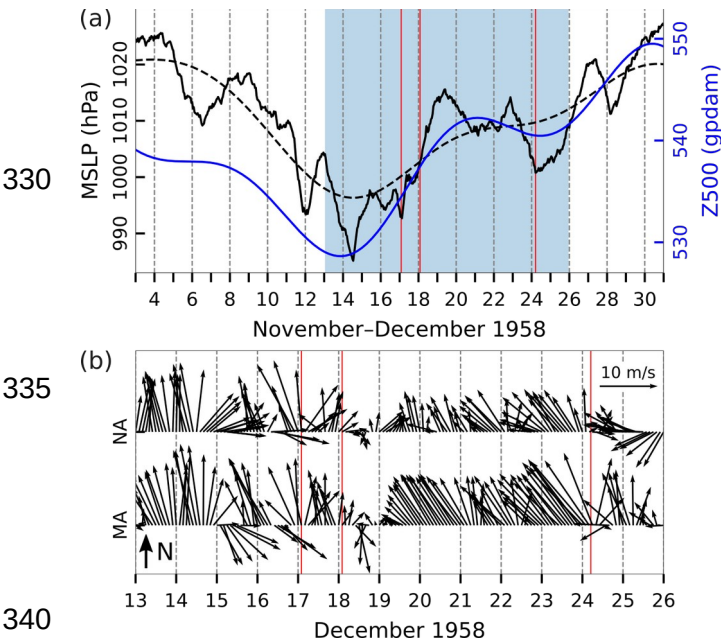
Figure 6: Series of ERA5 reanalysis data related to the floods of 17, 18 and 24 December 1958. (a) MSLP (hourly) and MSLP (lp) (low-pass filtered with a cut-off frequency of 10 d) and Z500 (lp) (low-pass filtered with a cut-off frequency of 10 d) at a grid point near TG Bakar. (b) Hourly W10 during the period marked in blue in the upper plot for the middle (MA) and northern (NA) Adriatic (all locations marked in Fig. 1). Every second value is plotted. The red lines indicate onset of SL maxima.
