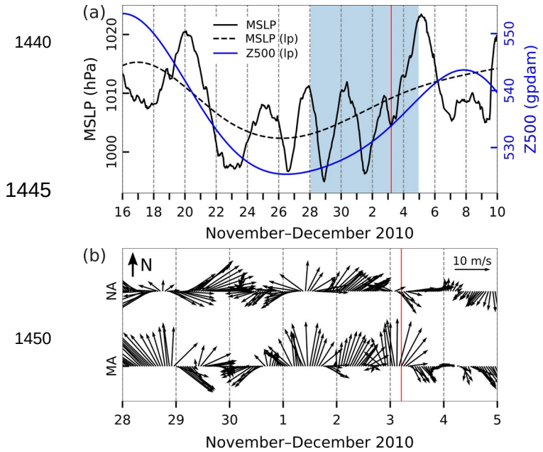
Figure 48: Series of ERA5 reanalysis data related to the flood of 3 December 2010. (a) MSLP (hourly) and MSLP (lp) (low-pass filtered with a cut-off frequency of 10 d) and Z500 (lp) (low-pass filtered with a cut-off frequency of 10 d) at a grid point near TG Bakar. (b) Hourly W10 during the period marked in blue in the upper plot for the middle (MA) and northern (NA) Adriatic (all locations marked in Fig. 1). The red line indicates onset of SL maximum.
