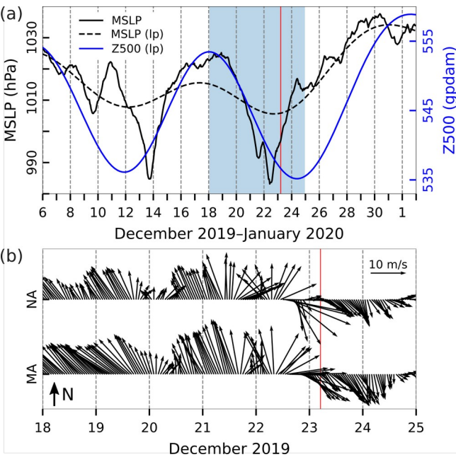
Figure 60: Series of ERA5 reanalysis data related to the flood of 23 December 2019. (a) MSLP (hourly) and MSLP (lp) (low-pass filtered with a cut-off frequency of 10 d) and Z500 (lp) (low-pass filtered with a cut-off frequency of 10 d) at a grid point near TG Bakar. (b) Hourly W10 during the period marked in blue in the upper plot for the middle (MA) and northern (NA) Adriatic (all locations marked in Fig. 1). The red line indicates onset of SL maximum.
