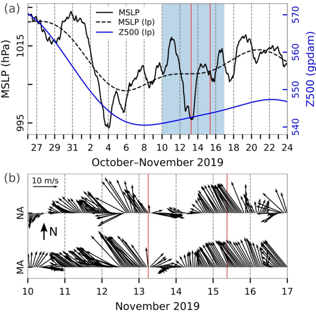
Figure 57: Series of ERA5 reanalysis data related to the floods of 13 and 15 November 2019. (a) MSLP (hourly) and MSLP (lp) (low-pass filtered with a cut-off frequency of 10 d) and Z500 (lp) (low-pass filtered with a cut-off frequency of 10 d) at a grid point near TG Bakar. (b) Hourly W10 during the period marked in blue in the upper plot for the middle (MA) and northern (NA) Adriatic (all locations marked in Fig. 1). The red lines indicate onset of SL maxima.
