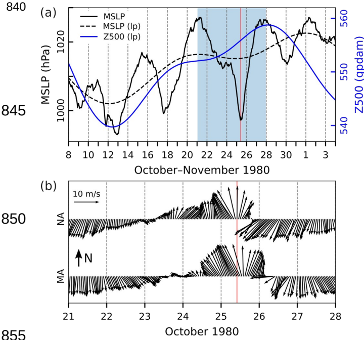
Figure 24: Series of ERA5 reanalysis data related to the flood of 25 October 1980. (a) MSLP (hourly) and MSLP (lp) (low-pass filtered with a cut-off frequency of 10 d) and Z500 (lp) (low-pass filtered with a cut-off frequency of 10 d) at a grid point near TG Bakar. (b) Hourly W10 during the period marked in blue in the upper plot for the middle (MA) and northern (NA) Adriatic (all locations marked in Fig. 1). The red line indicates onset of SL maximum.
