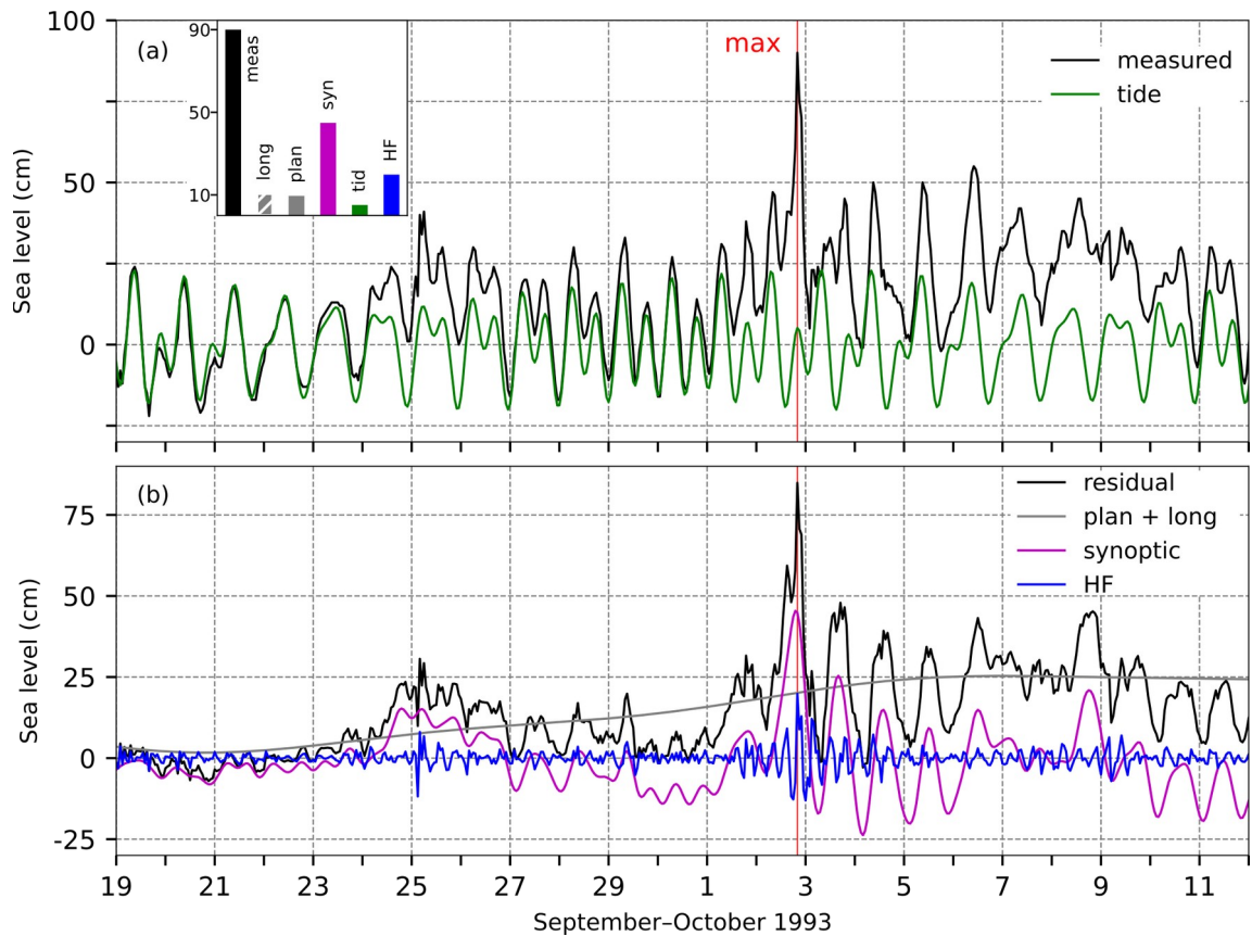
1195 Figure 38: SL series for the flood of 2 October 1993. (a) Measured sea level (black) and tide (green). The inset figure shows the contributions (cm) of the five sea-level components to the maximum measured sea level ("meas"; 20:00 UTC): "HF" refers to high-frequency oscillations (2 h < T < 9 h), "syn" to synoptic component (9 h < T < 10 d), "tid" to tide , "plan" to planetary-scale variability (10 d < T < 100 d), "long" to long-term sea-level variability (100 d < T). (b) Residual sea level (black), the combined series of planetary-scale variability and long-term sea-level variability (grey; plan + long), synoptic component (purple), and high-frequency oscillations (blue). 1200 The red line indicates the time of occurrence of the total SL maximum.
