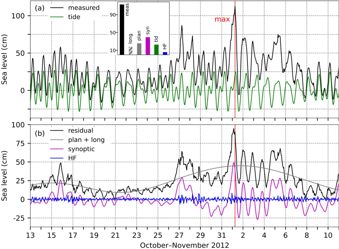
Figure 53: SL series for the flood of 1 November 2012. (a) Measured sea level (black) and tide (green). The inset figure shows the contributions (cm) of the five sea-level components to the maximum measured sea level ("meas"; 06:00 UTC): "HF" refers to high-frequency oscillations ( 2 \text{ h} < T < 9 \text{ h} ), "syn" to synoptic component ( 9 \text{ h} < T < 10 \text{ d} ), "tid" to tide , "plan" to planetary-scale variability ( 10 \text{ d} < T < 100 \text{ d} ), "long" to long-term sea-level variability ( 100 \text{ d} < T ). (b) Residual sea level (black), the combined series of planetary-scale variability and long-term sea-level variability (grey; plan + long), synoptic component (purple), and high-frequency oscillations (blue). The red line indicates the time of occurrence of the total SL maximum.
