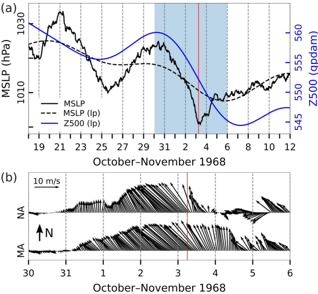
Figure 15: Series of ERA5 reanalysis data related to the flood of 3 November 1968. (a) MSLP (hourly) and MSLP (lp) (low-pass filtered with a cut-off frequency of 10 d) and Z500 (lp) (low-pass filtered with a cut-off frequency of 10 d) at a grid point near TG Bakar. (b) Hourly W10 during the period marked in blue in the upper plot for the middle (MA) and northern (NA) Adriatic (all locations marked in Fig. 1). The red line indicates onset of SL maximum.
