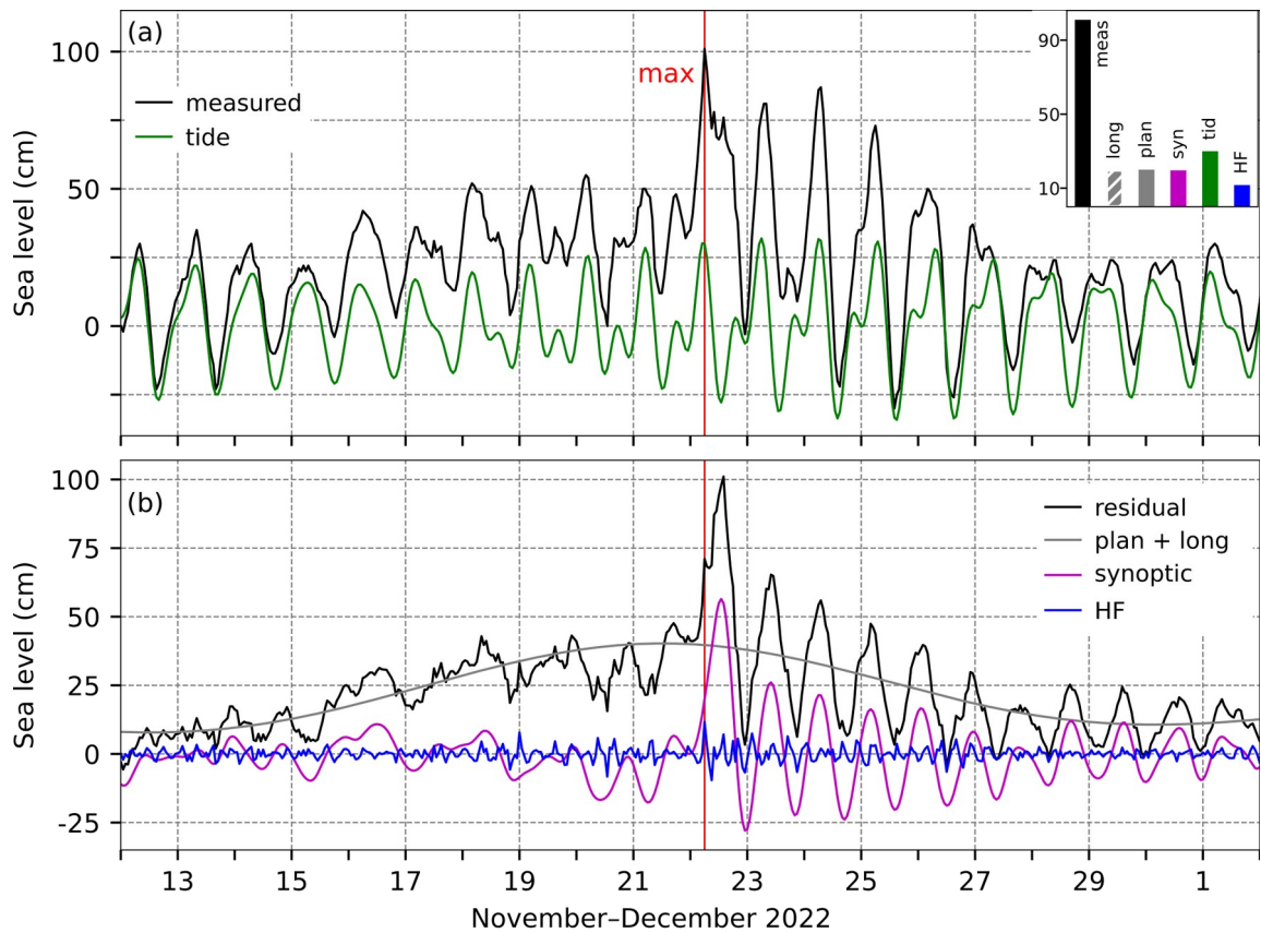
Figure 71: SL series for the flood of 22 November 2022. (a) Measured sea level (black) and tide (green). The inset figure shows the contributions (cm) of the five sea-level components to the maximum measured sea level ("meas"; 06:00 UTC): "HF" refers to high-frequency oscillations ( 2\text{ h} < T < 9\text{ h} ), "syn" to synoptic component ( 9\text{ h} < T < 10\text{ d} ), "tid" to tide , "plan" to planetary-scale variability ( 10\text{ d} < T < 100\text{ d} ), "long" to long-term sea-level variability ( 100\text{ d} < T ). (b) Residual sea level (black), the combined series of planetary-scale variability and long-term sea-level variability (grey; plan + long), synoptic component (purple), and high-frequency oscillations (blue). The red line indicates the time of occurrence of the total SL maximum.
