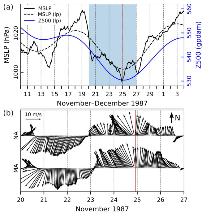
Figure 30: Series of ERA5 reanalysis data related to the flood of 24 November 1987. (a) MSLP (hourly) and MSLP (lp) (low-pass filtered with a cut-off frequency of 10 d) and Z500 (lp) (low-pass filtered with a cut-off frequency of 10 d) at a grid point near TG Bakar. (b) Hourly W10 during the period marked in blue in the upper plot for the middle (MA) and northern (NA) Adriatic (all locations marked in Fig. 1). The red line indicates onset of SL maximum.
