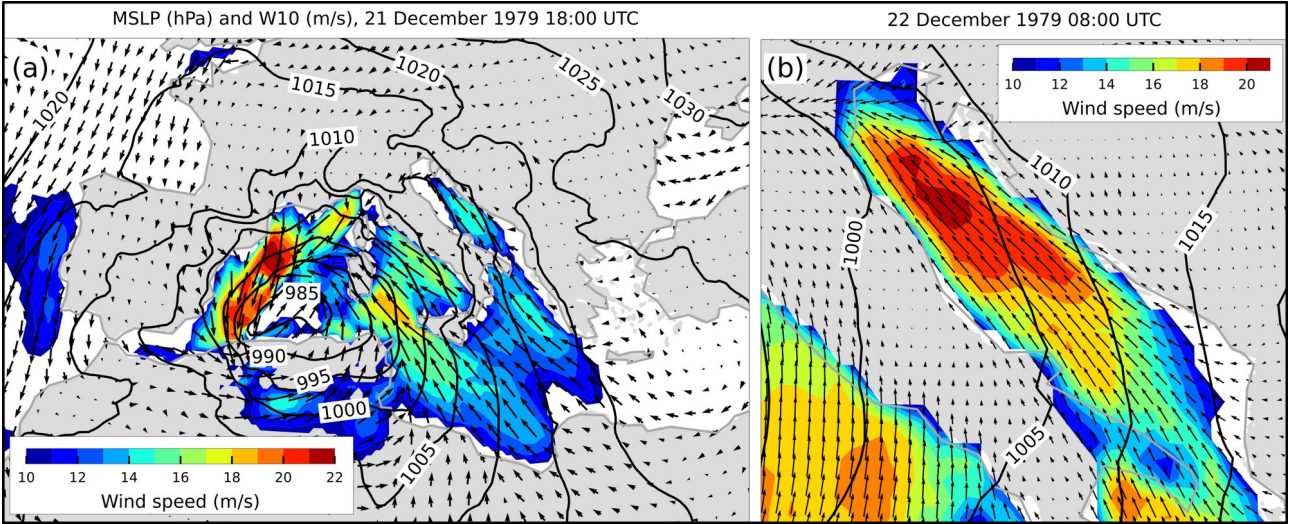
Figure 22: MSLP (black lines) and W10 (arrows and colours) fields from the ERA5 reanalysis. Conditions (a) over the Mediterranean that 795 preceded the situation (b) over the Adriatic Sea (an hour before maximum SL in Bakar). Only wind speeds exceeding 10 m/s are coloured.
