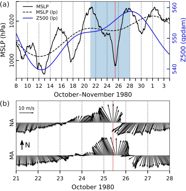
Figure 24: Series of ERA5 reanalysis data related to the flood of 25 October 1980. (a) MSLP (hourly) and MSLP (lp) (low-pass filtered with a cut-off frequency of 10 d) and Z500 (lp) (low-pass filtered with a cut-off frequency of 10 d) at a grid point near TG Bakar. (b) Hourly W10 during the period marked in blue in the upper plot for the middle (MA) and northern (NA) Adriatic (all locations marked in Fig. 1). The red line indicates onset of SL maximum.
