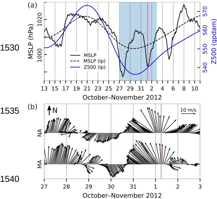
Figure 51: Series of ERA5 reanalysis data related to the flood of 1 November 2012. (a) MSLP (hourly) and MSLP (lp) (low-pass filtered with a cut-off frequency of 10 d) and Z500 (lp) (low-pass filtered with a cut-off frequency of 10 d) at a grid point near TG Bakar. (b) Hourly W10 during the period marked in blue in the upper plot for the middle (MA) and northern (NA) Adriatic (all locations marked in Fig. 1). The red line indicates onset of SL maximum.
