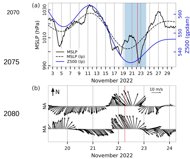
Figure 69: Series of ERA5 reanalysis data related to the flood of 22 November 2022. (a) MSLP (hourly) and MSLP (lp) (low-pass filtered with a cut-off frequency of 10 d) and Z500 (lp) (low-pass filtered with a cut-off frequency of 10 d) at a grid point near TG Bakar. (b) Hourly W10 during the period marked in blue in the upper plot for the middle (MA) and northern (NA) Adriatic (all locations marked in Fig. 1). The red line indicates onset of SL maximum.
