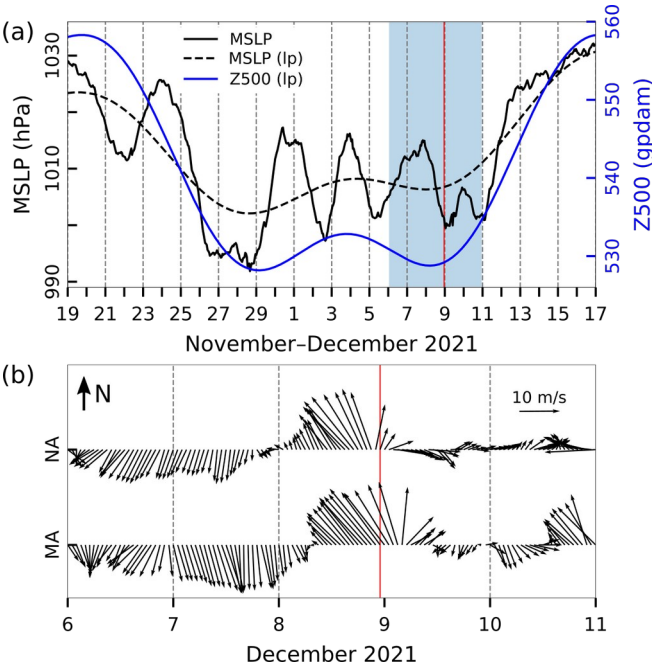
Figure 66: Series of ERA5 reanalysis data related to the flood of 8 December 2021. (a) MSLP (hourly) and MSLP (lp) (low-pass filtered with a cut-off frequency of 10 d) and Z500 (lp) (low-pass filtered with a cut-off frequency of 10 d) at a grid point near TG Bakar. (b) Hourly W10 during the period marked in blue in the upper plot for the middle (MA) and northern (NA) Adriatic (all locations marked in Fig. 1). The red line indicates onset of SL maximum.
