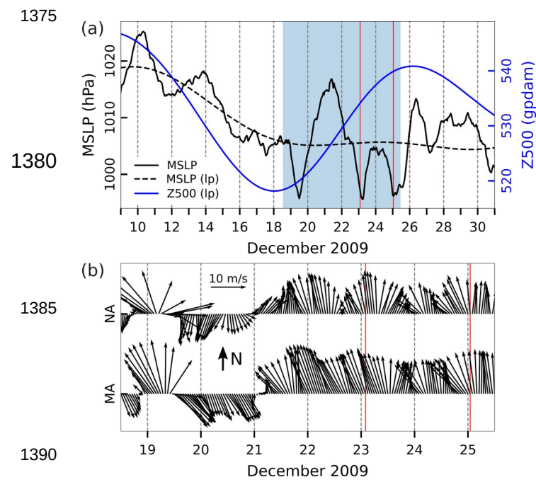
Figure 45: Series of ERA5 reanalysis data related to the floods of 23 and 25 December 2009. (a) MSLP (hourly) and MSLP (lp) (low-pass filtered with a cut-off frequency of 10 d) and Z500 (lp) (low-pass filtered with a cut-off frequency of 10 d) at a grid point near TG Bakar. (b) Hourly W10 during the period marked in blue in the upper plot for the middle (MA) and northern (NA) Adriatic (all locations marked in Fig. 1). The red lines indicate onset of SL maxima.
