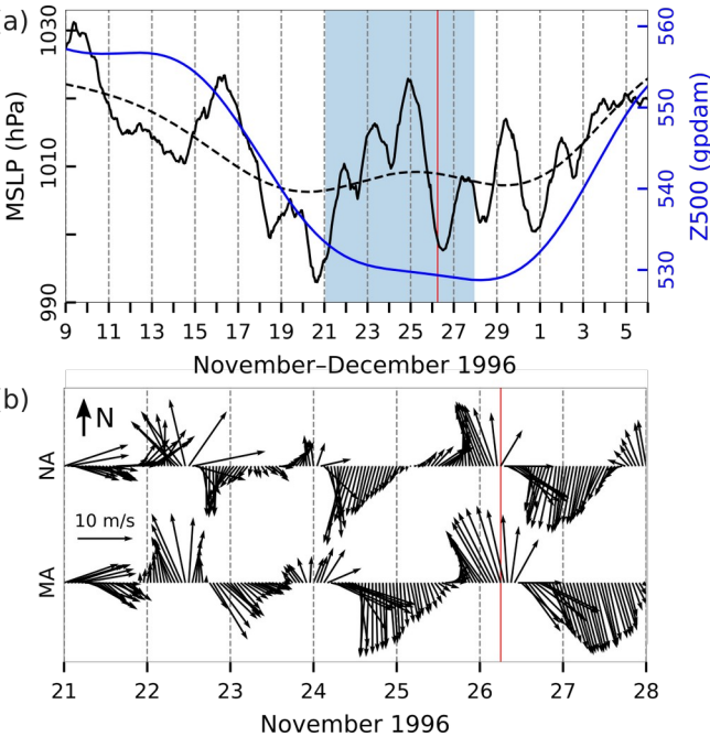
Figure 39: Series of ERA5 reanalysis data related to the flood of 26 November 1996. (a) MSLP (hourly) and MSLP (lp) (low-pass filtered with a cut-off frequency of 10 d) and Z500 (lp) (low-pass filtered with a cut-off frequency of 10 d) at a grid point near TG Bakar. (b) Hourly W10 during the period marked in blue in the upper plot for the middle (MA) and northern (NA) Adriatic (all locations marked in Fig. 1). The red line indicates onset of SL maximum.
