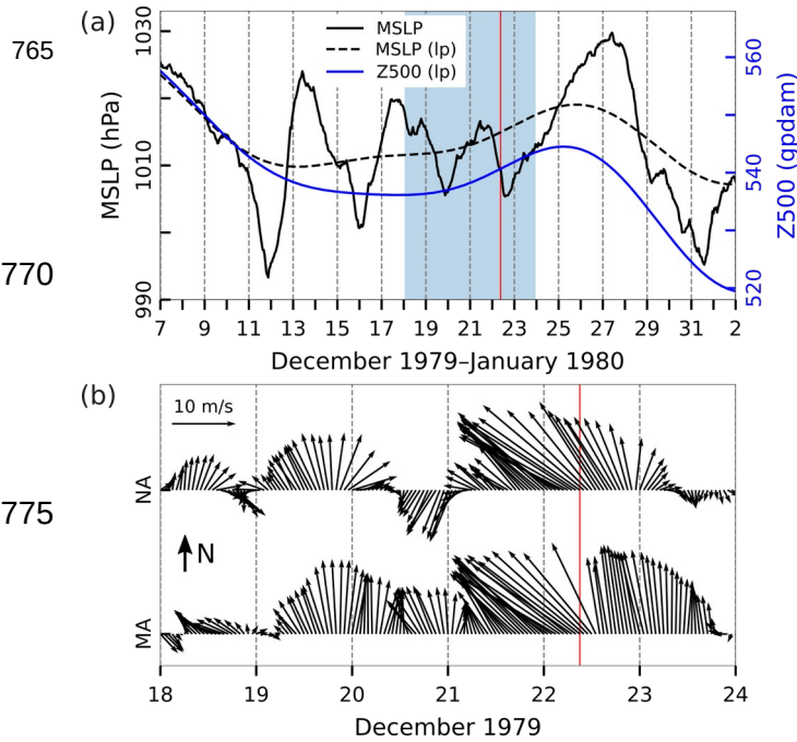
Figure 21: Series of ERA5 reanalysis data related to the flood of 22 December 1979. (a) MSLP (hourly) and MSLP (lp) (low-pass filtered with a cut-off frequency of 10 d) and Z500 (lp) (low-pass filtered with a cut-off frequency of 10 d) at a grid point near TG Bakar. (b) Hourly W10 during the period marked in blue in the upper plot for the middle (MA) and northern (NA) Adriatic (all locations marked in Fig. 1). The red line indicates onset of SL maximum.
