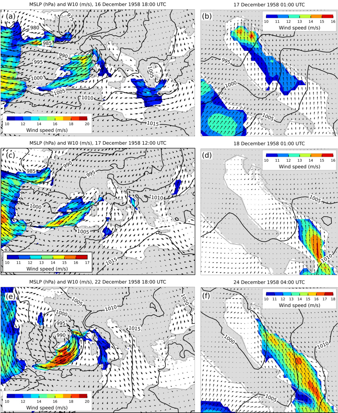
Figure 7: MSLP (black lines) and W10 (arrows and colours) fields from the ERA5 reanalysis. Conditions (a, c, e) over the Mediterranean that preceded the situations (b, d, f) over the Adriatic Sea (an hour before the SL maxima in Bakar). Only wind speeds exceeding 10 m/s are coloured.
