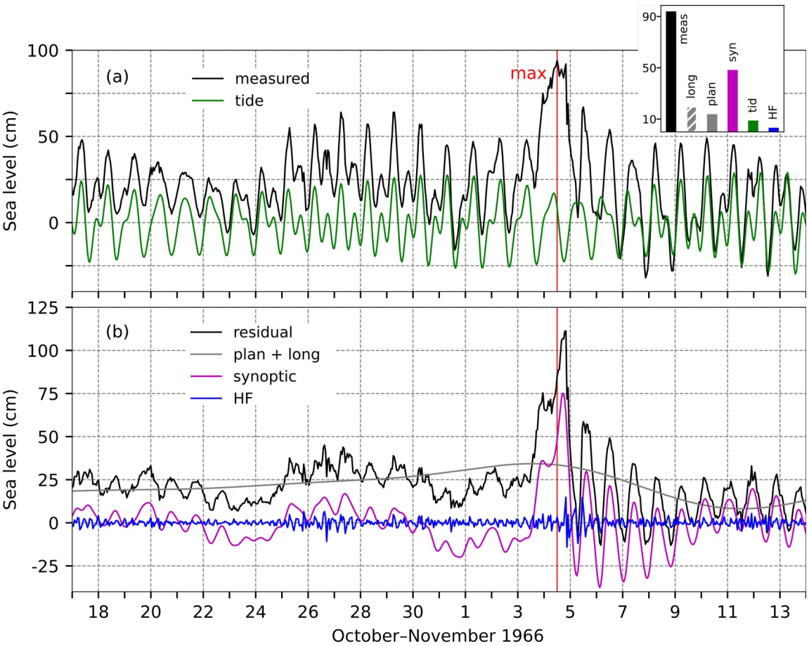
570 Figure 14: SL series for the flood of 4 November 1966. (a) Measured sea level (black) and tide (green). The inset figure shows the contributions (cm) of the five sea-level components to the maximum measured sea level ("meas"; 12:00 UTC): "HF" refers to high-frequency oscillations ( 2\text{ h} < T < 9\text{ h} ), "syn" to synoptic component ( 9\text{ h} < T < 10\text{ d} ), "tid" to tide , "plan" to planetary-scale variability ( 10\text{ d} < T < 100\text{ d} ), "long" to long-term sea-level variability ( 100\text{ d} < T ). (b) Residual sea level (black), the combined series of planetary-scale variability and long-term sea-level variability (grey; plan + long), synoptic component (purple), and high-frequency oscillations (blue). The red line indicates the time of occurrence of the total SL maximum.
