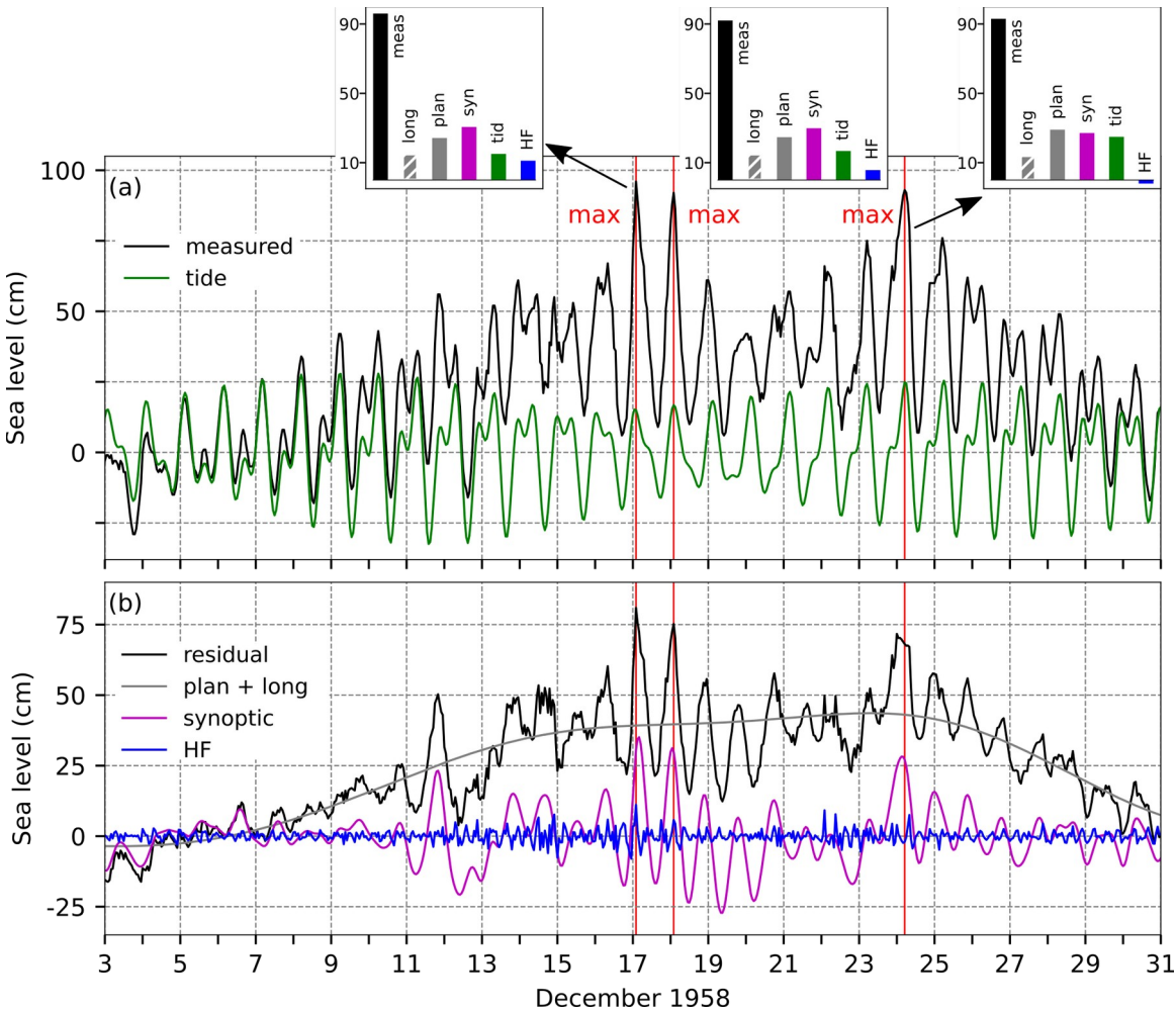
405 Figure 8: SL series for the floods 17, 18 and 24 December 1958. (a) Measured sea level (black) and tide (green). The inset figures show the contributions (cm) of the five sea-level components to the maximum measured sea levels ("meas"; left: 17 December 1958 02:00 UTC, middle: 18 December 1958 02:00 UTC, right: 24 December 1958 05:00 UTC): "HF" refers to high-frequency oscillations ( 2\text{ h} < T < 9\text{ h} ), "syn" to synoptic component ( 9\text{ h} < T < 10\text{ d} ), "tid" to tide , "plan" to planetary-scale variability ( 10\text{ d} < T < 100\text{ d} ), "long" to long-term 410 sea-level variability ( 100\text{ d} < T ). (b) Residual sea level (black), the combined series of planetary-scale variability and long-term sea-level variability (grey; plan + long), synoptic component (purple), and high-frequency oscillations (blue). The red lines indicate the times of
