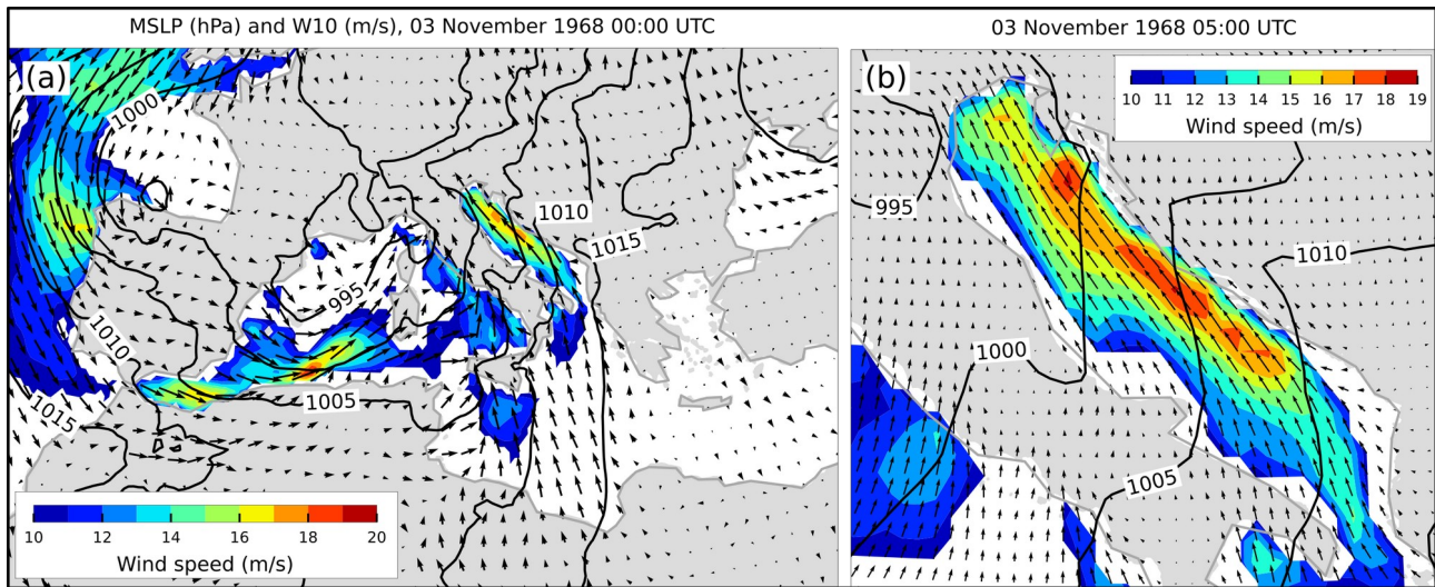
635 Figure 16: MSLP (black lines) and W10 (arrows and colours) fields from the ERA5 reanalysis. Conditions (a) over the Mediterranean that preceded the situation (b) over the Adriatic Sea (an hour before maximum SL in Bakar). Only wind speeds exceeding 10 m/s are coloured.
