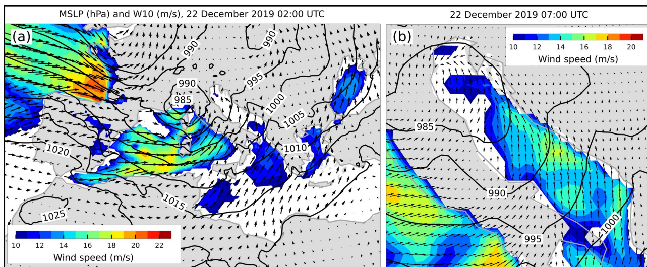
1845 Figure 61: MSLP (black lines) and W10 (arrows and colours) fields from the ERA5 reanalysis. Conditions (a) over the Mediterranean 1850 depicting a cyclone over the Gulf of Genoa that preceded the situation (b) over the Adriatic Sea (22 h before the flood). Only wind speeds exceeding 10 m/s are coloured.
