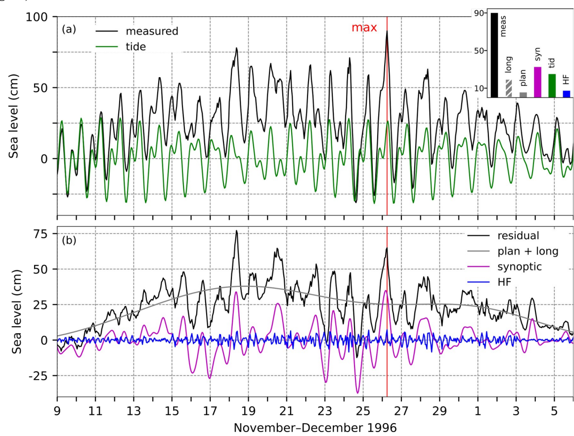
Figure 41: SL series for the flood of 26 November 1996. (a) Measured sea level (black) and tide (green). The inset figure shows the contributions (cm) of the five sea-level components to the maximum measured sea level ("meas"; 06:00 UTC): "HF" refers to high-frequency oscillations ( 2\text{ h} < T < 9\text{ h} ), "syn" to synoptic component ( 9\text{ h} < T < 10\text{ d} ), "tid" to tide , "plan" to planetary-scale variability ( 10\text{ d} < T < 100\text{ d} ), "long" to long-term sea-level variability ( 100\text{ d} < T ). (b) Residual sea level (black), the combined series of planetary-scale variability and long-term sea-level variability (grey; plan + long), synoptic component (purple), and high-frequency oscillations (blue). The red line indicates the time of occurrence of the total SL maximum.
