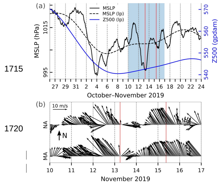
Figure 57: Series of ERA5 reanalysis data related to the floods of 13 and 15 November 2019. (a) MSLP (hourly) and MSLP (lp) (low-pass filtered with a cut-off frequency of 10 d) and Z500 (lp) (low-pass filtered with a cut-off frequency of 10 d) at a grid point near TG Bakar. (b) Hourly W10 during the period marked in blue in the upper plot for the middle (MA) and northern (NA) Adriatic (all locations marked in Fig. 1). The red lines indicate onset of SL maxima.
