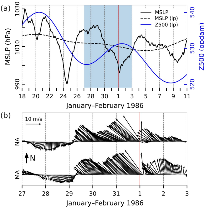
Figure 27: Series of ERA5 reanalysis data related to the flood of 1 February 1986. (a) MSLP (hourly) and MSLP (lp) (low-pass filtered with a cut-off frequency of 10 d) and Z500 (lp) (low-pass filtered with a cut-off frequency of 10 d) at a grid point near TG Bakar. (b) Hourly W10 during the period marked in blue in the upper plot for the middle (MA) and northern (NA) Adriatic (all locations marked in Fig. 1). The red line indicates onset of SL maximum.
