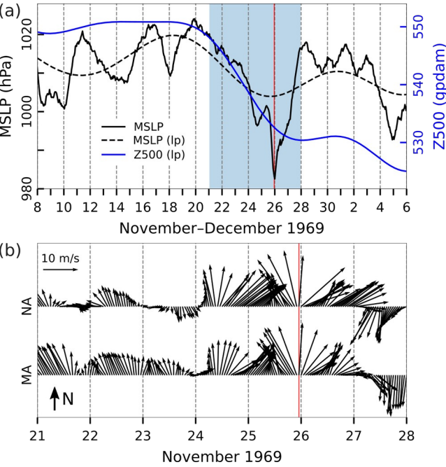
Figure 18: Series of ERA5 reanalysis data related to the flood of 25 November 1969. (a) MSLP (hourly) and MSLP (lp) (low-pass filtered with a cut-off frequency of 10 d) and Z500 (lp) (low-pass filtered with a cut-off frequency of 10 d) at a grid point near TG Bakar. (b) Hourly W10 during the period marked in blue in the upper plot for the middle (MA) and northern (NA) Adriatic (all locations marked in Fig. 1). The red line indicates onset of SL maximum.
