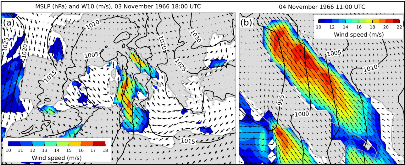
Figure 13: MSLP (black lines) and W10 (arrows and colours) fields from the ERA5 reanalysis. Conditions (a) over the Mediterranean that preceded the situation (b) over the Adriatic Sea (an hour before maximum SL in Bakar). Only wind speeds exceeding 10 m/s are coloured.
