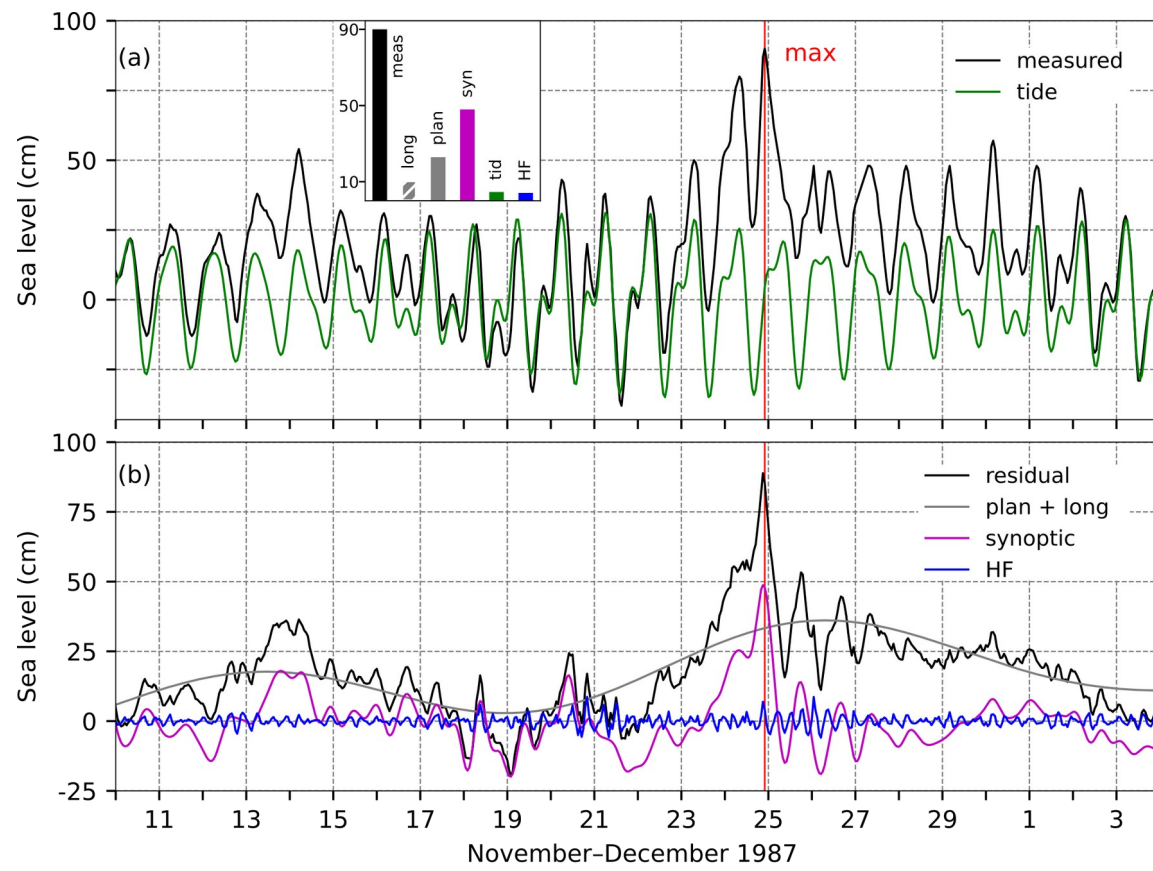
1050 Figure 32: SL series for the flood of 24 November 1987. (a) Measured sea level (black) and tide (green). The inset figure shows the contributions (cm) of the five sea-level components to the maximum measured sea level ("meas"; 22:00 UTC): "HF" refers to high-frequency oscillations ( 2\text{ h} < T < 9\text{ h} ), "syn" to synoptic component ( 9\text{ h} < T < 10\text{ d} ), "tid" to tide , "plan" to planetary-scale variability ( 10\text{ d} < T < 100\text{ d} ), "long" to long-term sea-level variability ( 100\text{ d} < T ). (b) Residual sea level (black), the combined series of planetary-scale variability and long-term sea-level variability (grey; plan + long), synoptic component (purple), and high-frequency oscillations (blue). The red line indicates the time of occurrence of the total SL maximum.
