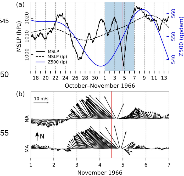
Figure 12: Series of ERA5 reanalysis data related to the flood of 4 November 1966. (a) MSLP (hourly) and MSLP (lp) (low-pass filtered with a cut-off frequency of 10 d) and Z500 (lp) (low-pass filtered with a cut-off frequency of 10 d) at a grid point near TG Bakar. (b) Hourly W10 during the period marked in blue in the upper plot for the middle (MA) and northern (NA) Adriatic (all locations marked in Fig. 1). The red line indicates onset of SL maximum.
