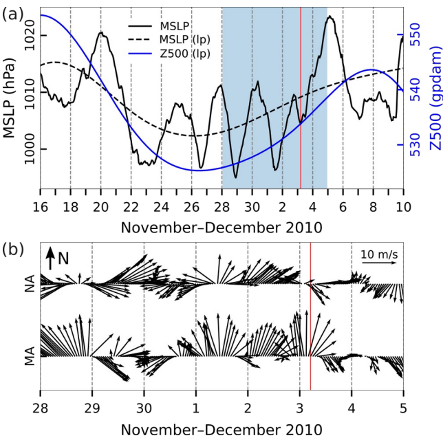
Figure 48: Series of ERA5 reanalysis data related to the flood of 3 December 2010. (a) MSLP (hourly) and MSLP (lp) (low-pass filtered with a cut-off frequency of 10 d) and Z500 (lp) (low-pass filtered with a cut-off frequency of 10 d) at a grid point near TG Bakar. (b) Hourly W10 during the period marked in blue in the upper plot for the middle (MA) and northern (NA) Adriatic (all locations marked in Fig. 1). The red line indicates onset of SL maximum.
