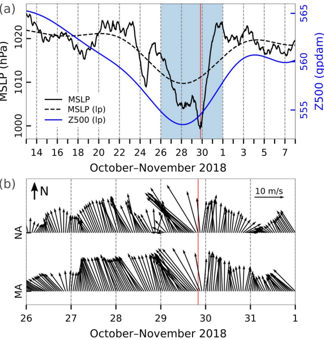
Figure 54: Series of ERA5 reanalysis data related to the flood of 29 October 2018. (a) MSLP (hourly) and MSLP (lp) (low-pass filtered with a cut-off frequency of 10 d) and Z500 (lp) (low-pass filtered with a cut-off frequency of 10 d) at a grid point near TG Bakar. (b) Hourly W10 during the period marked in blue in the upper plot for the middle (MA) and northern (NA) Adriatic (all locations marked in Fig. 1). The red line indicates onset of SL maximum.
