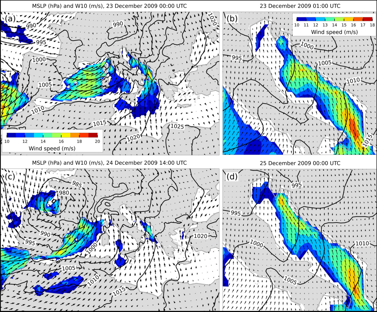
Figure 46: MSLP (black lines) and W10 (arrows and colours) fields from the ERA5 reanalysis. Conditions (a, c) over the Mediterranean that preceded the situations (b, d) over the Adriatic Sea (an hour before maxima SL in Bakar). Only wind speeds exceeding 10 m/s are coloured. The left colourbar is for the Mediterranean and the right one is for the Adriatic.
