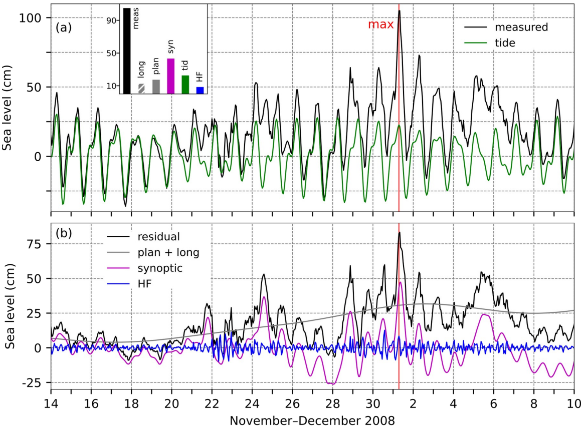
Figure 44: SL series for the flood of 1 December 2008. (a) Measured sea level (black) and tide (green). The inset figure shows the contributions (cm) of the five sea-level components to the maximum measured sea level ("meas"; 07:00 UTC): "HF" refers to high-frequency oscillations ( 2\text{ h} < T < 9\text{ h} ), "syn" to synoptic component ( 9\text{ h} < T < 10\text{ d} ), "tid" to tide , "plan" to planetary-scale variability ( 10\text{ d} < T < 100\text{ d} ), "long" to long-term sea-level variability ( 100\text{ d} < T ). (b) Residual sea level (black), the combined series of planetary-scale variability and long-term sea-level variability (grey; plan + long), synoptic component (purple), and high-frequency oscillations (blue). The red line indicates the time of occurrence of the total SL maximum.
