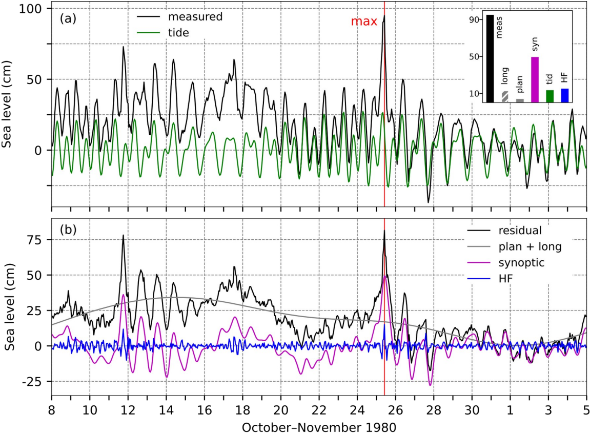
895 Figure 26: SL series for the flood of 25 October 1980. (a) Measured sea level (black) and tide (green). The inset figure shows the contributions (cm) of the five sea-level components to the maximum measured sea level ("meas"; 10:00 UTC): "HF" refers to high- frequency oscillations (2 h < T < 9 h), "syn" to synoptic component (9 h < T < 10 d), "tid" to tide , "plan" to planetary-scale variability (10 d < T < 100 d), "long" to long-term sea-level variability (100 d < T). (b) Residual sea level (black), the combined series of planetary-scale variability and long-term sea-level variability (grey; plan + long), synoptic component (purple), and high-frequency oscillations (blue). 900 The red line indicates the time of occurrence of the total SL maximum.
