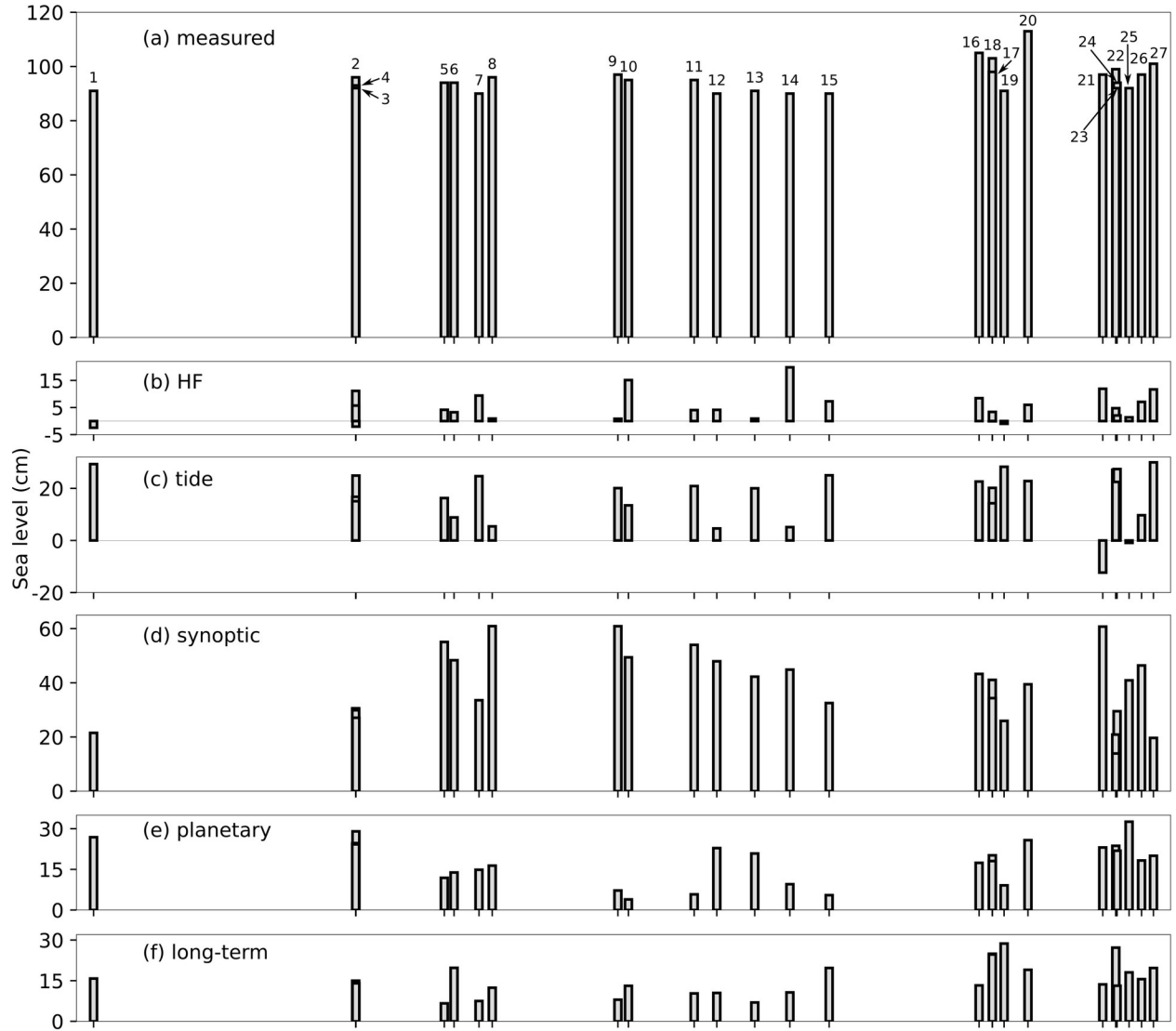
Figure 72: (a) Temporal distribution of total SL maxima observed in Bakar during the 27 extreme SL episodes (marked with their ID numbers from Table 2). Contributions of SL components to observed maxima: (b) high-frequency oscillations ( 2 \text{ h} < T < 9 \text{ h} ), (c) tide , (d) synoptic component ( 9 \text{ h} < T < 10 \text{ d} ), (e) planetary-scale component , ( 10 \text{ d} < T < 100 \text{ d} ), and (f) long-term sea-level variability ( 100 \text{ d} < T ).
