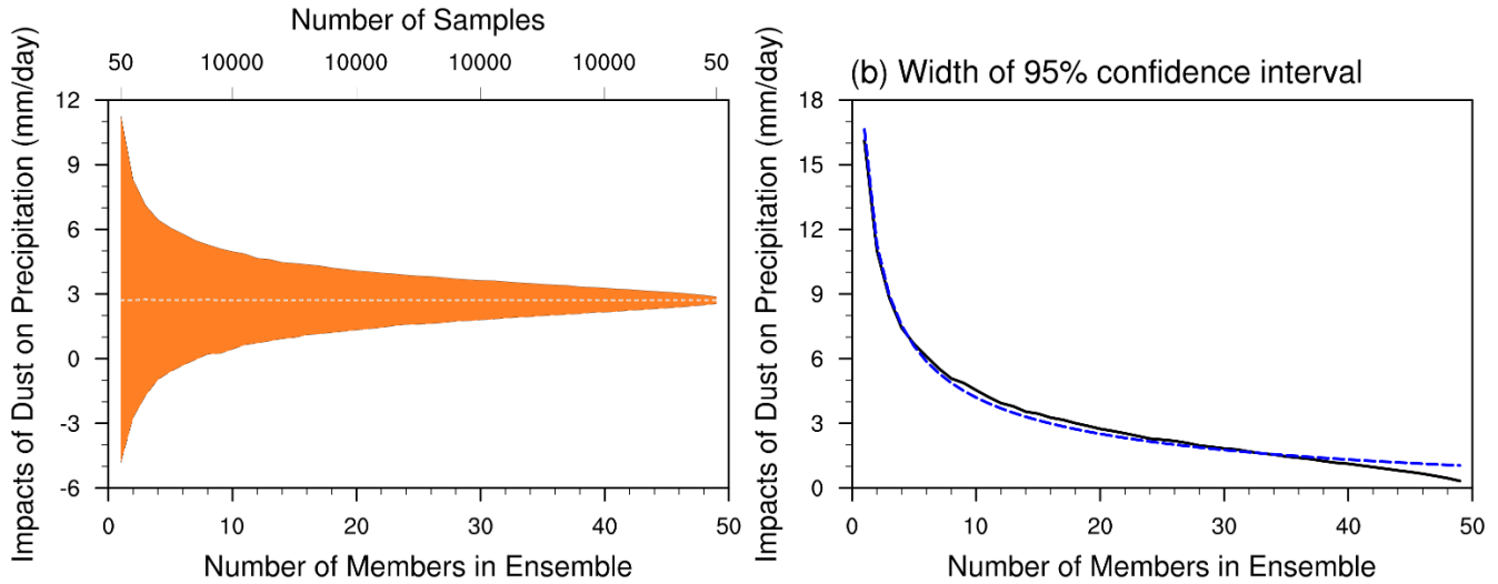
Figure 7: 95% confidence interval of regional average precipitation difference. The vertical axis represents the difference in average precipitation between the control experiment and the sensitivity experiment within the monsoon depression area. The definition of the 95% confidence interval is the range between the 97.5th percentile and the 2.5th percentile of the sample. (a) Shows the 95% confidence interval, with the black dashed line representing the average precipitation difference of 50 experiments, and the white dashed line representing the average value for each number of members in ensemble. (b) The black solid line in the figure shows how the width of the 95% confidence interval varies with number of members in ensemble, and the blue dashed line represents the logarithmic fitting curve, with the fitting expression being 18.18N^{-\frac{1}{2}} - 1.55 .
