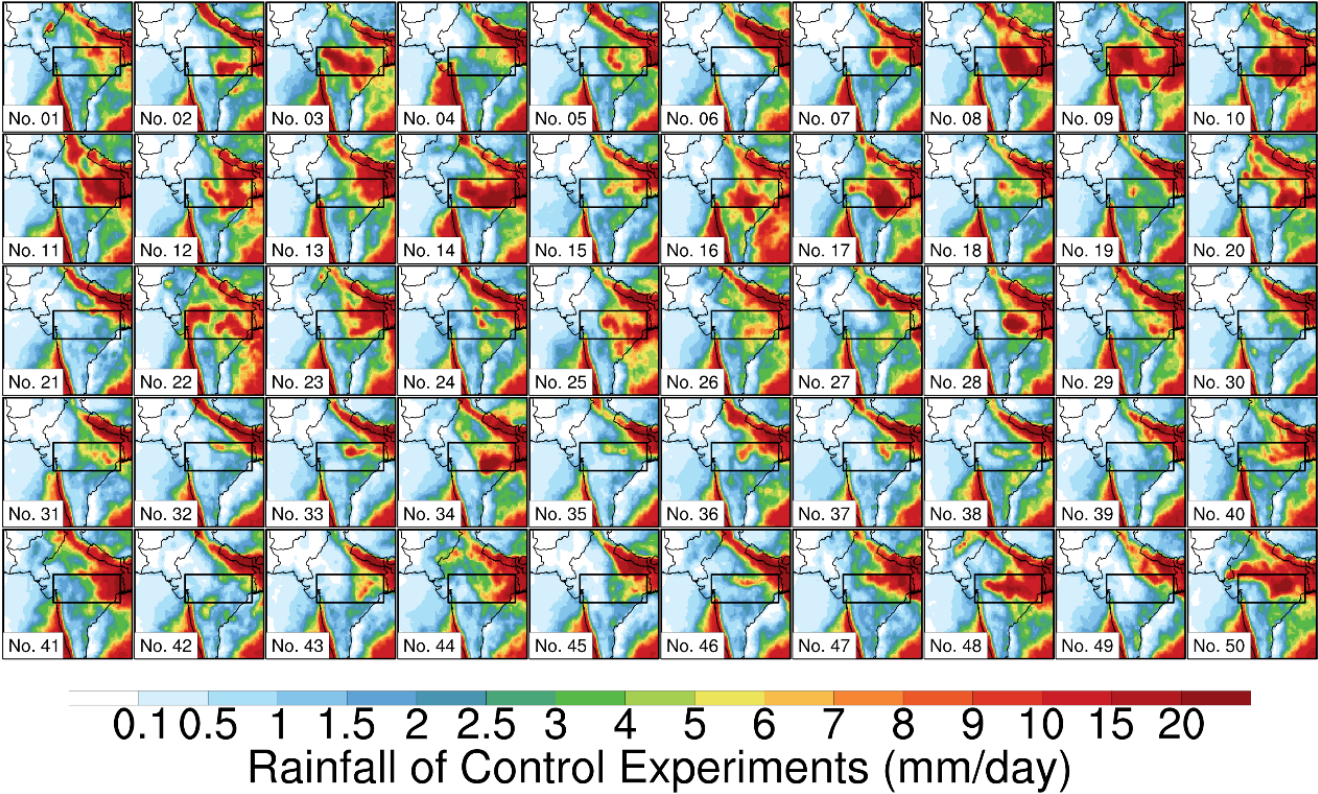
Figure 2: The spatial distributions of precipitation derived from 50 ensemble members of “Control” experiments over the Indian monsoon region. The results are averaged from June 10, 2016, to June 30, 2016. The monsoon depression region is delineated by the black box.
