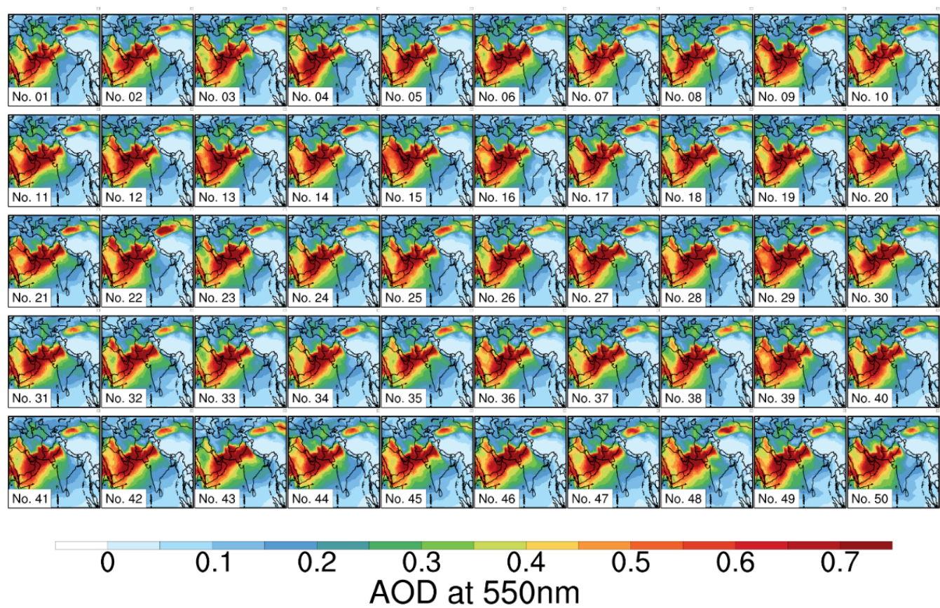
315 Figure 4: Same as Fig. 2 but for AOD at 550nm of “Control” experiments.
