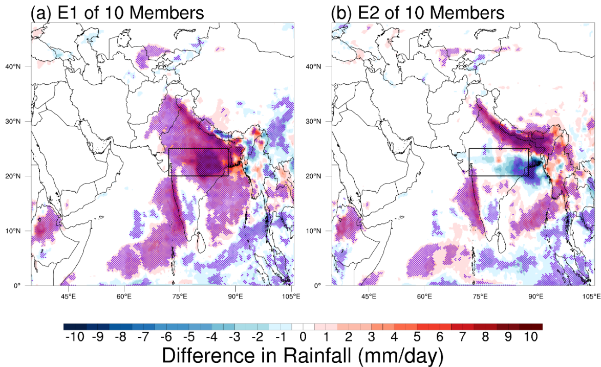
465 Figure 9: 95% significance test (Student's t-test) results for two extreme cases selected from 10,000 possible combinations of 10-member ensembles, representing the maximum (panel a) and minimum (panel b) area-averaged responses.
