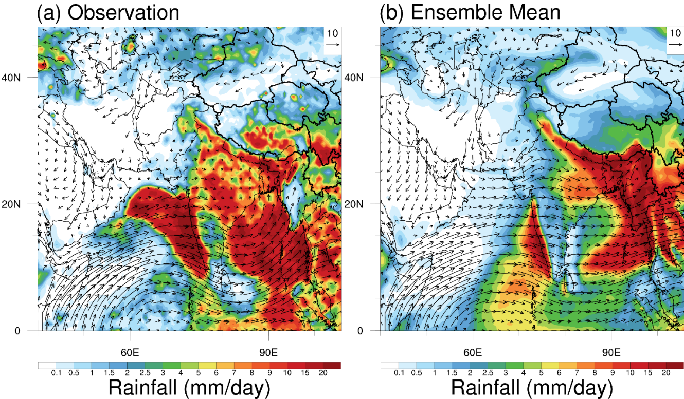
270 Figure 1: The observations and simulations of monsoon circulation (wind field at 850hPa) and precipitation, averaged from June 10, 2016, to June 30, 2016. The observed wind field at 850hPa derived from ERA5 and the observed rainfall is from CMORPH. The simulation results are shown as 50-member ensemble mean.
