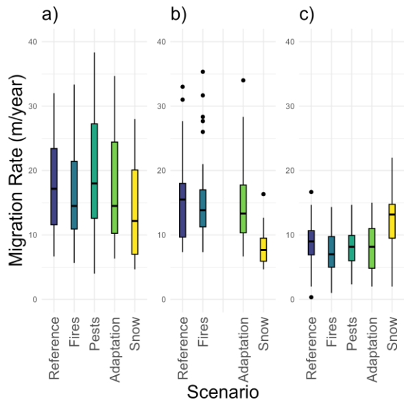
405 Figure 6: Box plots showing migration rates from 40 simulation runs at three study sites: a) Fort McPherson, Canada (CA), b) Lake Ilirney, Russia (RU), and c) Road to Central, Alaska, USA (AK). Each panel compares the reference scenario with four scenarios in which specific environmental modules were activated. Note that for the Russian study site, the insect disturbance module was not implemented in LAVESI.
