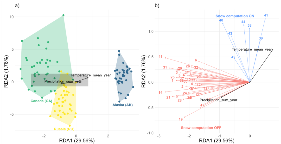
450 Figure 8: Redundancy Analysis (RDA) biplot showing a) site scores and b) species scores along the first two principal axes. Plot b provides a close-up of the centre region (grey rectangle) of plot a to highlight tightly grouped species. Site scores (migration rates) are represented by points, colour-coded according to their study site. Species scores (simulation scenarios) are depicted as arrows, colour-coded to indicate whether snow computation is activated (blue: Snow computation ON) or not (red: Snow computation OFF). Black arrows in both plots represent the direction and strength of environmental variables influencing migration rates.
