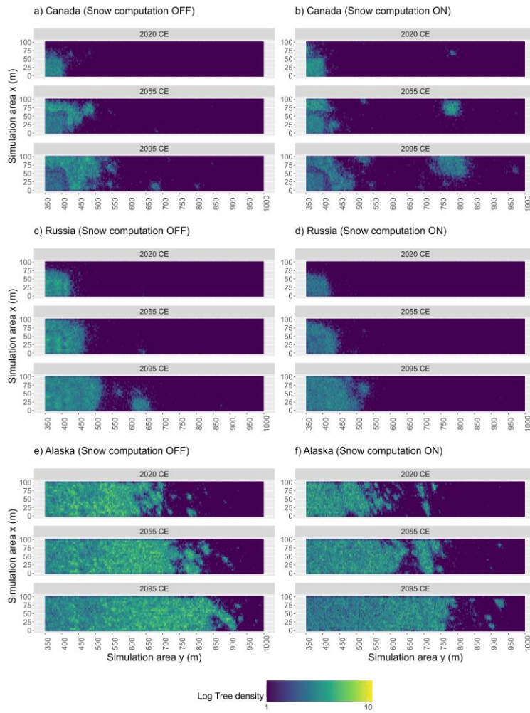
Figure 7: Tree density over time. Tree density in 2020, 2055, and 2095 CE at study site Fort McPherson West, Canada (CA) under a) the reference scenario (run 34) and b) the scenario with activated snow computation (run 2). Tree density in 2020, 2055, and 2095 CE at study site Lake Ilirney, Russia (RU) under c) the reference scenario (run 13) and d) the scenario with activated snow computation (run 3). Tree density in 2020, 2055, and 2095 CE at study site Road to Central, Alaska, USA (AK) under e) the reference scenario (run 15) and f) the scenario with activated snow computation (run 3). (Run with the median migration rate calculated from 40 runs for each simulation scenario). Each plot represents data from the simulation run with the median migration rate derived from 40 simulation runs per scenario. Tree density values (dimensionless units) were log-transformed to enhance data visualisation.
