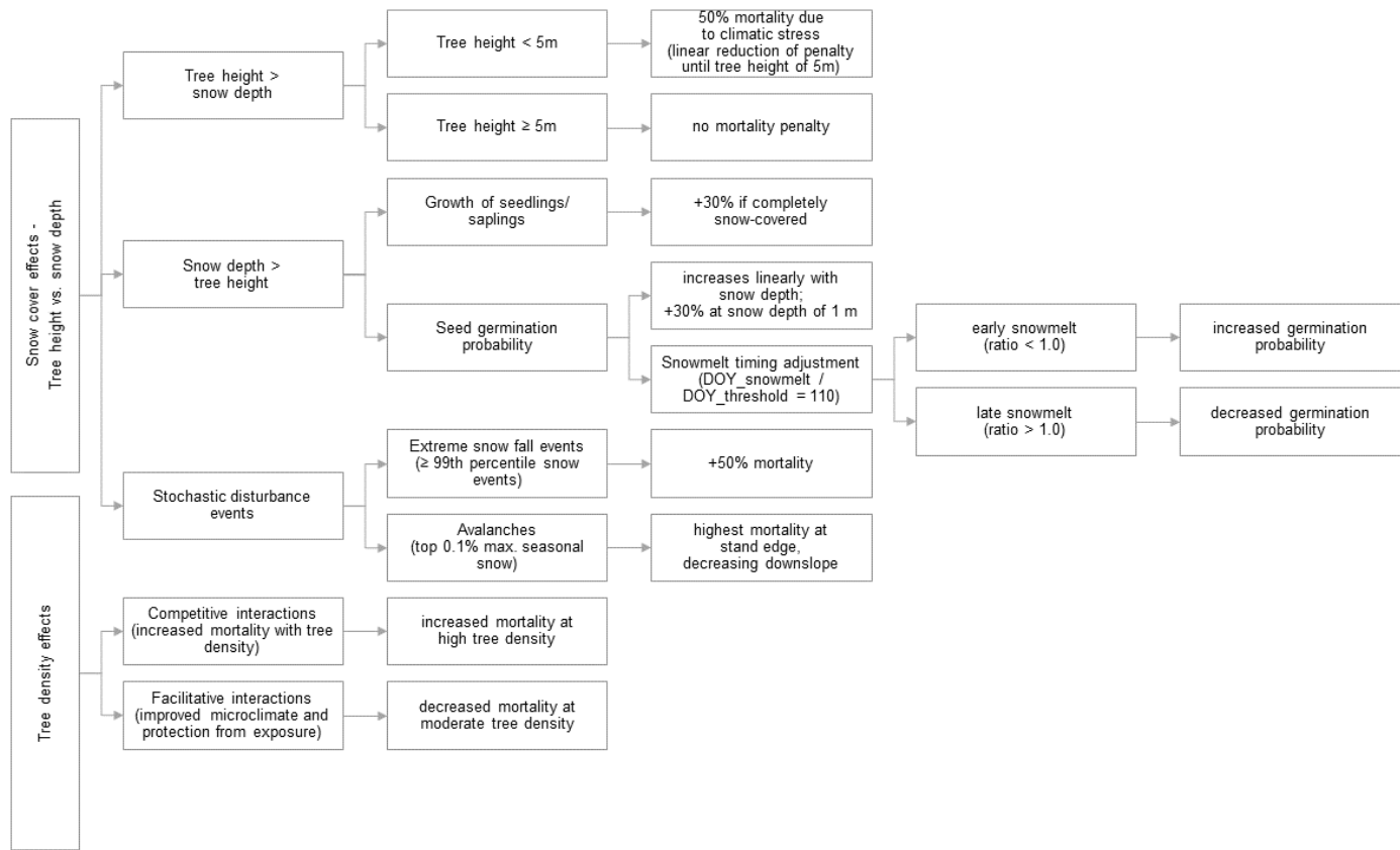
200 Figure 2: Flowchart illustrating snow-related processes influencing alpine treeline migration, as implemented in the snow module of the vegetation model LAVESI ( Larix Vegetation Simulator).
