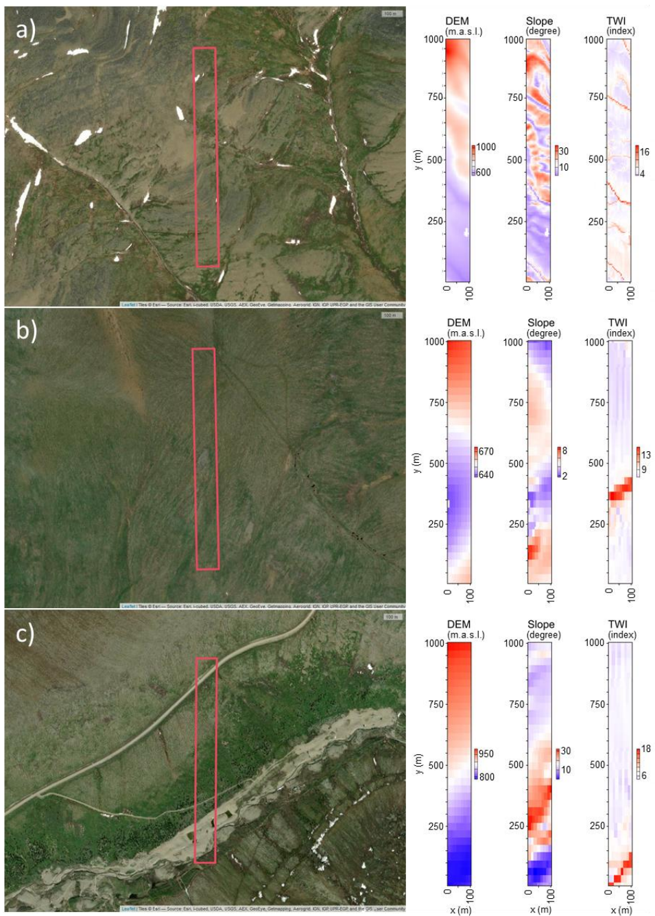
Figure 5: Satellite images of the study sites: a) Fort McPherson, Canada (CA), b) Lake Ilirney, Russia (RU), and c) Road to Central, Alaska/ USA (AK), including the simulation area (red box). Digital elevation model (DEM), slope, and topographic wetness index (TWI) for the simulation area. Esri, i-cubed, USDA, USGS, AEX, Geoeeye, Getmapping, Aerogrid, IGN, IGP, UPR-EGP, and the GIS User Community.
