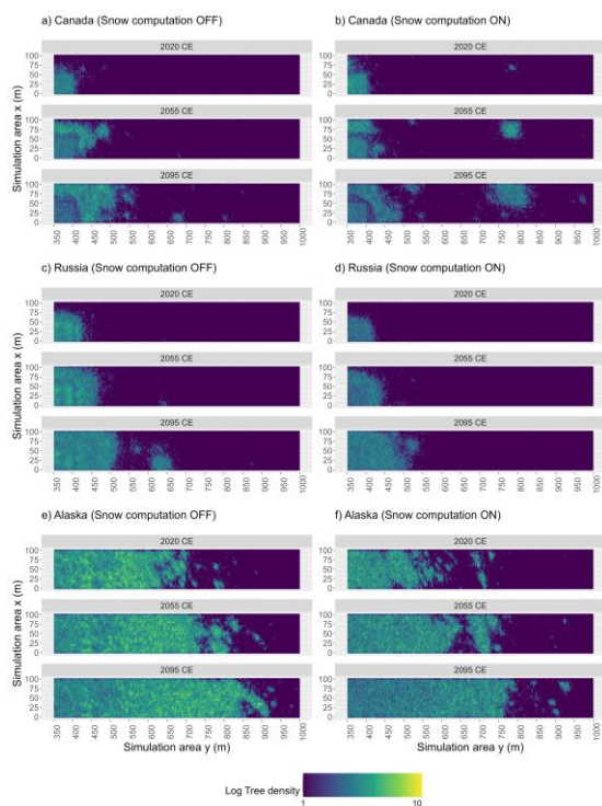
Figure 79: Tree density over time. Tree density in 2020, 2055, and 2095 CE at study site Fort McPherson West, Canada (CA) under a) the reference scenario (run 34) and b) the scenario with activated snow computation (run 2). Tree density in 2020, 2055, and 2095 CE at study site Lake Ilirney, Russia (RU) under c) the reference scenario (run 13) and d) the scenario with activated snow computation (run 3). Tree density in 2020, 2055, and 2095 CE at study site Road to Central, Alaska, USA (AK) under e) the reference scenario (run 15) and f) the scenario with activated snow computation (run 3). (Run with the median migration rate calculated from 40 simulation runs per scenario). Each plot represents data from the simulation run with the median migration rate derived from 40 simulation runs per scenario. Tree density values ( dimensionless units ) were log-transformed to enhance data visualisation.
