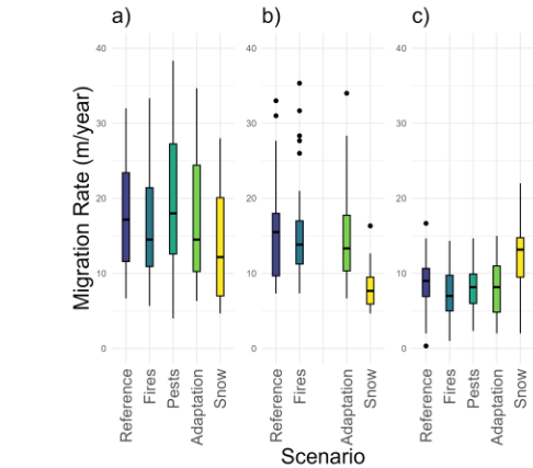
Figure 68: Box plots showing migration rates from 40 simulation runs at three study sites: a) Fort McPherson, Canada (CA), b) Lake Ilirney, Russia (RU), and c) Road to Central, Alaska, USA (AK). Each panel compares the reference scenario with four scenarios in which specific environmental modules were activated. Note that for the Russian study site, the insect disturbance module was not implemented in LAVESL.
